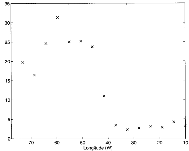
FIG. 4. Relative power in the north-south wavenumber spectrum of wind curl from COADS data (from Fig. 2); the mean of the two lowest wavenumbers is shown.
