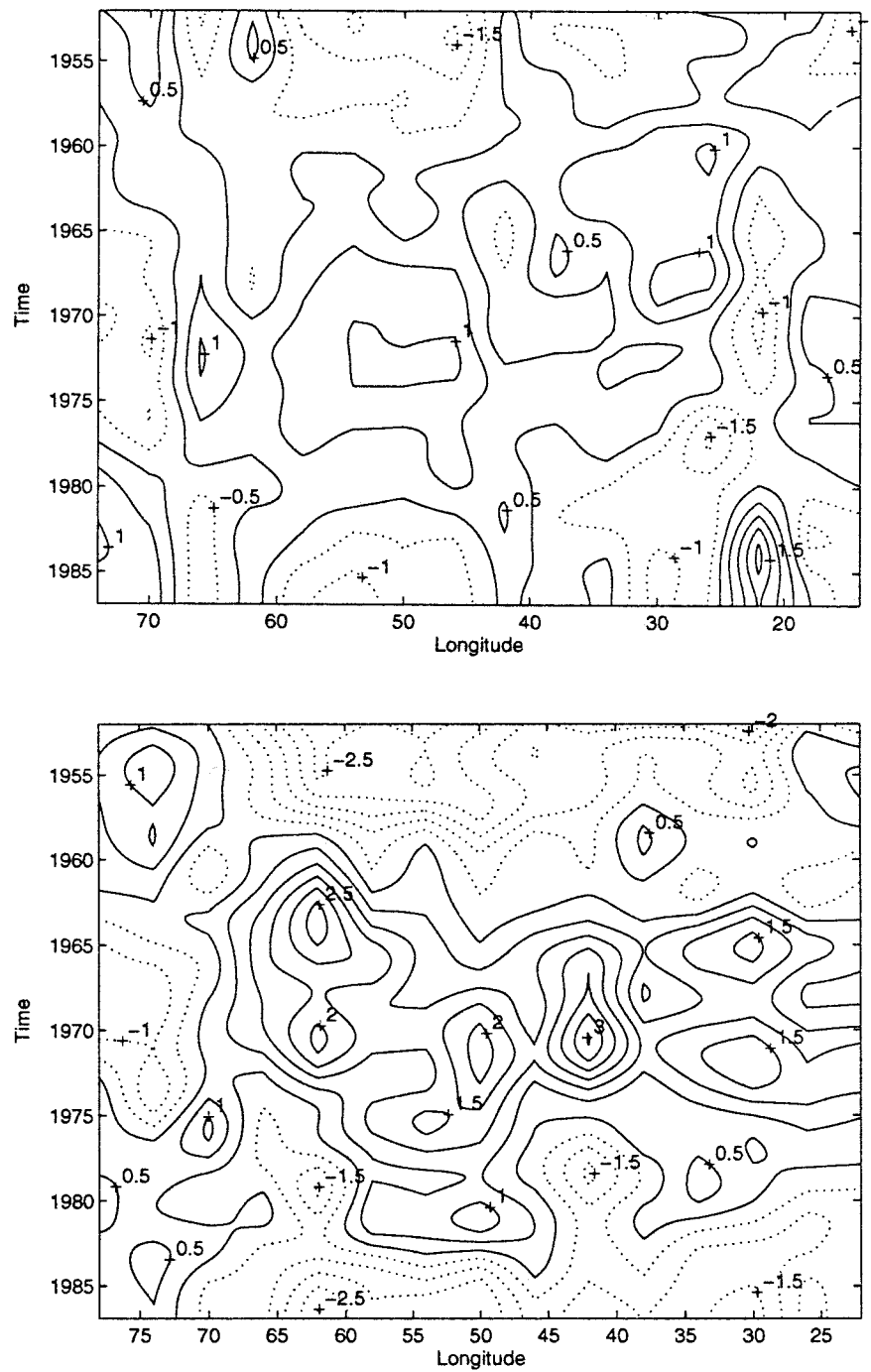
FIG. 5c,d. Computed fluctuations in the Ekman pumping across the Atlantic at 34°N (upper) and 18°N (lower), as a function of longitude and time, that are used to force the results shown in Figs. 5a,b.
