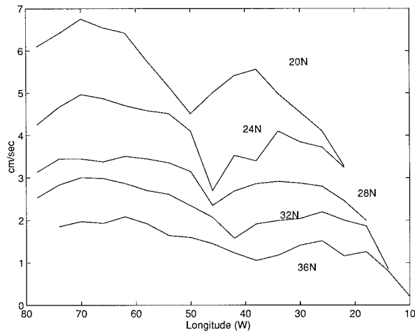
FIG. 2. Speeds of the long Rossby waves in the model. Only every other latitude band used is shown. The speeds were computed for the first vertical mode based on the data available from NODC in each 4° by 4° box (see text).
