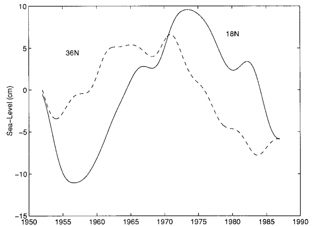
FIG. 9. Departures of model sea level along 70^{\circ}\text{W} for two latitudes: 18^{\circ}\text{N} (solid curve) and 36^{\circ}\text{N} (dashed). Time is in years.
