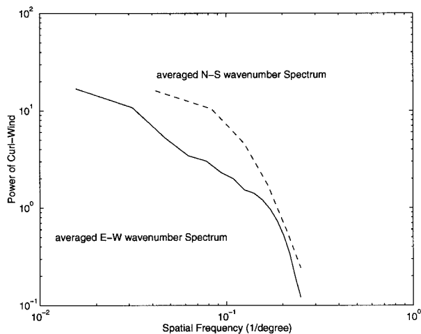
FIG. 3. Average wavenumber spectra of wind curl forcing based on COADS data. The east-west spectrum is averaged from 18° to 42°N across the width of the Atlantic. The calculation uses 2° resolution, but the wind stress was initially integrated around 4° boxes to compute the curl. For simplicity in plotting the east-west variability, the power is shown as if each degree of longitude were 100 km in length.
