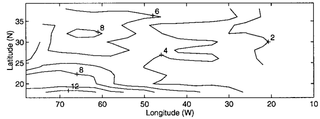
FIG. 6. The maximum absolute amplitude of the ocean's response in the model; amplitudes are in centimeters.
