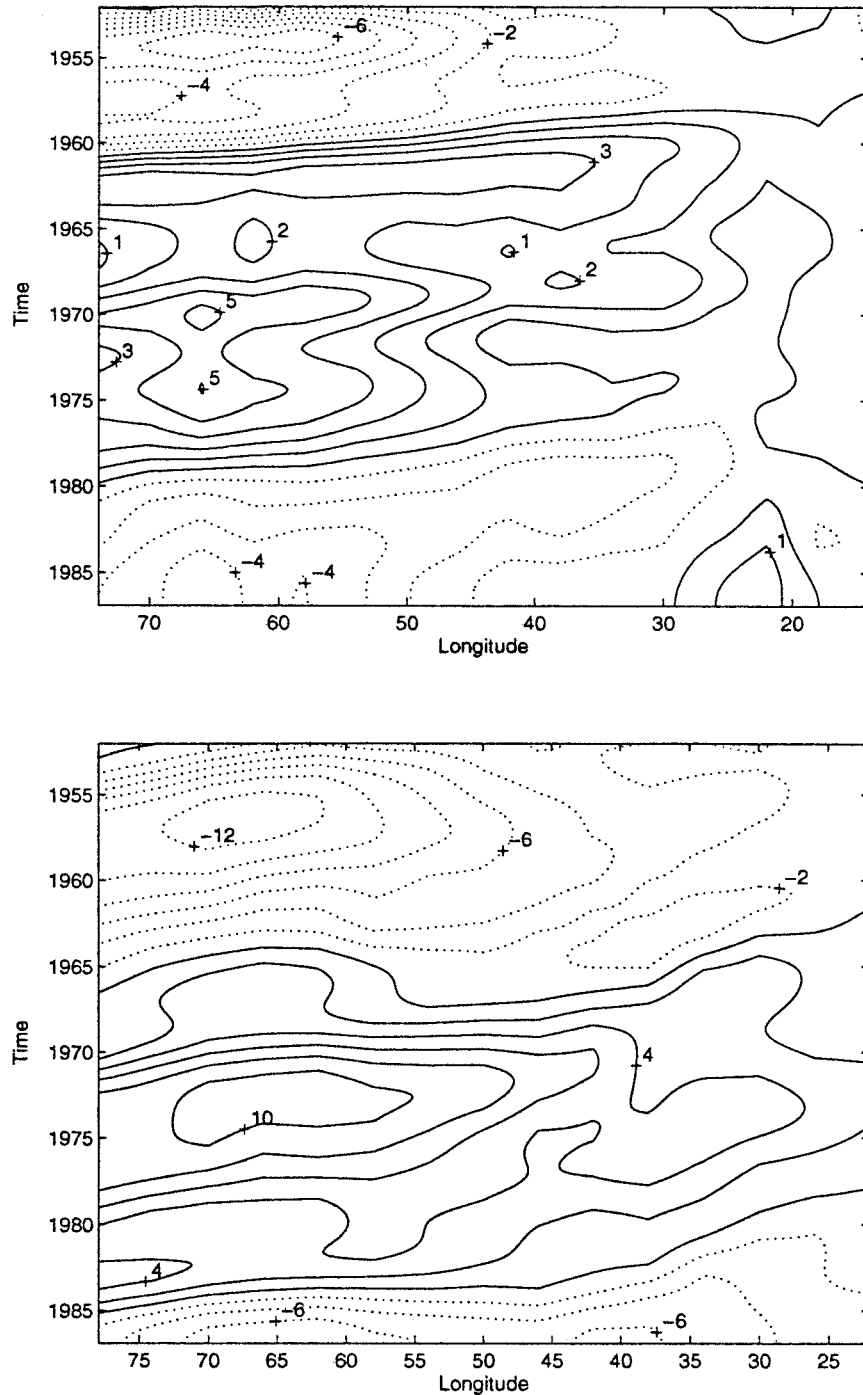
FIG. 5a,b. Computed fluctuations in the height of sea level across the Atlantic at 34°N (upper) and 18°N (lower) as a function of longitude and time. Heights are in centimeters.
