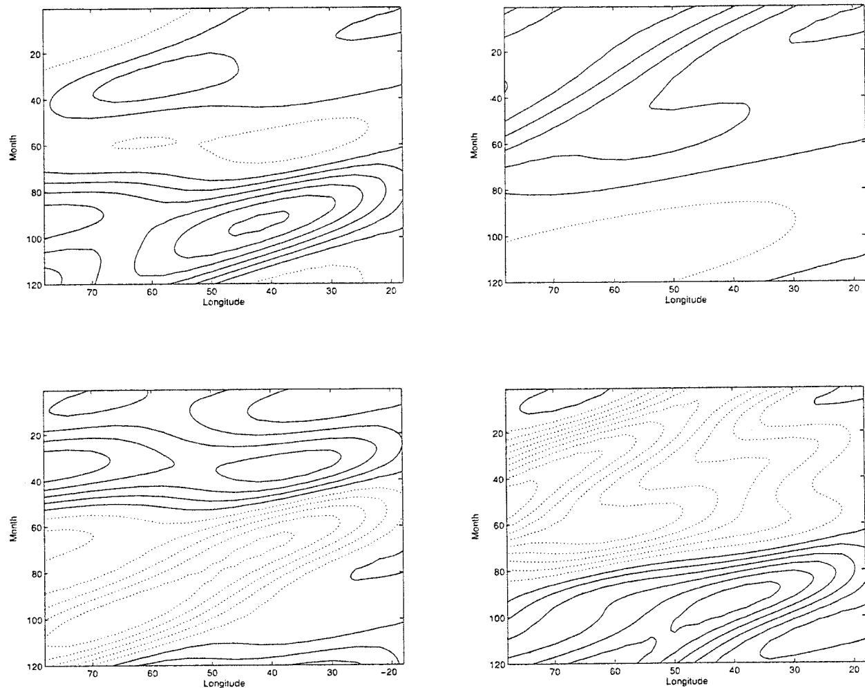
FIG. 10b–e. Examples of model output for a test case, as in Fig. 10a except that random noise has been added to the forcing. The noise amplitude is a factor of 20 times that of the cosine wave. Solid contours represent positive sea surface displacement; amplitudes are arbitrary. The speed doubling is no longer apparent.
