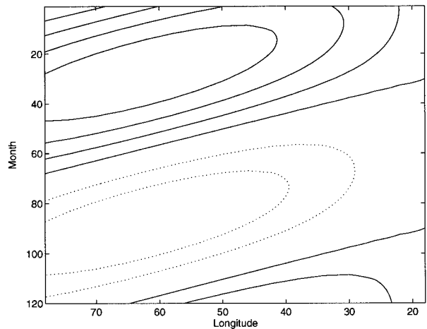
FIG. 10a. Model output for a test case; forcing is by a single cosine wave, uniform in x , a period of 120 months, with wave speed set at a constant 3 \text{ cm s}^{-1} . The apparent propagation is twice the free wave speed, and there is a maximum in the western ocean. See text.
