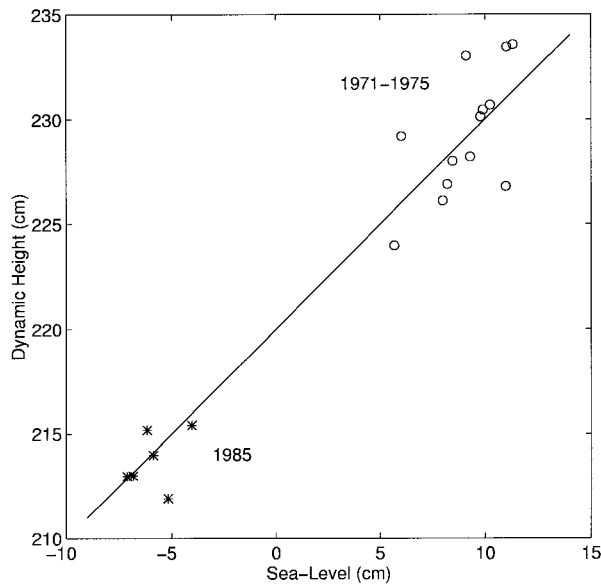
FIG. 7. Comparison between model output and dynamic height, 100–1000 db, from all hydrographic data during time intervals of large departures (as determined from Fig. 5b), using the times and positions of the available data to extract model output.
