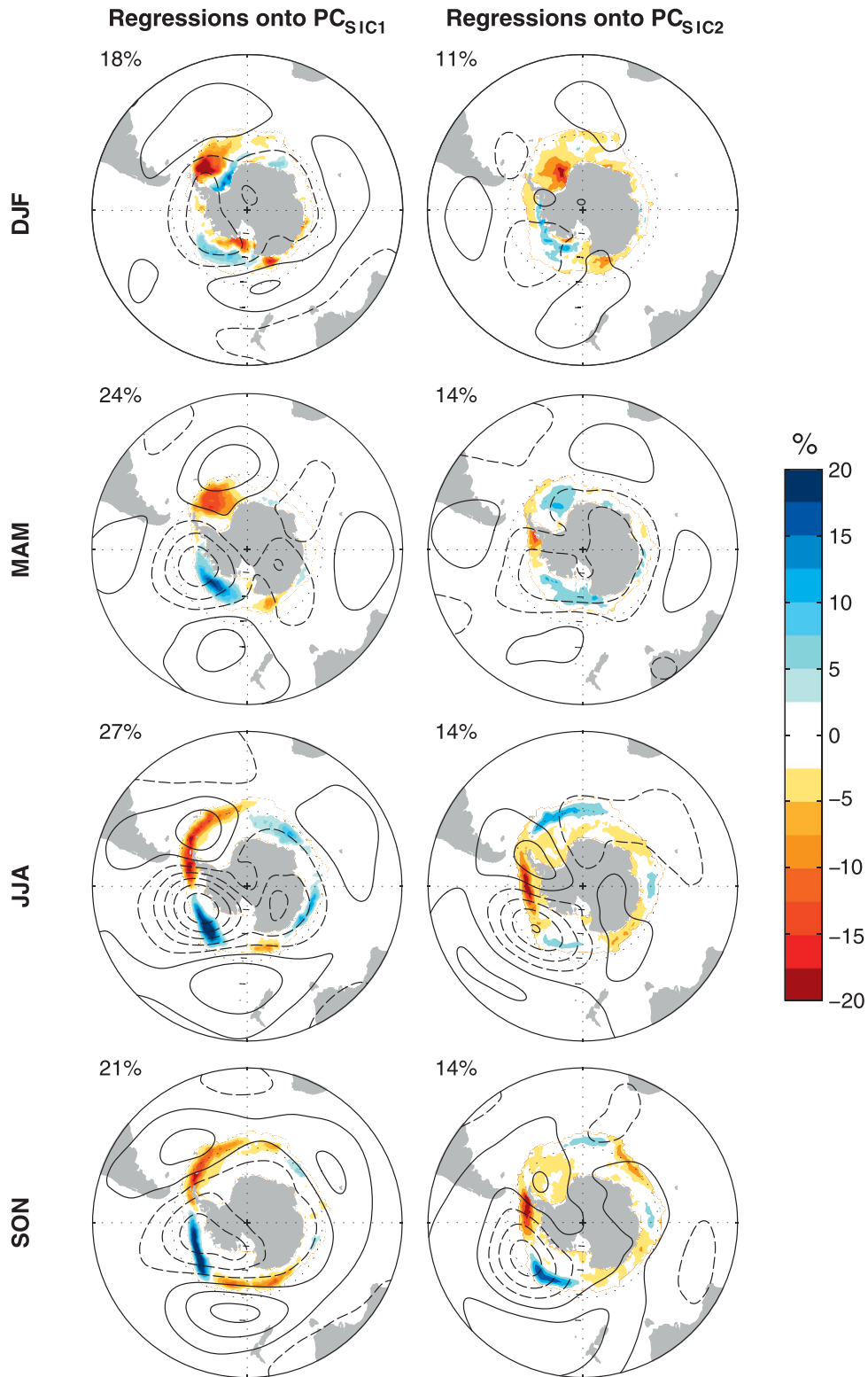
FIG. 4. As in Fig. 3 but for Z_{500} (contours) and SIC (shading) anomalies regressed onto standardized (left) PC SIC1 and (right) PC SIC2 . The value (top-left above each panel) describes the percentage variance explained by each mode.
