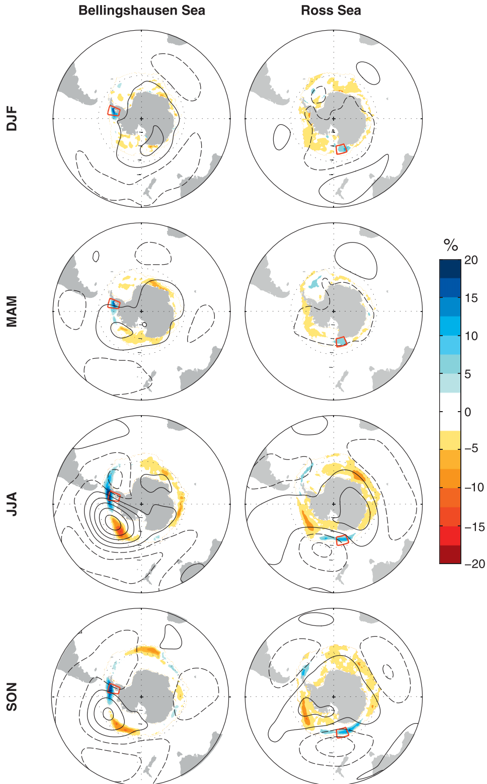
FIG. 11. As in Fig. 3 but for Z_{500} (contours) and SIC (shading) anomalies regressed onto standardized sea ice time series from the (left) Bellingshausen and (right) Ross Sea regions. Red squares define the spatial limit of the area used to create the sea ice time series and correspond to the black boxes of Fig. 8. Note that the Ross Sea box moves equatorward during JJA and SON.
