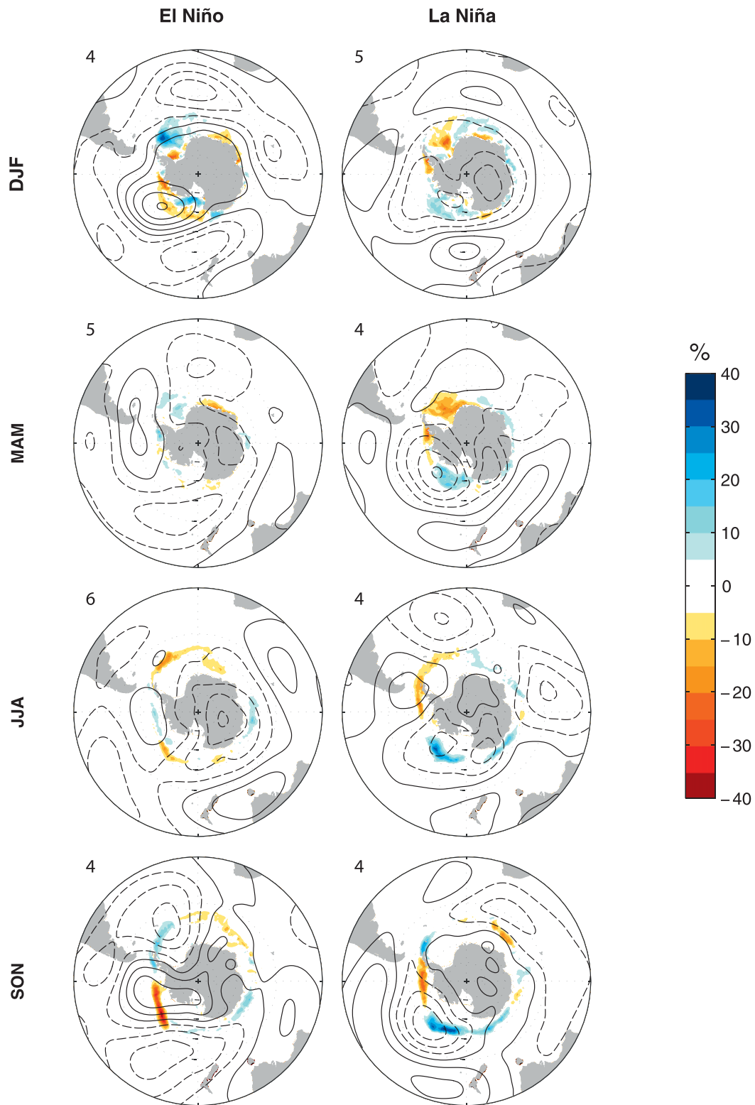
FIG. 7. (left) El Niño and (right) La Niña composites of seasonal-mean Z_{500} (contours) and SIC (shading) anomalies averaged over seasons wherein the cold tongue ENSO index exceeds one standard deviation. Positive (negative) contours are denoted by solid (dashed) lines drawn at intervals of 15 m ( -22.5, -7.5, 7.5, 22.5 m...). The value (top-left above each panel) indicates the number of seasons used to create the composite.
