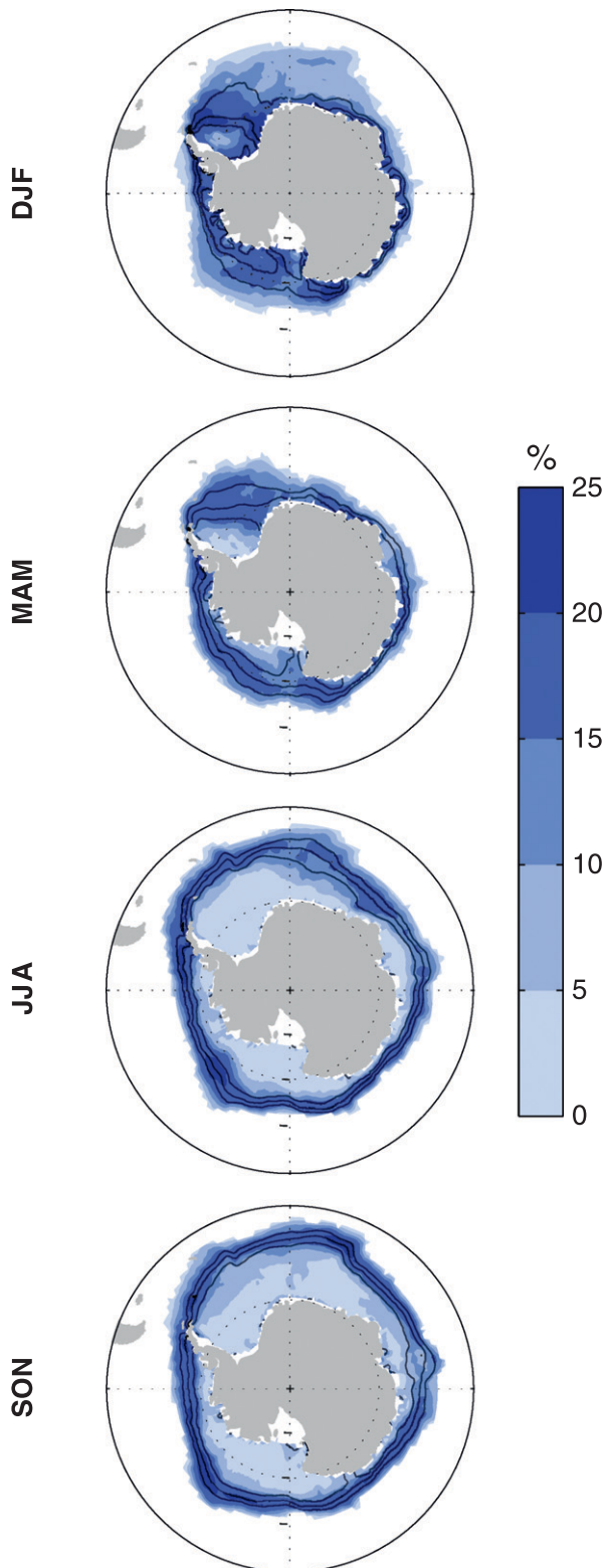
FIG. 2. Climatological mean (contours) and standard deviation (shading) of sea ice concentration (SIC) anomalies for (first row) DJF, (second row) MAM, (third row) JJA, and (fourth row) SON. Contours of the mean SIC are drawn at 25% intervals, with the 0% contour excluded.
