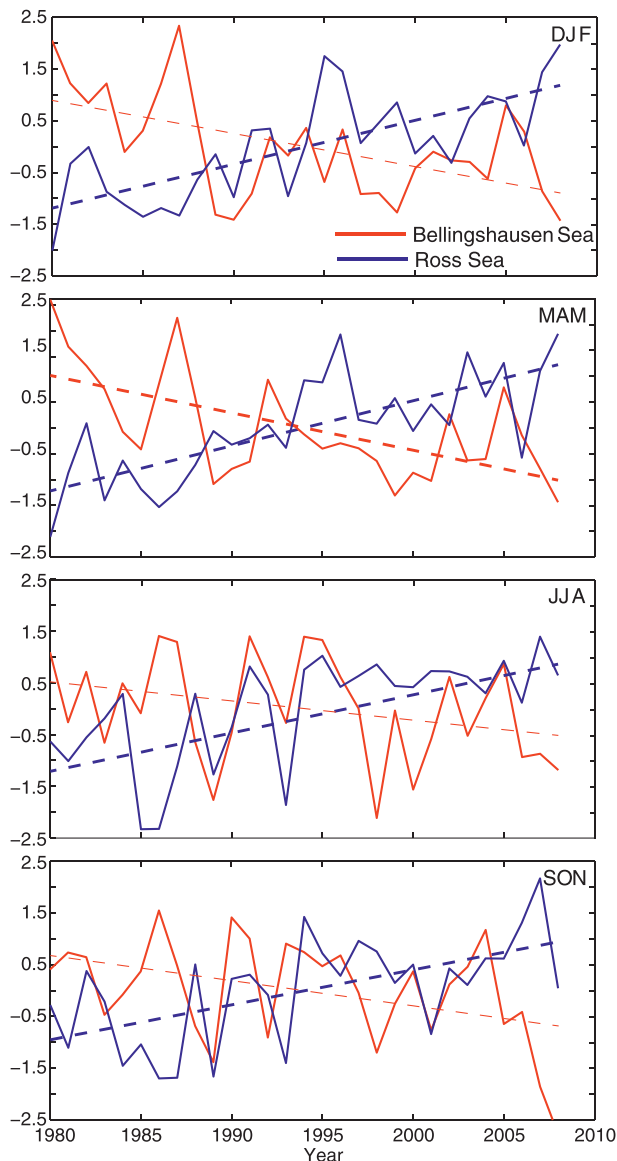
FIG. 10. Standardized seasonal-mean Bellingshausen Sea (red) and Ross Sea (blue) sea ice time series for (first row) DJF, (second row) MAM, (third row) JJA, and (fourth row) SON. Dashed lines represent the line of best fit with thick lines denoting statistically significant trends, as quantified in Table 2. Time series correspond to the average SIC over the region defined by black boxes shown in Fig. 8.
