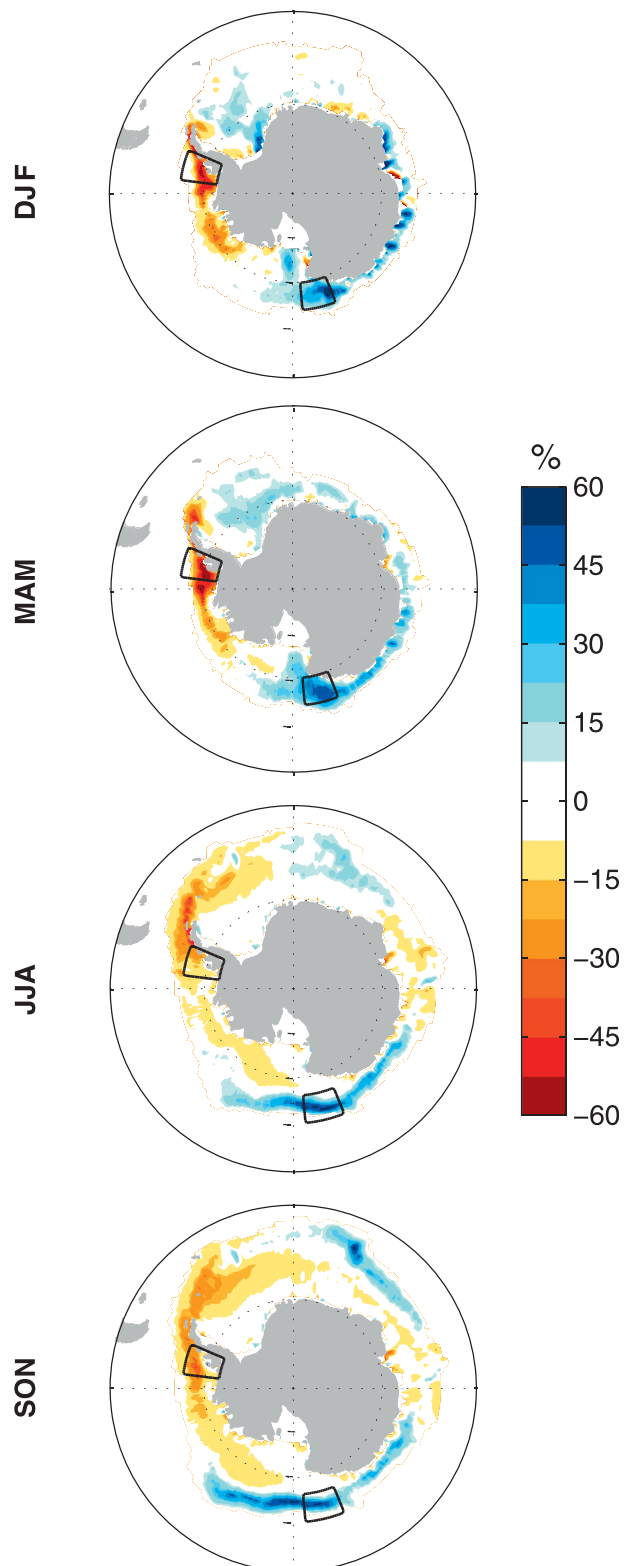
FIG. 8. Linear trends in seasonal-mean SIC calculated over 1980–2008 for (first row) DJF, (second row) MAM, (third row) JJA, and (fourth row) SON. Black boxes define the areas used to calculate regional sea ice time series (Fig. 10).
