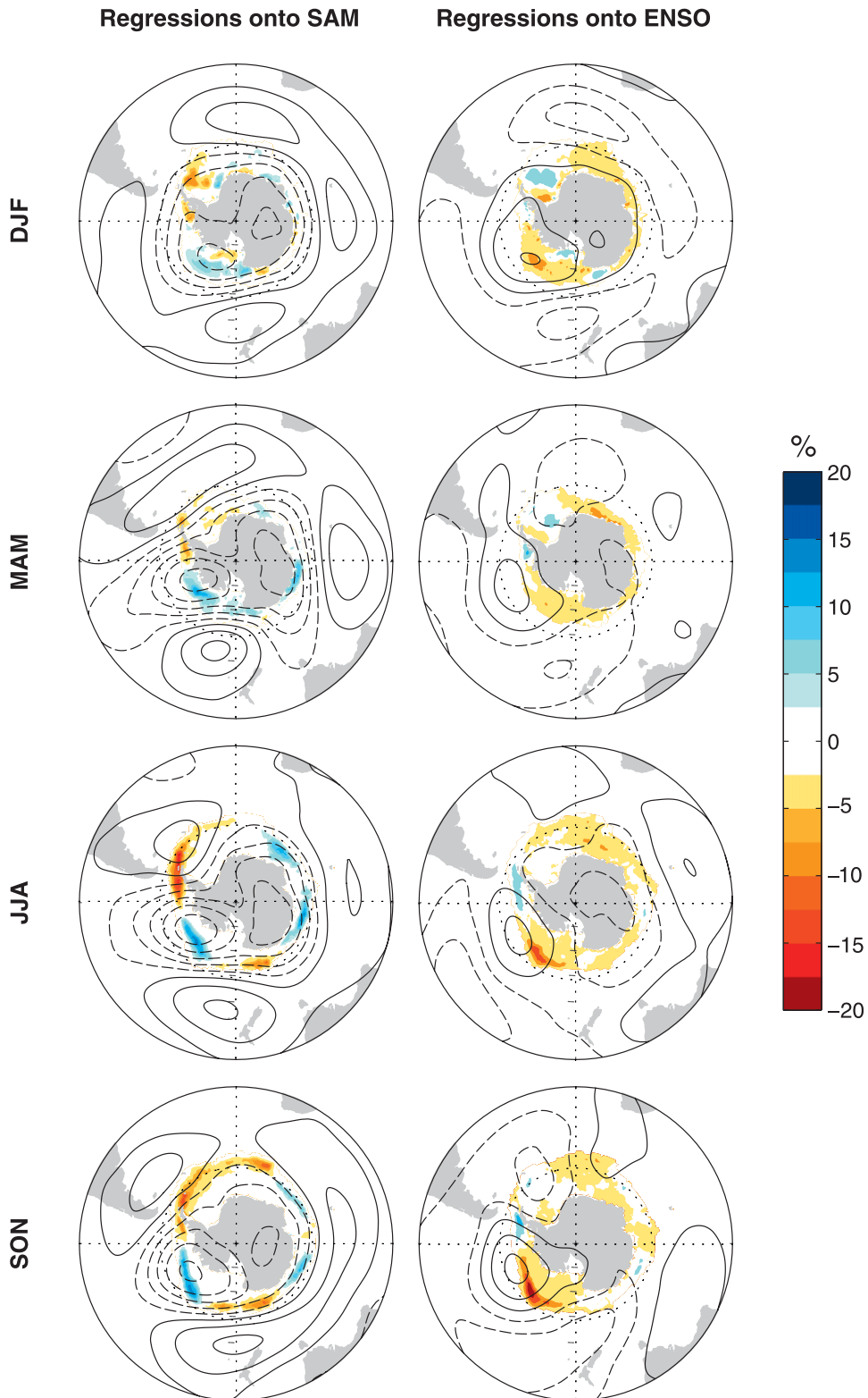
FIG. 3. Seasonal-mean Z_{500} (contours) and SIC (shading) anomalies regressed onto standardized (left) SAM and (right) ENSO indices for (first row) DJF, (second row) MAM, (third row) JJA, and (fourth row) SON. Positive (negative) contours are denoted by solid (dashed) lines and are drawn at intervals of 10 m ( -15, -5, 5, 15 m...).
