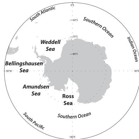
FIG. 1. Locations of the main Antarctic seas.
