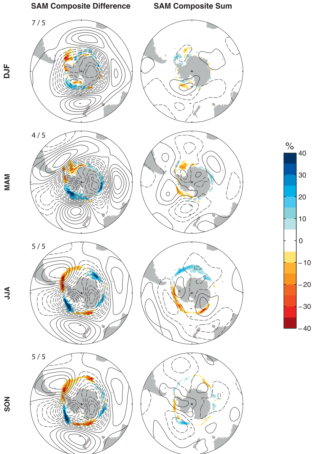
FIG. 5. (left) Composite differences and (right) composite sums of seasonal-mean Z_{500} (contours) and SIC (shading) anomalies averaged over seasons wherein the SAM index exceeds one standard deviation. Positive (negative) contours are denoted by solid (dashed) lines and are drawn at intervals of 15 m ( -22.5 , -7.5 , 7.5 , 22.5 m . . .). The values (top-left above the composite differences) indicate the number of positive/negative seasons, respectively, that were used to create the composite.
