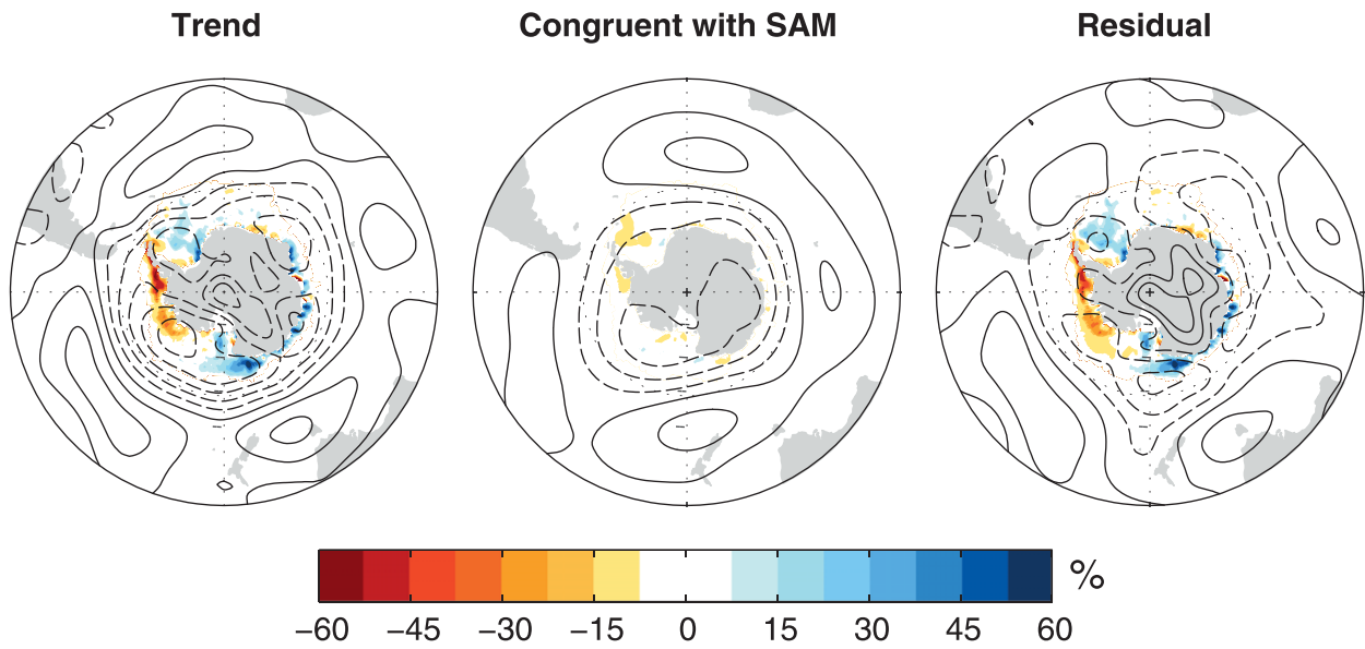
FIG. 9. (left) DJF Z_{500} (contours) and SIC (shading) trends calculated over 1980–2008, (middle) the proportion of trends congruent with DJF SAM, and (right) the residual trends after removing the effects of the DJF SAM. Positive (negative) contours are denoted by solid (dashed) lines drawn at intervals of 15 m ( -22.5 , -7.5 , 7.5 , 22.5 m . . .).
