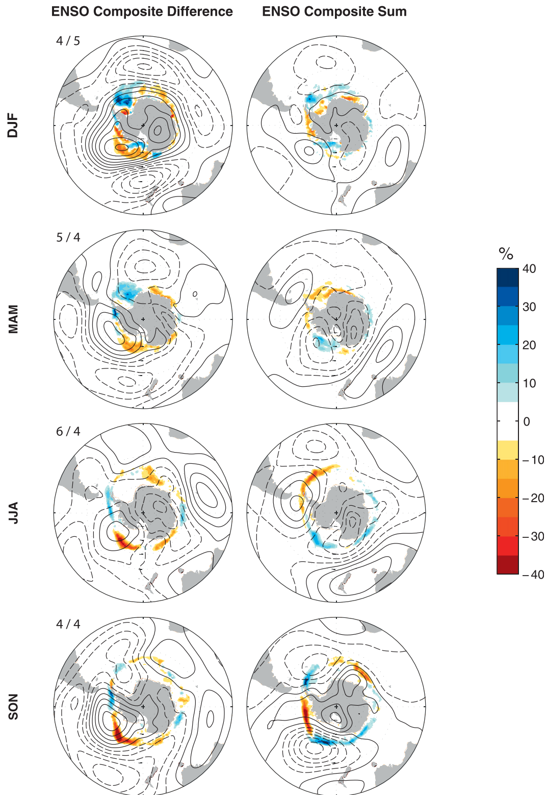
FIG. 6. As in Fig. 5 but for (left) composite differences and (right) composite sums based on seasons wherein the cold tongue ENSO index exceeds one standard deviation.
