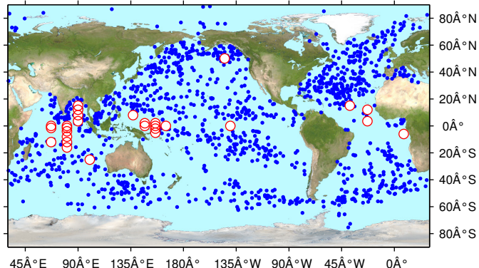
Observing system status, October–December 2014
