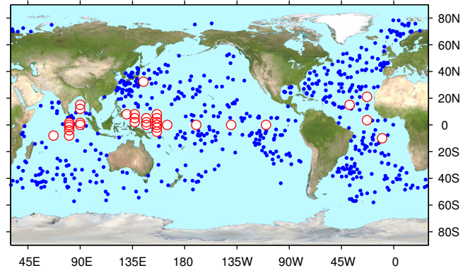
Observing system status, July–September 2008
