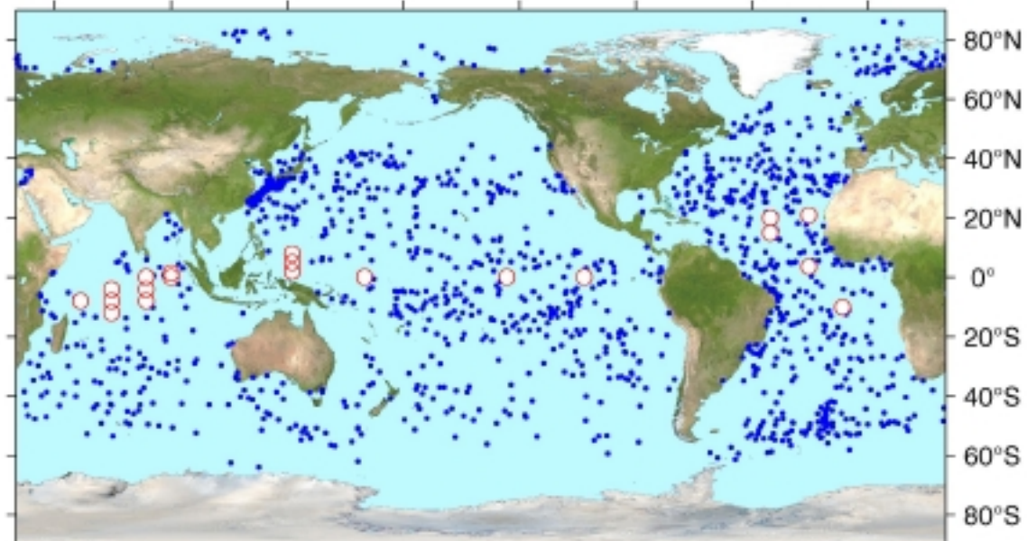
Observing system status, July–September 2009
