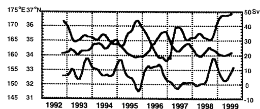
Figure 5: Time series of the monthly based latitude (green) and volume transport (red) of the KE at the first crest, and of the longitude of the BP (blue).
