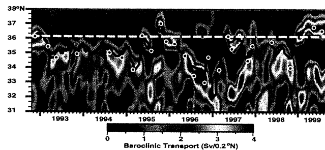
Figure 2: Time series of the baroclinic transport across groundtrack a-128 estimated every 0.2 degrees of latitude (color scale). The continuous black line indicates the location of the altimeter-derived 9°C isotherm at 500 m depth on the same groundtrack. The dots represent the latitude of the 9°C isotherm at 500 m depth from the hydrographic sections at 144°E. The horizontal dashed line at 36° 09'N represents the latitude where the a-128 and the 144°E meridian cross each other.
