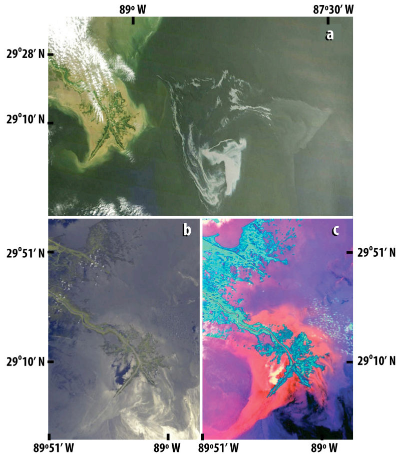
Fig. 4. (a) Oil slick as seen in a Terra MODIS visible-near IR image, distinguishable because of its a pale swirl in the darker seawater of the Gulf of Mexico just south of the Mississippi Delta on May 1, 2010, (b) MISR true color image for May 17, 2010; (c) MISR multi-angle composite acquired on the same date that separates the oil spill (black and dark blue) from specular reflections.
