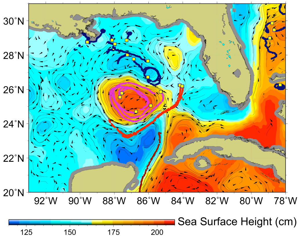
Fig. S4. Surface current vectors derived at NOAA Atlantic Oceanographic and Meteorological Laboratory from satellite altimetry observations for Jun 13, 2010. The
