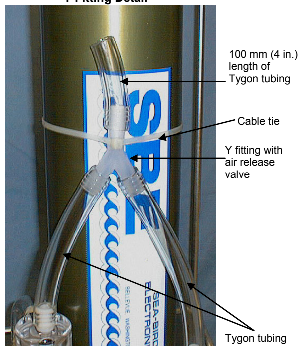
Y Fitting Detail
