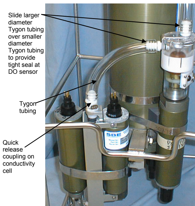
Temperature/Conductivity to DO Sensor Detail
