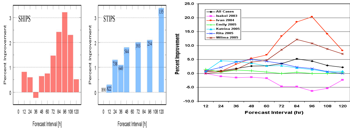
Figure 3. (left) Percent improvement of the 2004-2007 operational Statistical Hurricane Intensity Prediction Scheme (SHIPS) forecasts for the Atlantic sample of over-water cases west of 50^{\circ}\text{W} due to the inclusion of input from TCHP-derived altimetry and GOES infrared cloud-top temperature information. (center) Percent improvement that results from the use of TCHP information in the Statistical Typhoon Intensity Prediction Scheme (STIPS) forecast model. (right) The percentage of SHIPS model forecast improvement, for six category 5 Atlantic hurricanes and collectively, with the incorporation of the TCHP fields, created at the NOAA National Hurricane Center (adapted from Mainelli et al., 2008).
