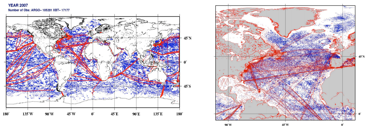
Figure 2. (left) Locations of profiling float (blue) and XBT (red) observations transmitted in real-time into the Global Telecommunication System (GTS) during 2007. (right) Locations of profiling float (blue) and XBT (red) observations in the North Atlantic transmitted into the GTS during 2003-2008.
