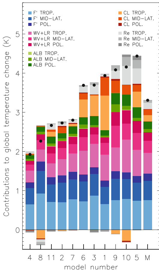
(b) FEEDBACKS + FORCINGS
