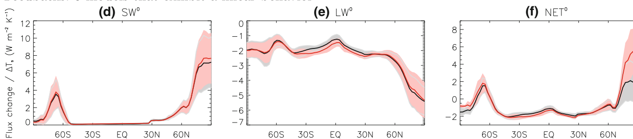
Fig. 4 Same as Fig. 3 but for the feedbacks. TOA flux changes derived from model output have been normalized by \Delta T_{s,\Delta SST} for comparison with the feedbacks. Units are W\ m^{-2}\ K^{-1} . a–c is the SW, LW and NET components for all models, and d–f is for the 6 models that exhibit a linear behavior (for \%Re^f < 10 in Table 3)
