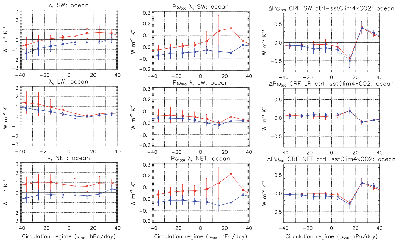
Fig. 13 SW (top), LW (middle) and NET (bottom) cloud feedback ( \Delta C ) composited in each dynamical regime (left), the contribution from the thermodynamic component ( P_\omega \Delta C_\omega , middle) and from the dynamic component ( C_\omega \Delta P_\omega , right). Results are presented for two groups of models: models that predicts a greater tropically-averaged
