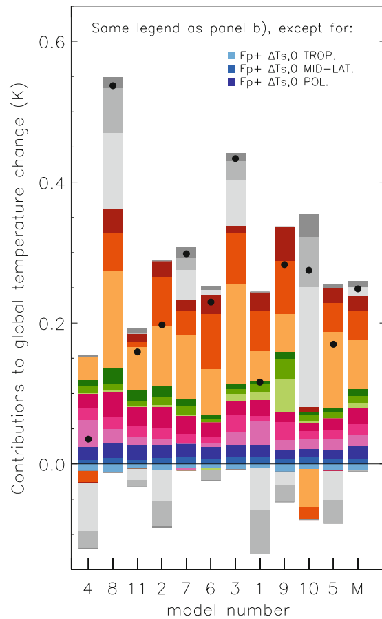
(c) FORCINGS: ADJUSTMENTS
