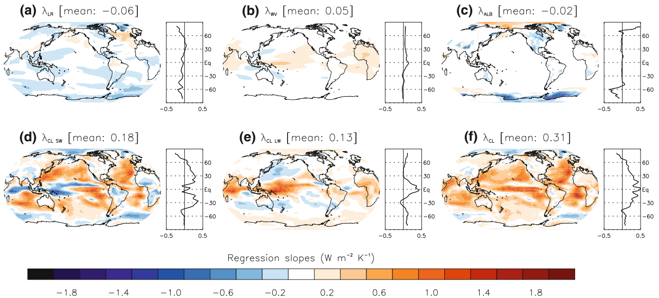
Fig. 8 Inter-model regression slopes of the lapse rate (a), water vapor (b), albedo (c) and cloud (SW in d; LW in e; NET in f) feedbacks against the global mean surface temperature change for the 11 models considered in this study and reported in Table 1. Large values indicate
