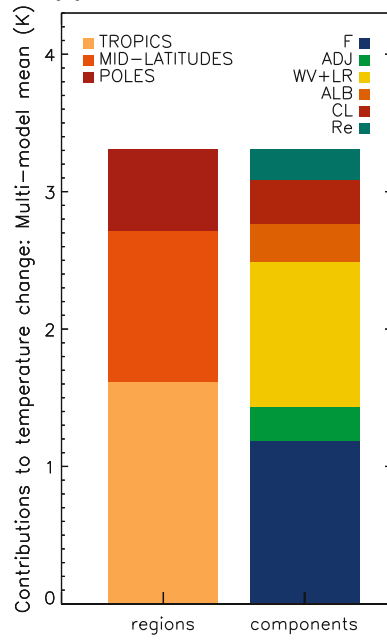
(a) FEEDBACKS + FORCINGS
