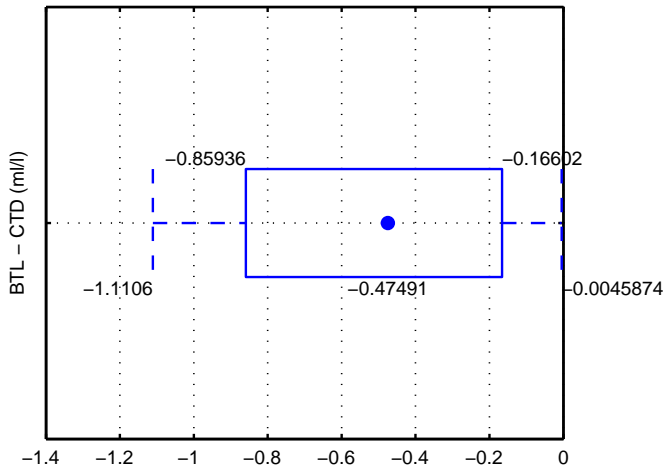
Box Plot of BTL - CTD Oxygen - Uncalibrated Data - Below 0 dbar
