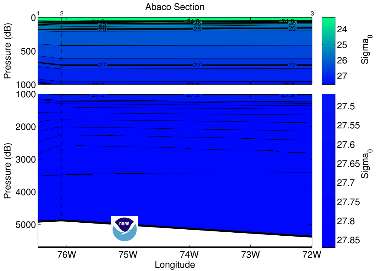
Figure 26: Neutral density ( \text{kg/m}^3 ) section for the Abaco Section. Dashed vertical lines are the CTD station locations.
