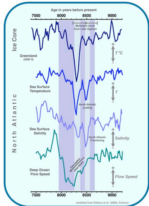
Figure 3.2: Evidence for surface and deep ocean links during the 8.2 kyr abrupt climate change event in the sub-polar North Atlantic Ocean. From top to bottom (i) the GISP2 temperature ( \delta T ) record (ii) Core MD99-2251 N. pachyderma s. percent abundance data (higher abundances indicate sea surface cooling), (iii) surface ocean salinity, and (iv) sortable silt mean palaeocurrent speed index. Shaded bars indicate the two pulses of cooling and freshening of surface ocean conditions that appear to correlate with a larger (3.6 Sv) Lake Agassiz outburst at ~7,700 C years B.P. and a second, smaller meltwater discharge (1.6 Sv) dated at ~7,600 C years B.P. The 8.2 kyr abrupt climate change event has a duration of ~70 years in both ice and ocean records.
