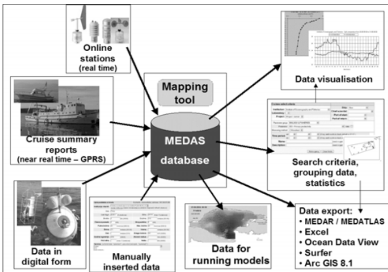
Fig. 2. Database functionalities.
