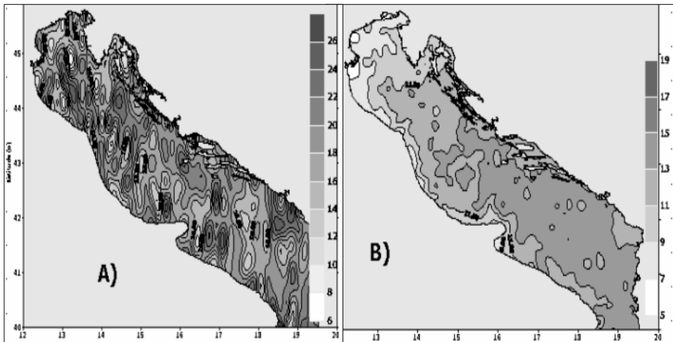
Fig. 12. Interpolated field of mean value of temperature at the sea surface gathered from the original data (A) and data passed quality control (B).
