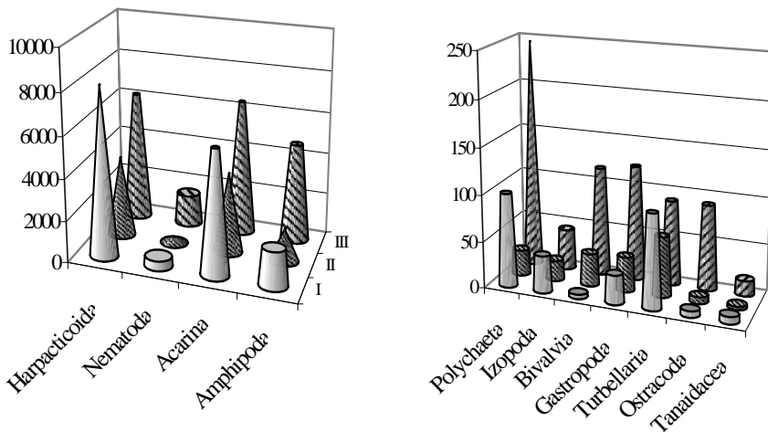
Fig. 3. Average abundance ( \text{ind.kg}^{-1} algal wet weight) for the major meiobenthos taxa in the Kruglaya Bay at locality I, II, III (May 1990 - May 1991).
