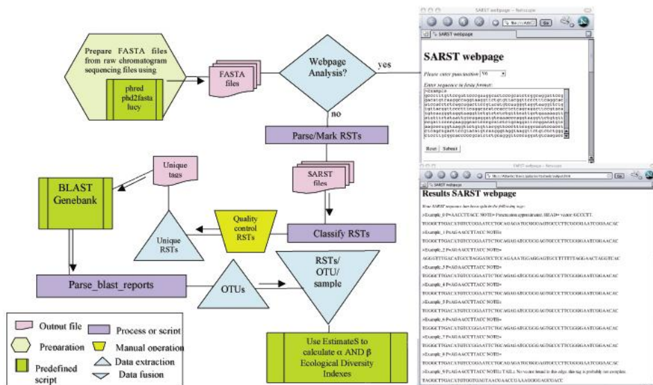
Fig. 1. SARST-V6 pipeline. This pipeline outlines the different stages of SARST-V6 sequence analysis (see text for details).
