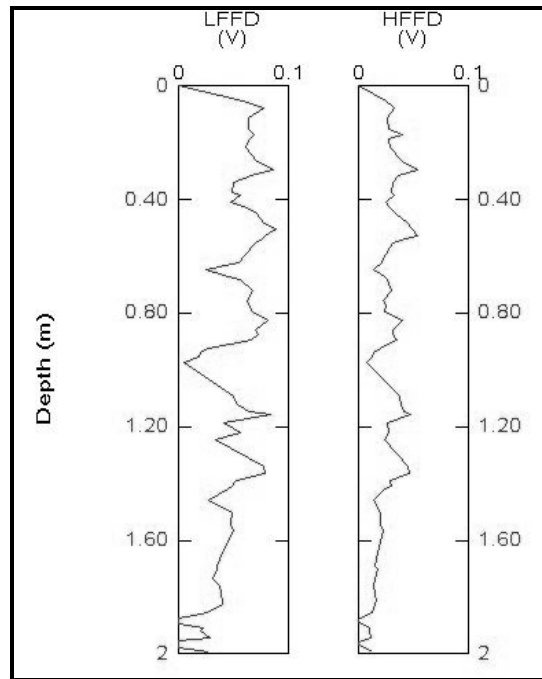
Figure 12: FFD probe analysis of BP-18.
