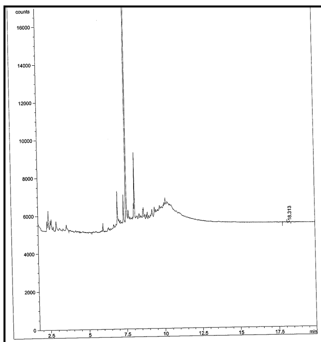
Chromatogram for sediment core BP-31 (265-271 cm).
