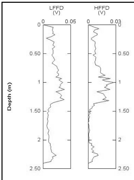
Figure 31: FFD probe analysis of BP-71.
