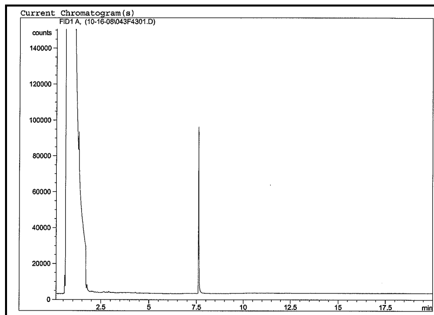
Chromatogram of sediment core JP-10 (88-93 cm).
