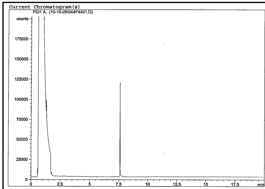
Chromatograph of sediment core JP-15 (240-245 cm).
