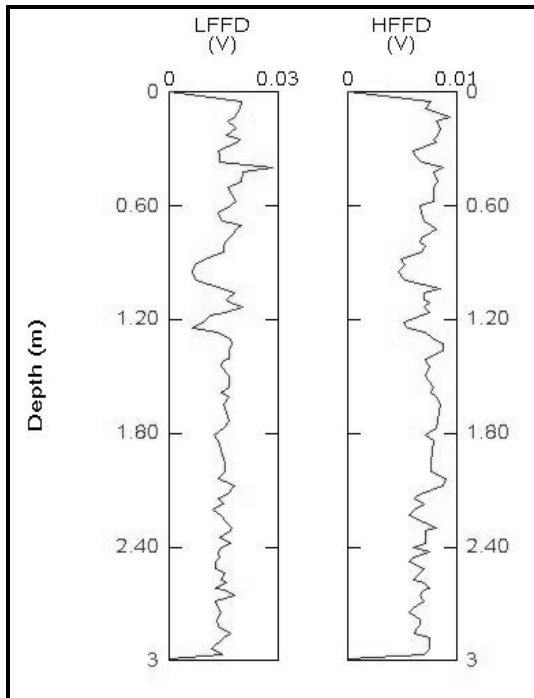
Figure 27: FFD probe analysis of BP-47.
