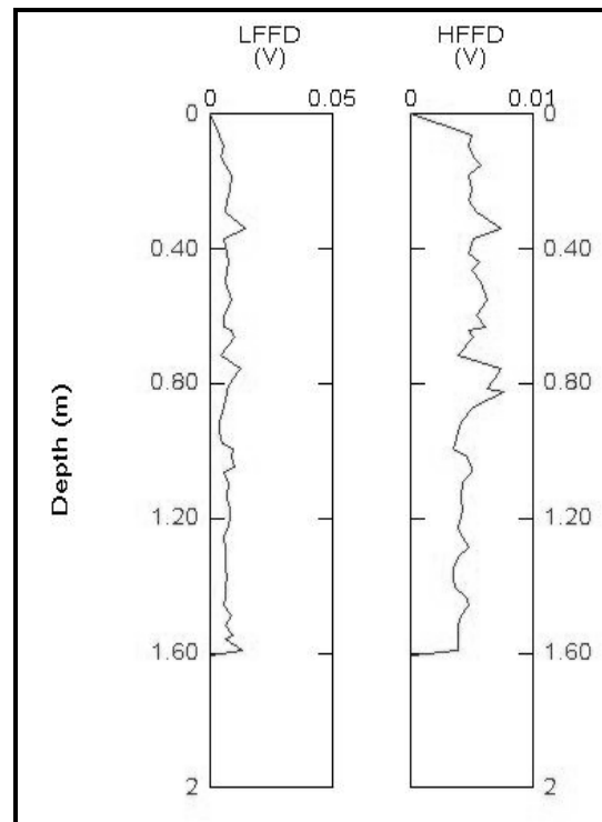
Figure 60: FFD probe analysis of BP-65.
