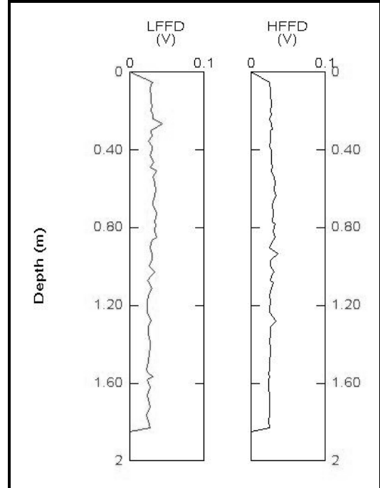
Figure 6: FFD probe analysis of BP-59.
