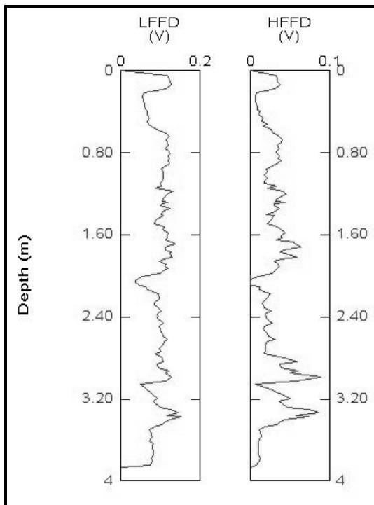
Figure 63: FFD probe analysis of BP-49.
