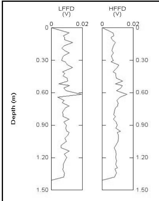
Figure 25: FFD probe analysis of BP-6.
