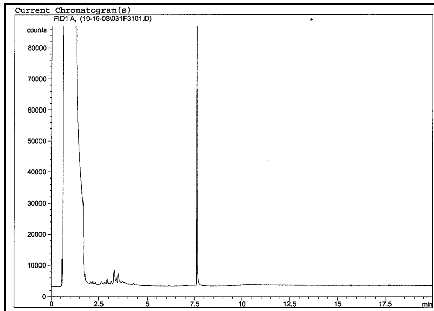
Chromatograph of sediment core JP-3 (85-90 cm).
