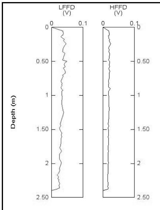
Figure 19: FFD probe analysis of JP-4.
