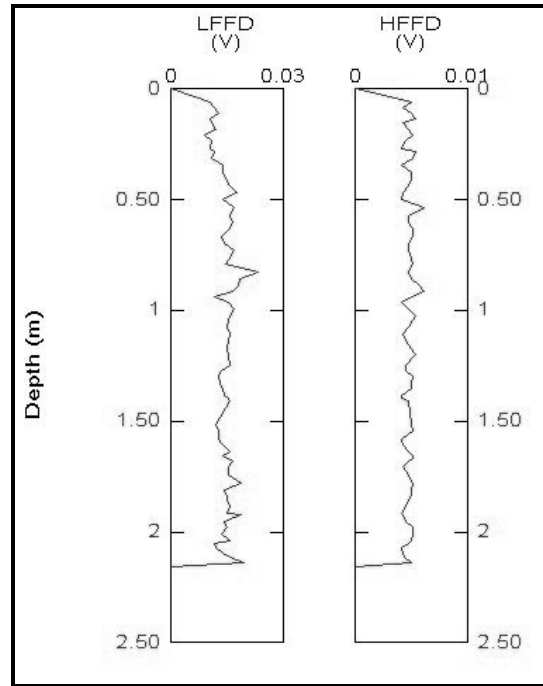
Figure 82: FFD probe analysis of BP-92.
