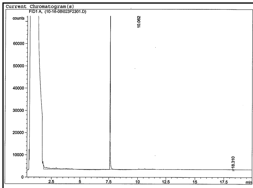
Chromatogram of sediment core JP-13 (65-70 cm).
