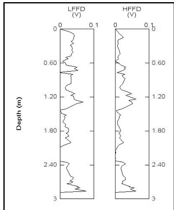
Figure 92: FFD probe analysis of BP-89.
