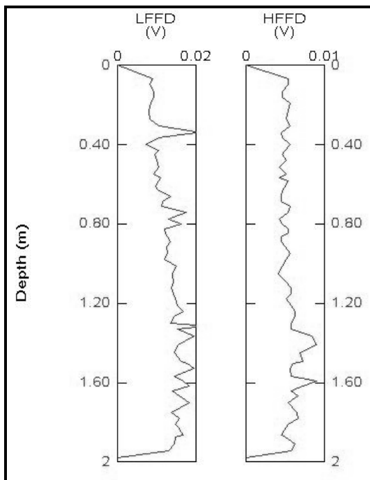
Figure 87: FFD probe analysis of BP-73.
