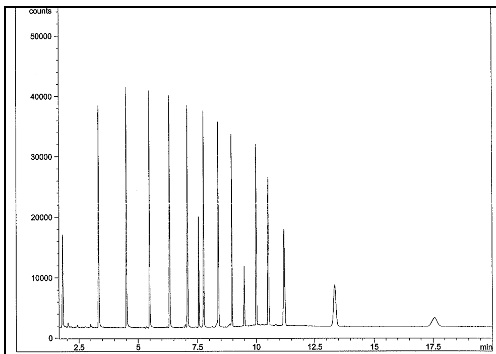
Chromatogram
