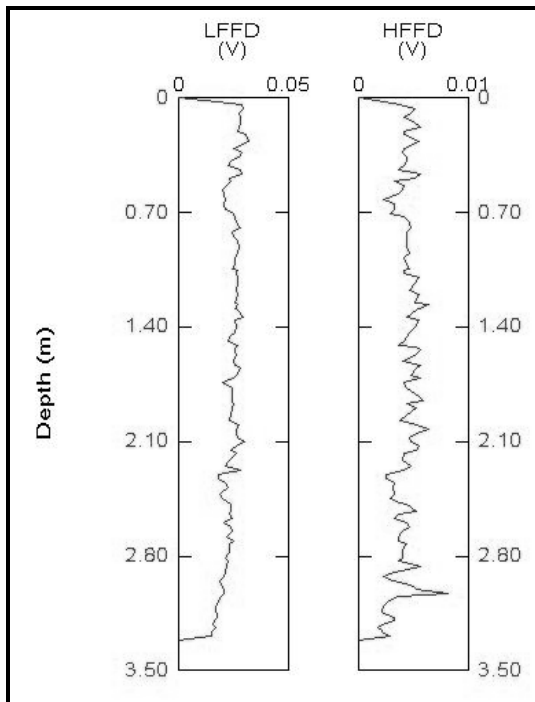
Figure 67: FFD probe analysis of BP-57.
