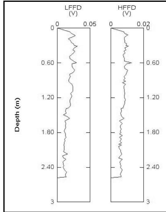
Figure 30: FFD probe analysis of BP-55.
