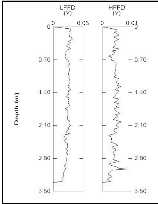
Figure 97: FFD probe analysis of BP-C.
