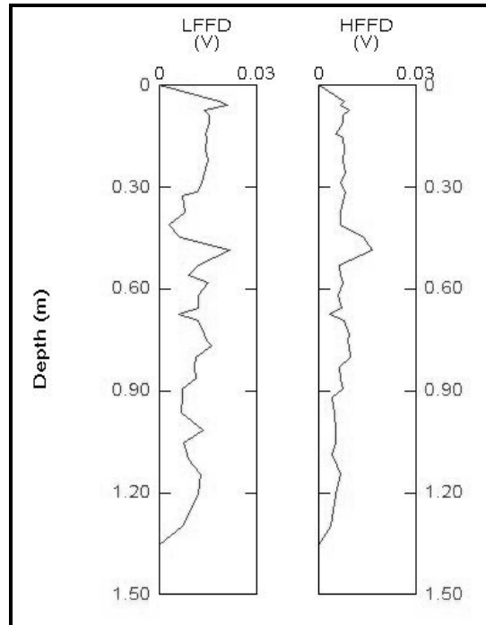
Figure 24: FFD probe analysis of BP-25.
