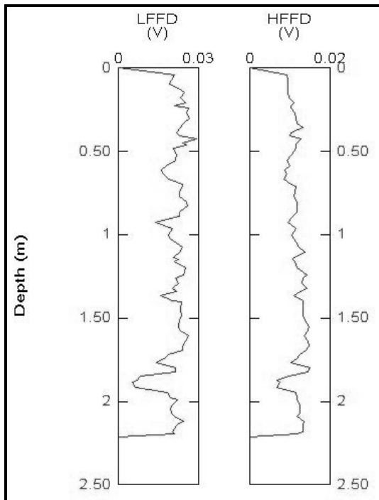
Figure 79: FFD probe analysis of BP-87.
