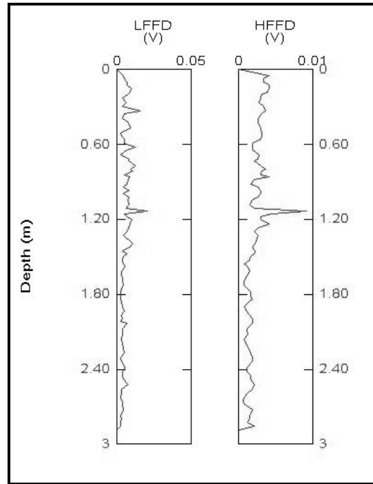
Figure 58: FFD probe analysis of BP-63.
