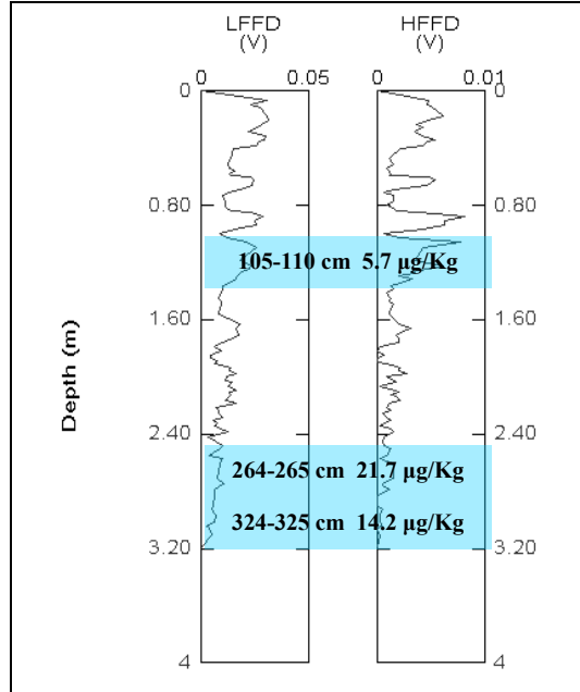
Figure 44: FFD probe analysis of sediment core BP-24.
