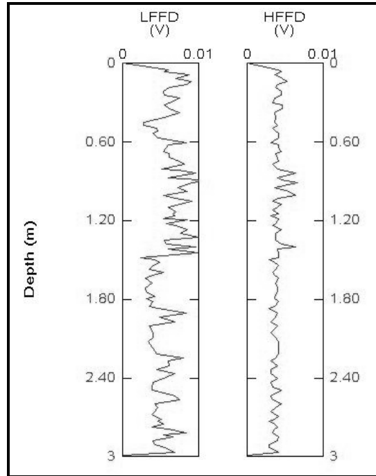
Figure 74: FFD probe analysis of BP-62.
