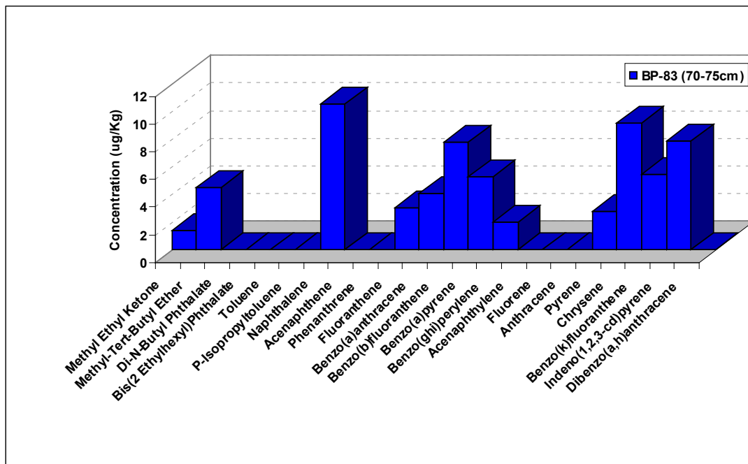
Figure 16D: Individual petroleum hydrocarbon speciation of BP-83 (70-75 cm) from the South Channel of Blind Pass.
