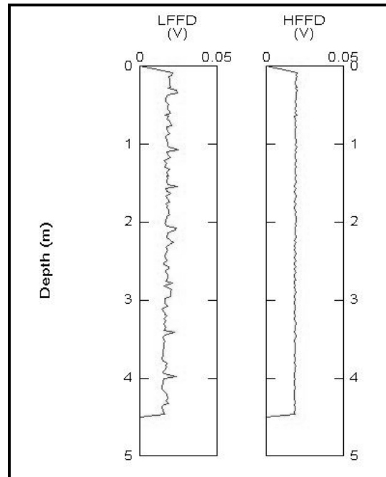
Figure 30: FFD probe analysis of JP-15.
