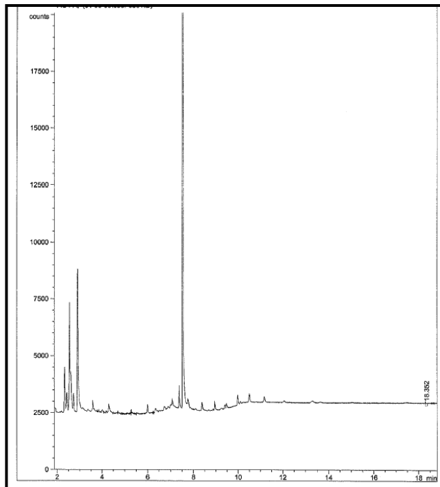
Chromatogram for sediment core BP-76 (78-81 cm).
