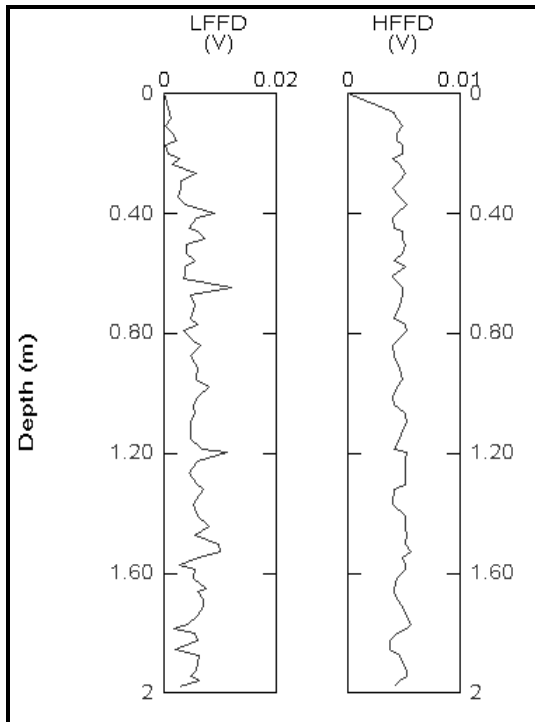
Figure 83: FFD probe analysis of BP-52.
