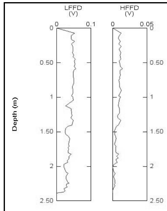
Figure 20: FFD probe analysis of BP-90.
