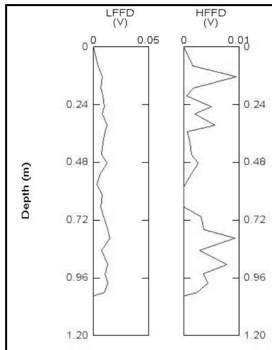
Figure 8: FFD probe analysis of BP-80.
