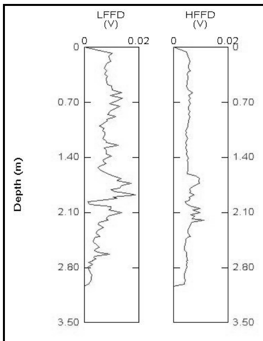
Figure 35: FFD probe analysis of BP-35.
