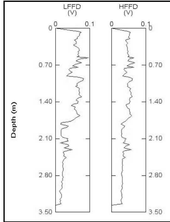
Figure 66: FFD probe analysis of BP-61.
