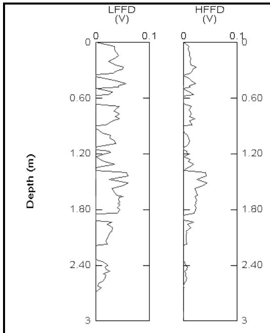
Figure 1: FFD probe analysis of BP-12.
