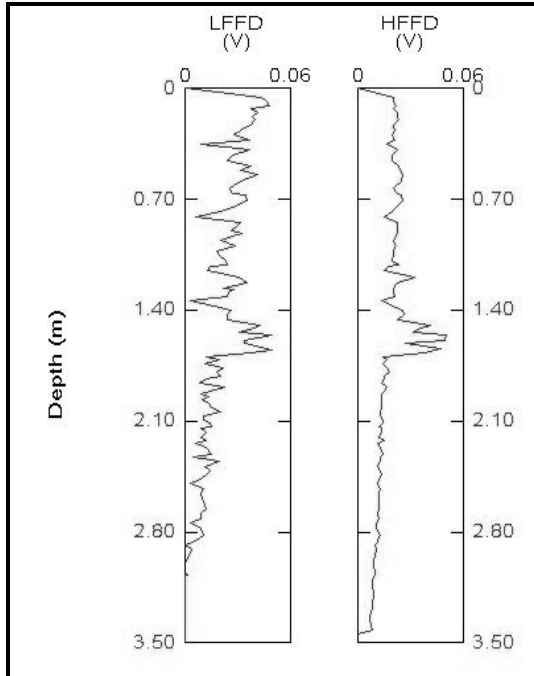
Figure 61: FFD probe analysis of BP-8.
