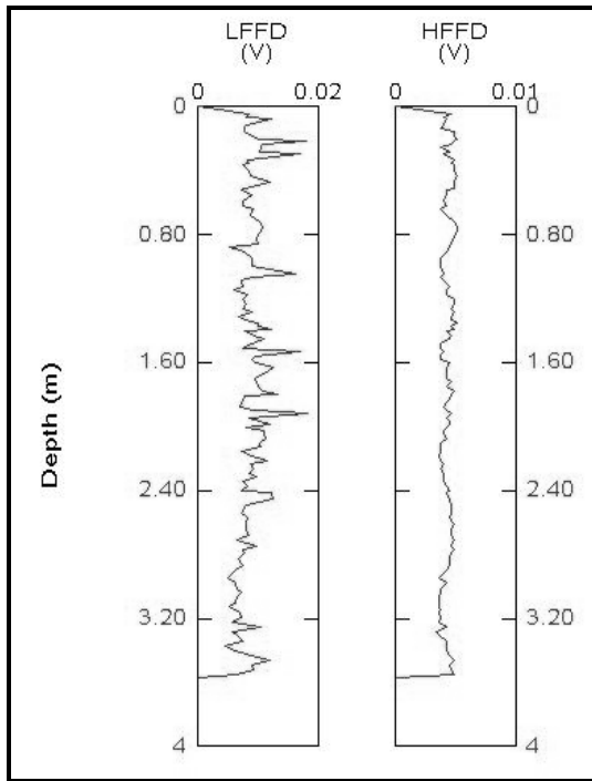
Figure 41: FFD probe analysis of BP-20.
