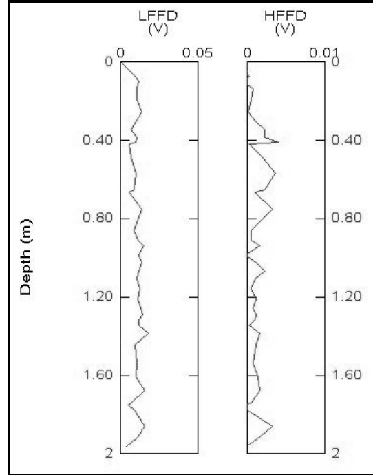
Figure 10: FFD probe analysis of BP-91.
