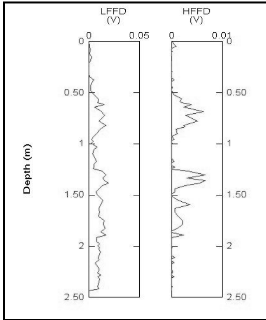
Figure 17: FFD probe analysis of JP-1.
