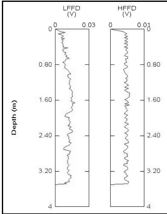
Figure 81: FFD probe analysis of BP-7.
