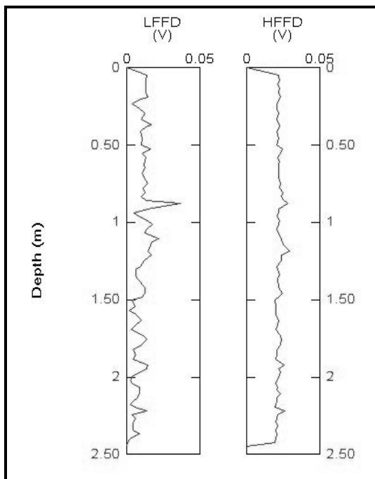
Figure 19: FFD probe analysis of BP-82.
