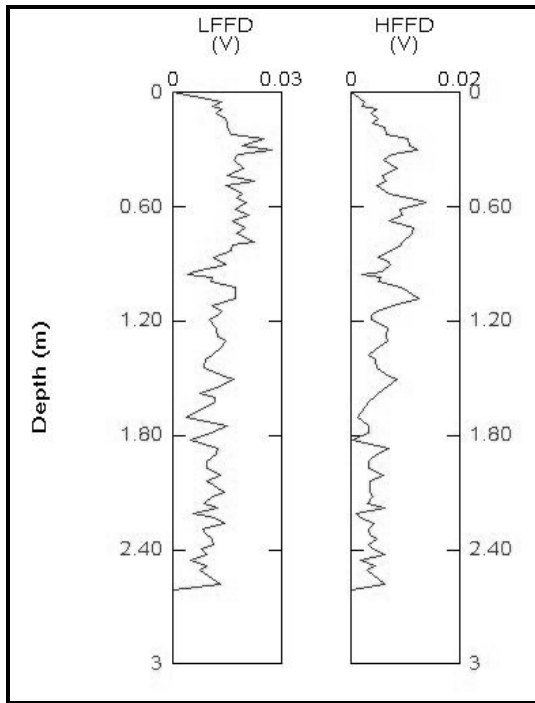
Figure 33: FFD probe analysis of BP-38.
