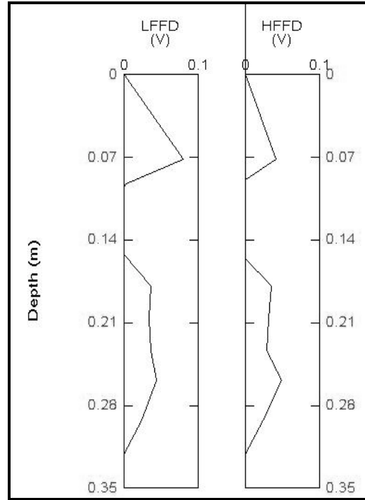
Figure 98: FFD probe analysis of BP-84.
