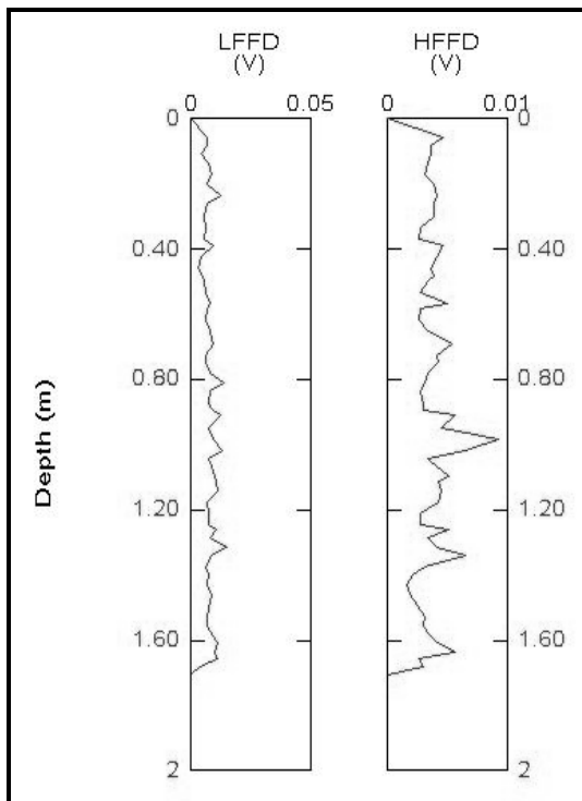
Figure 59: FFD probe analysis of BP-66.
