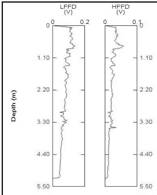
Figure 89: FFD probe analysis of BP-19.
