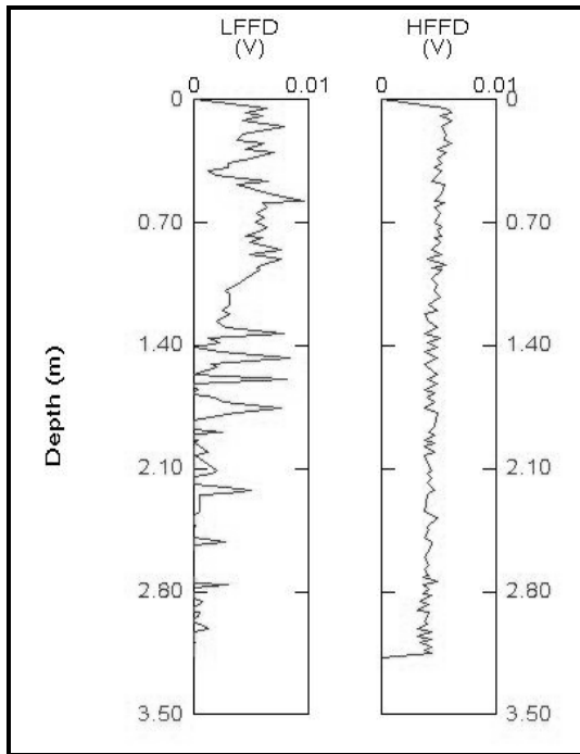
Figure 53: FFD probe analysis of BP-54.
