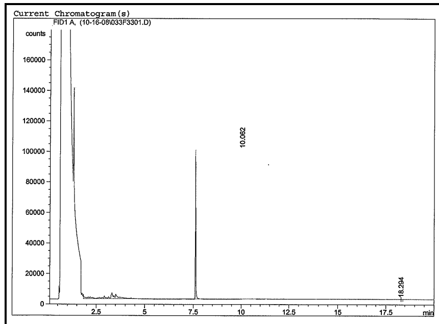
Chromatograph of sediment core JP-14 (235-240 cm).
