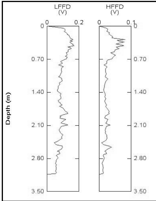
Figure 29: FFD probe analysis of BP-44.
