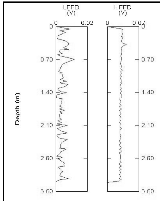
Figure 26: FFD probe analysis of JP-11(2).
