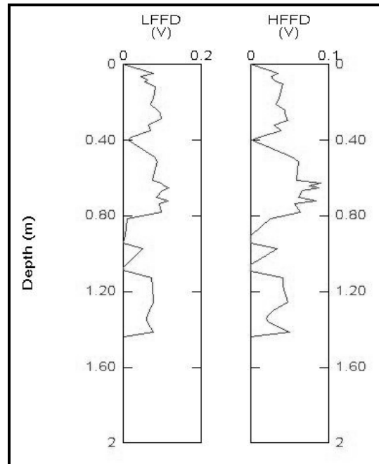
Figure 2: FFD probe analysis of BP-2.
