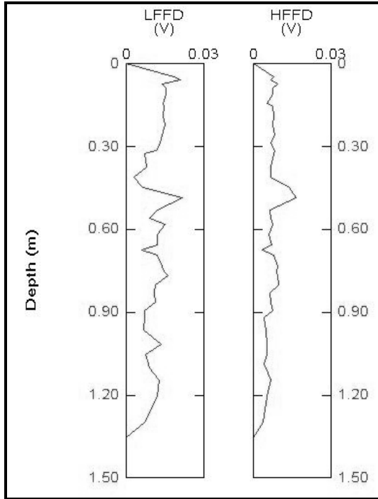
Figure 65: FFD probe analysis of BP-78.
