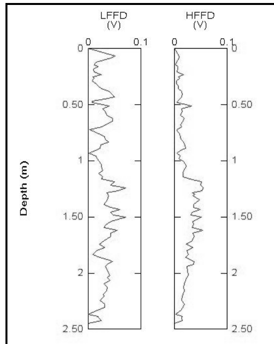
Figure 88: FFD probe analysis of BP-16.
