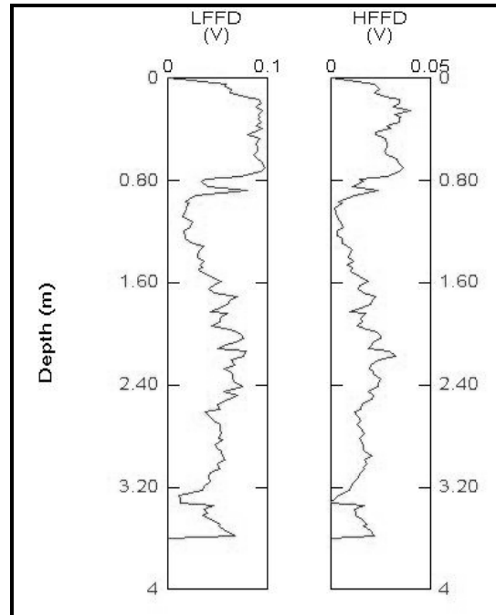
Figure 62: FFD probe analysis of BP-27.
