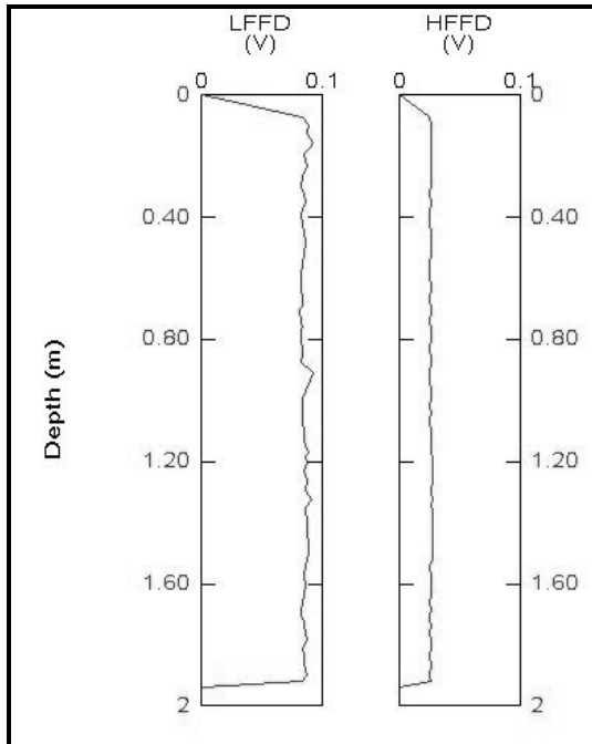
Figure 25: FFD probe analysis of JP-10.
