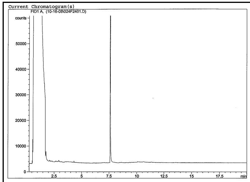
Chromatogram of sediment core JP-12-2 (120-125 cm).
