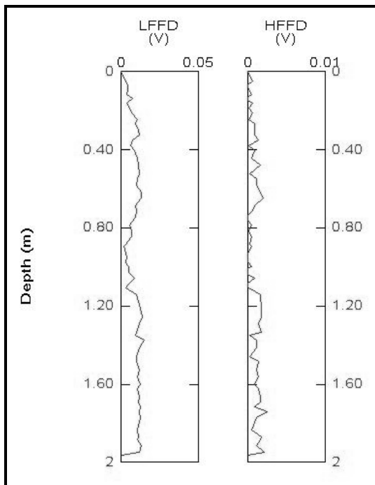
Figure 27: FFD probe analysis of JP-12(2).
