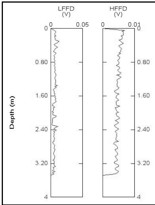
Figure 57: FFD probe analysis of BP-86.
