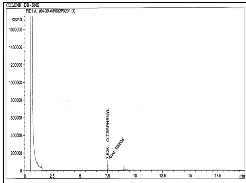
Chromatogram for sediment core BP-83 (70-75 cm).
