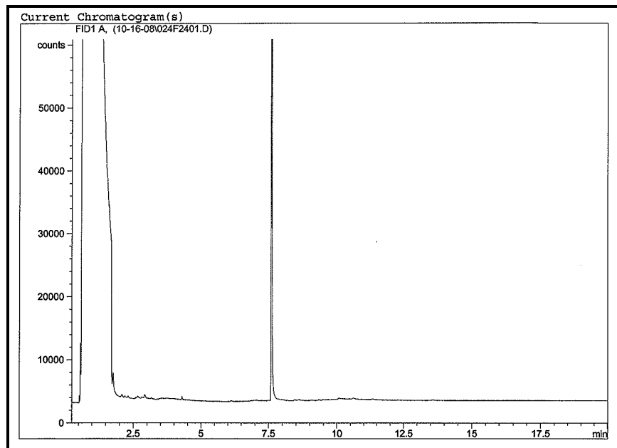
Chromatogram of sediment core JP-11-2 (148-153 cm).
