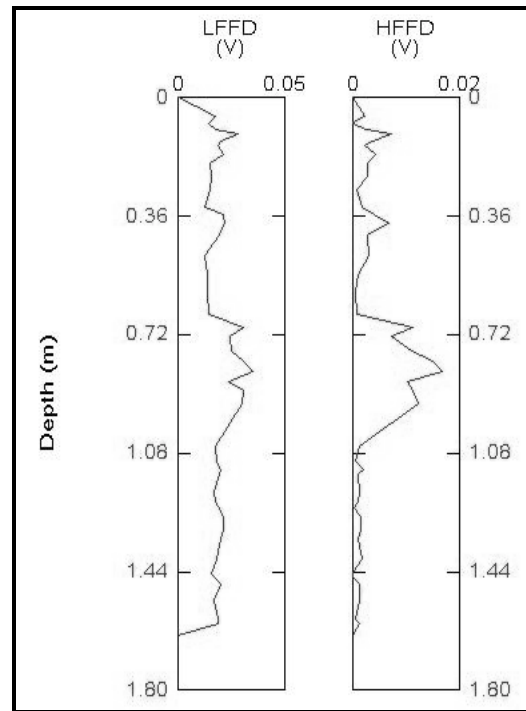
Figure 100: FFD probe analysis of BP-83.
