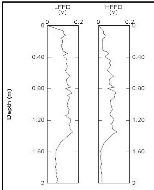
Figure 77: FFD probe analysis of BP-A.
