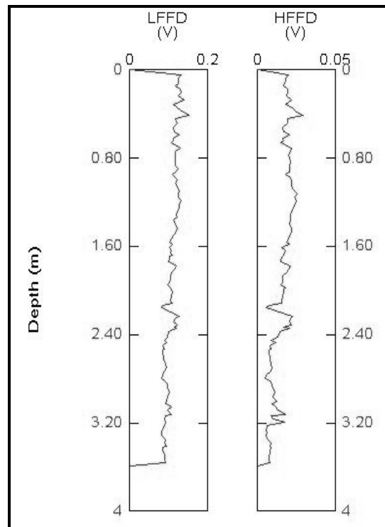
Figure 44: FFD probe analysis of BP-5.
