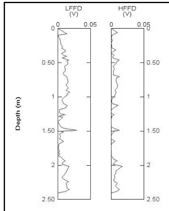
Figure 52: FFD probe analysis of BP-37.
