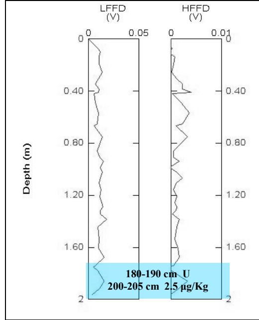
Figure 50: FFD probe analysis of sediment core BP-91.
