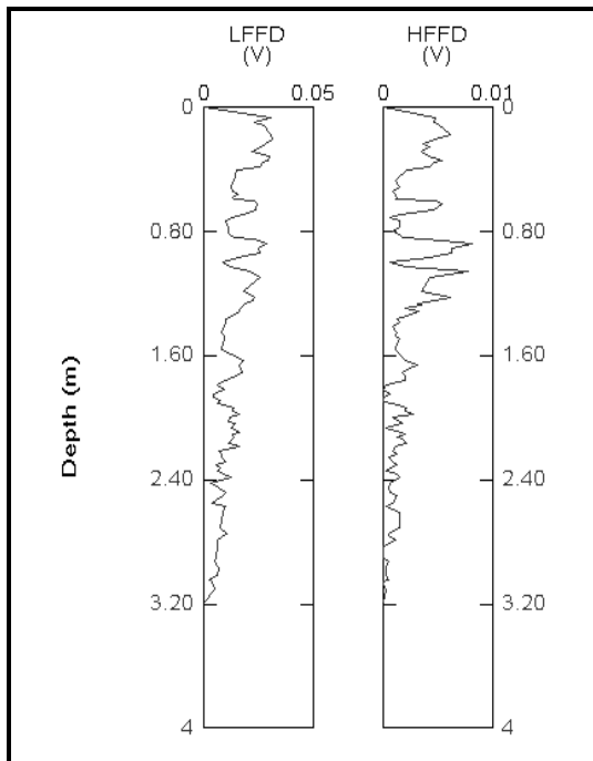
Figure 3: FFD probe analysis of BP-26.
