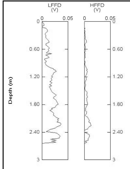
Figure 20: FFD probe analysis of JP-5.
