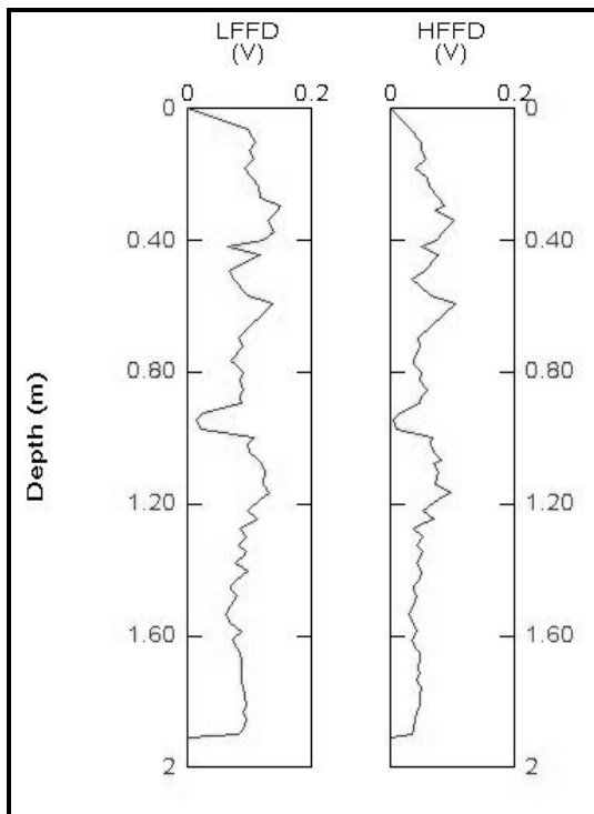
Figure 43: FFD probe analysis of BP-11.
