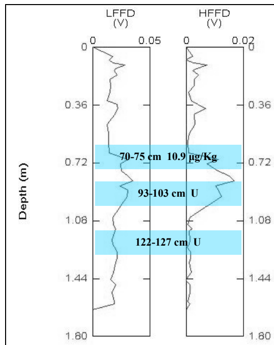
Figure 56: FFD probe analysis of sediment core BP-83.
