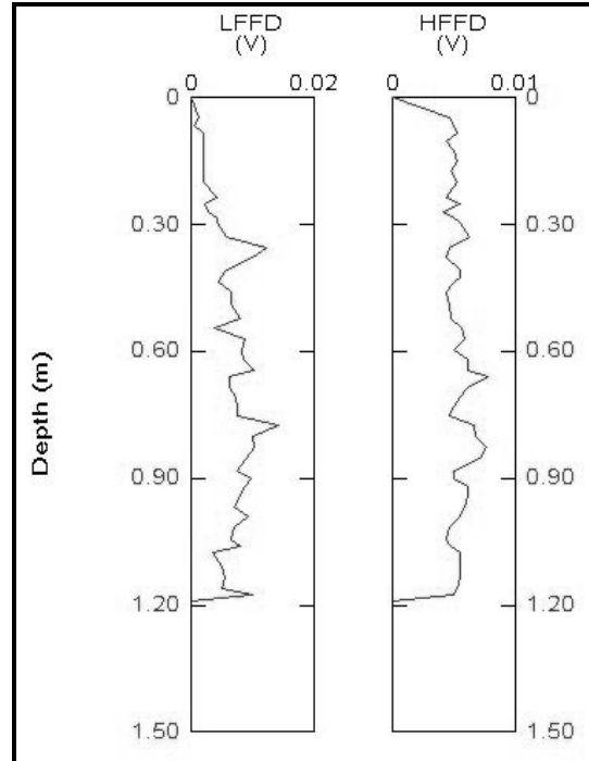
Figure 86: FFD probe analysis of BP-74.
