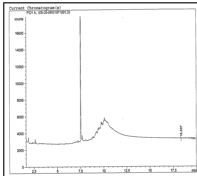
Chromatogram for sediment core BP-81 (328-338 cm).
