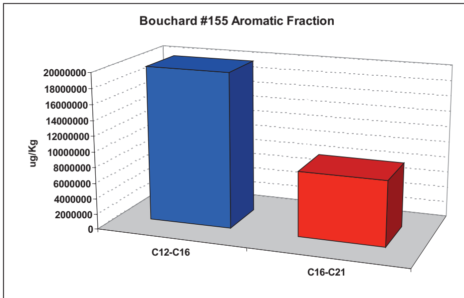
Figure 11: Aromatic fractions in the Bouchard 155 reference sample.
