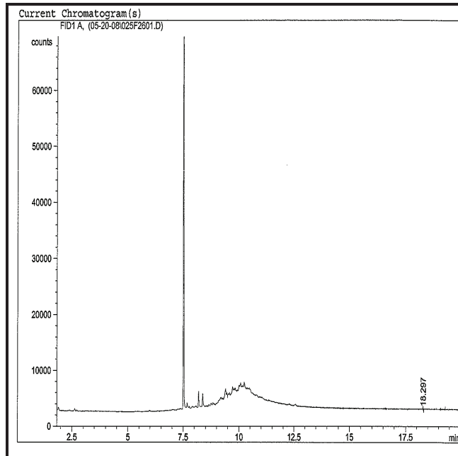
Chromatogram for sediment core BP-45 (225-230 cm).
