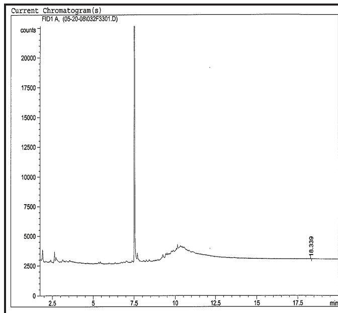
Chromatogram for sediment core BP-24 (116-121 cm).
