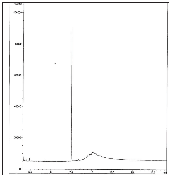
Chromatogram of sediment core BP-35 (116-120 cm).
