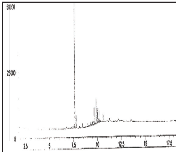
Chromatogram for sediment core BP-97 (192-197 cm).
