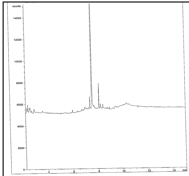
Chromatogram for sediment core BP-31 (214-219 cm).
