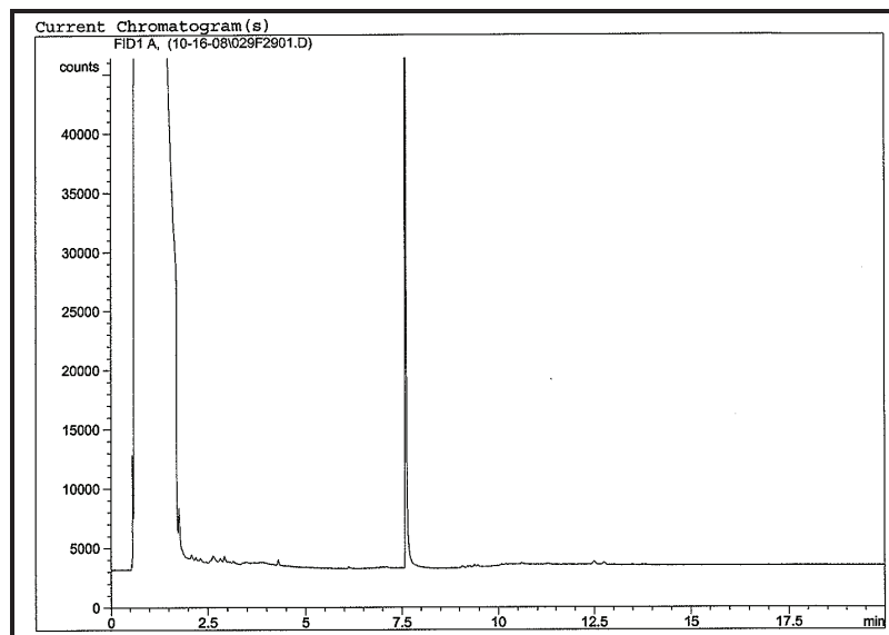
Chromatogram of sediment core JP-1 (115-120 cm).
