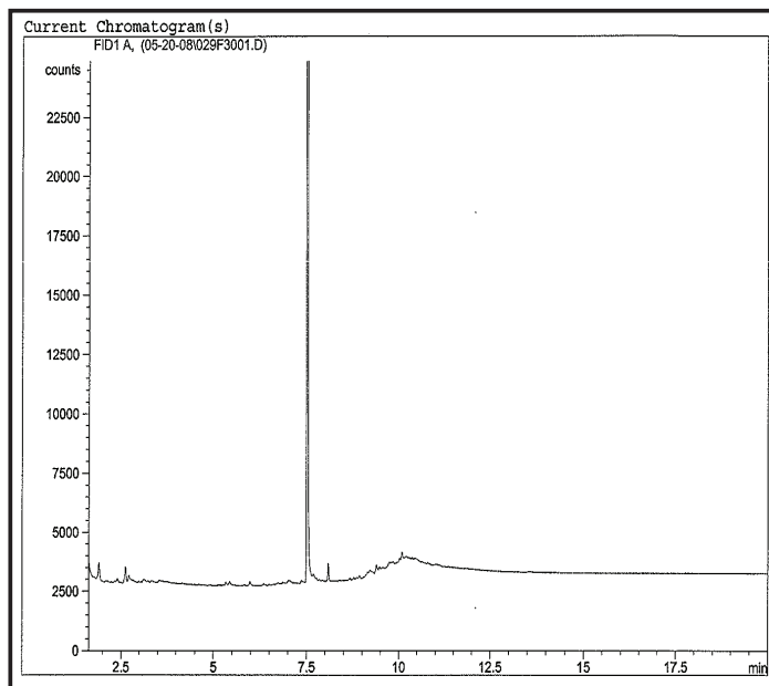
Chromatogram for sediment core BP-70 (236-241 cm).
