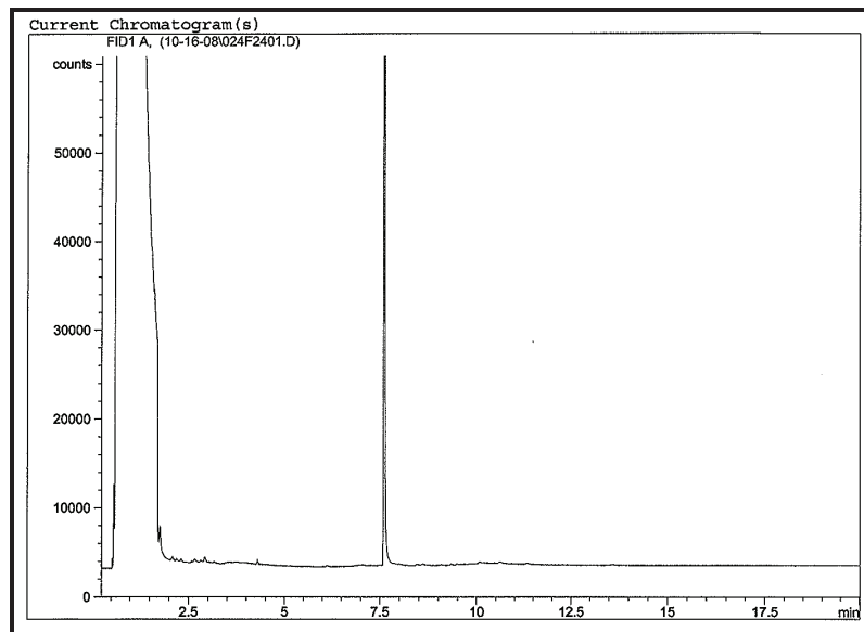
Chromatograph of sediment core JP-12-2 (120-125 cm).
