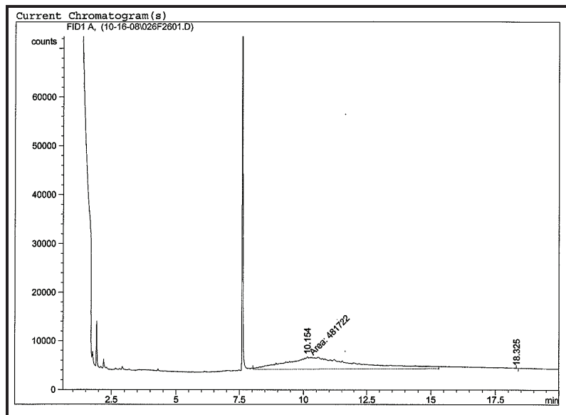
Chromatograph of sediment core JP-9 (70-75 cm).
