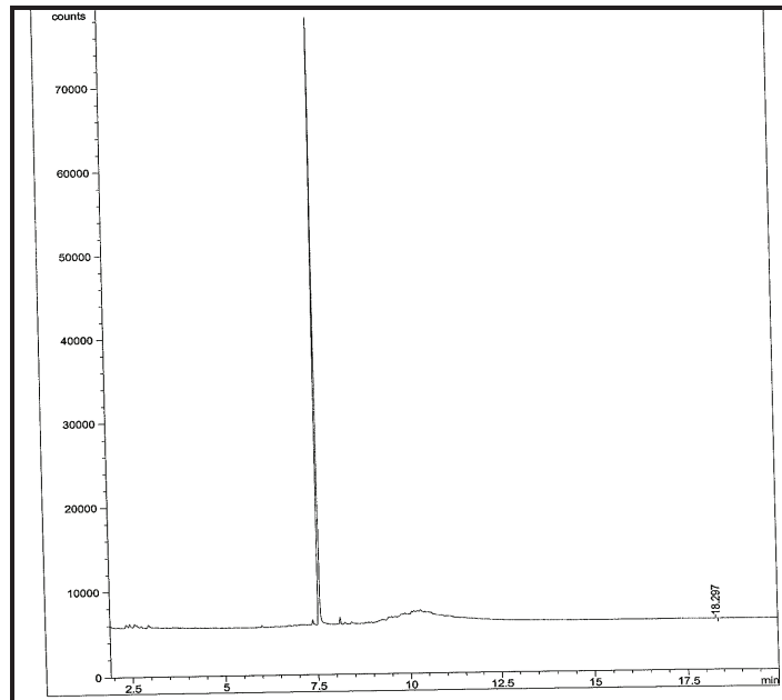
Chromatogram for sediment core BP-26 (262-263 cm).
