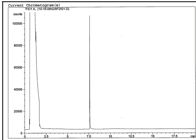
Chromatograph of sediment core JP-6 (65-70 cm).
