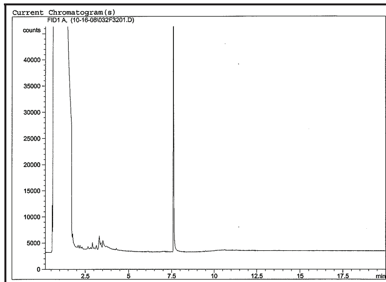
Chromatograph of sediment core JP-8 (180-185 cm).
