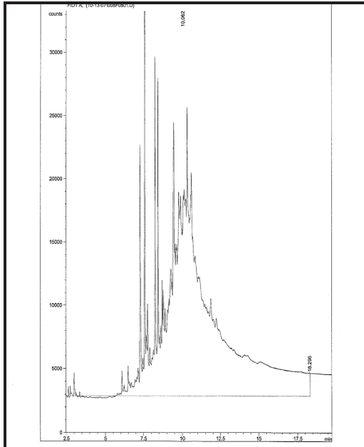
Chromatogram for sediment core BP-45 (266-272 cm).
