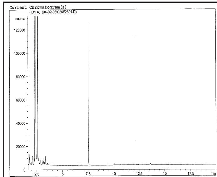
Chromatogram for sediment core BP-1 (249-254 cm).
