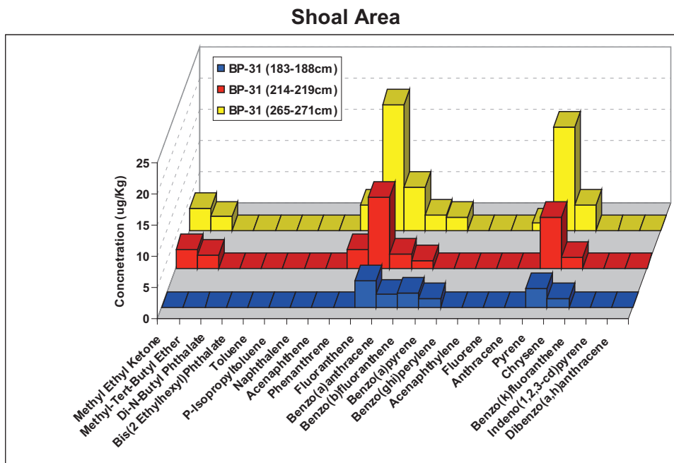
Figure 17C: Individual petroleum hydrocarbon speciation of BP-31 (183-188 cm, 214-219 cm, and 265-271 cm) from the Shoal area of Blind Pass.
