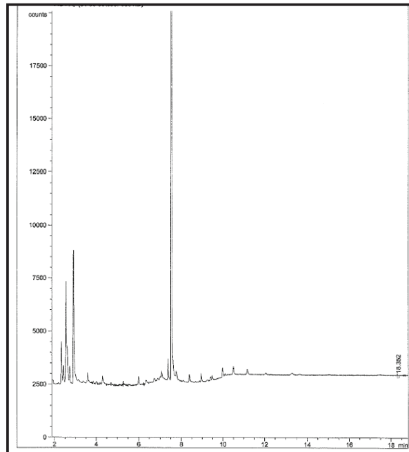
Chromatogram for sediment core BP-76 (78-81 cm).
