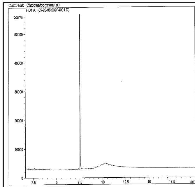
Chromatogram for sediment core BP-76 (224-229 cm).
