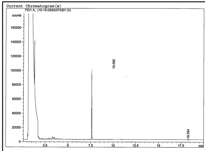
Chromatograph of sediment core JP-14 (235-240 cm).
