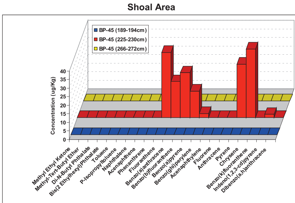
Figure 17D: Individual petroleum hydrocarbon speciation of BP-45 (189-194 cm, 225-230 cm, and 266-272 cm) from the Shoal area of Blind Pass.
