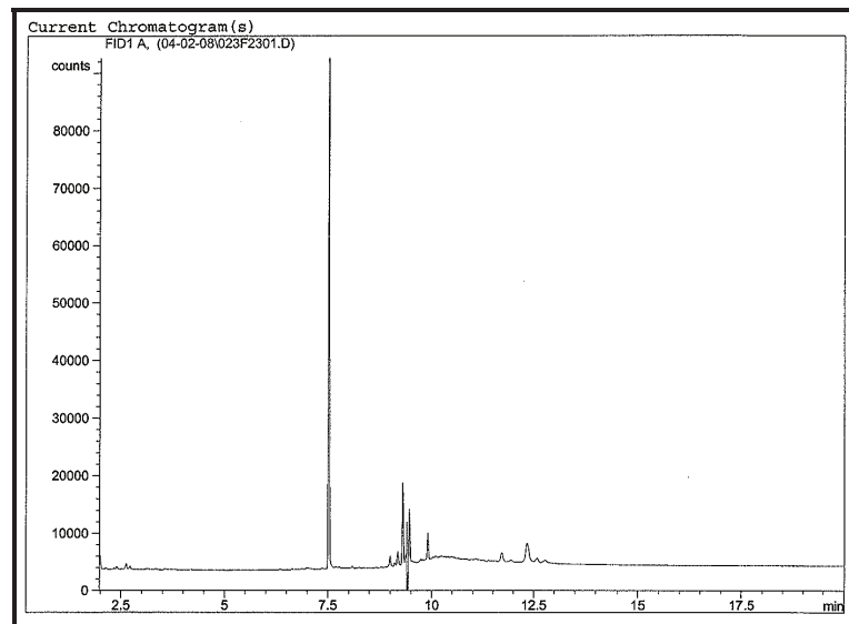
Chromatogram for sediment core BP-73 (48-53 cm).
