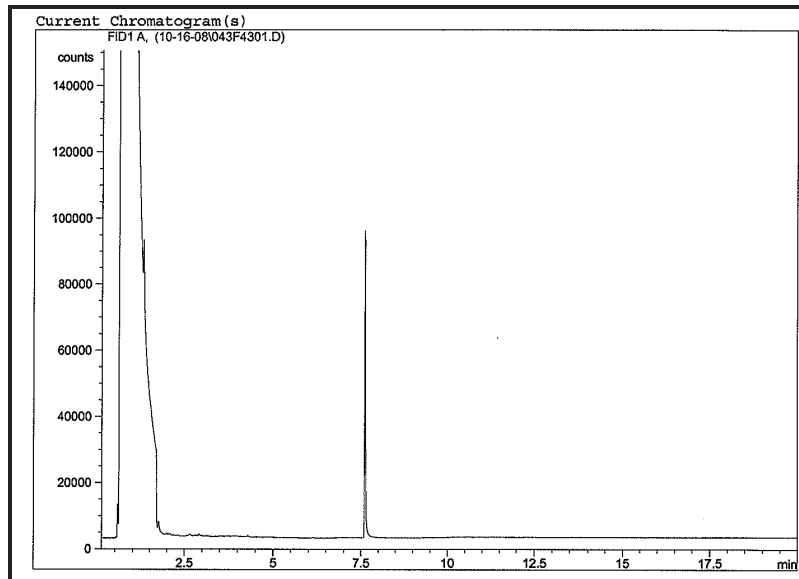
Chromatograph of sediment core JP-10 (88-93 cm).
