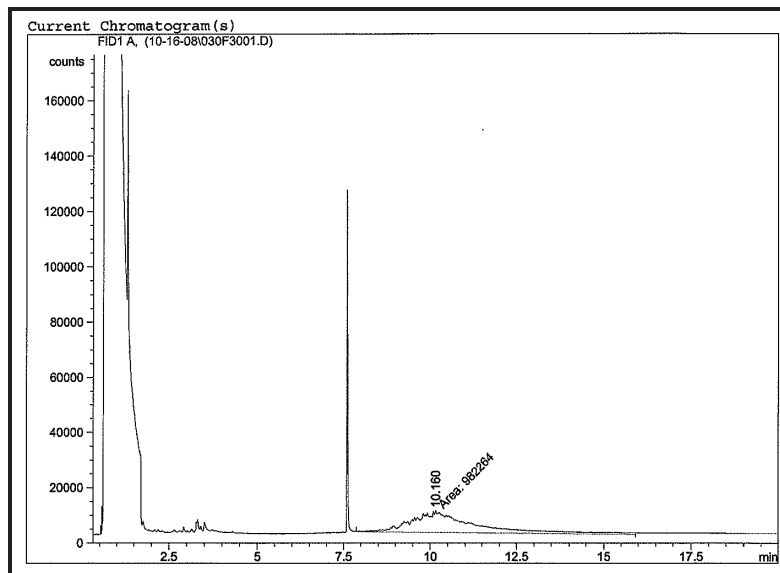
Chromatogram of sediment core JP-7 (145-250 cm).
