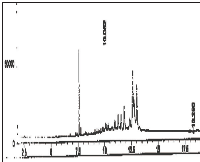
Chromatogram of sediment core BP-70 (24-26 cm).
