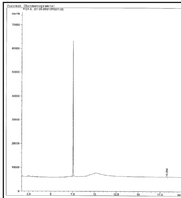
Chromatogram for sediment core 90 (221-223 cm).
