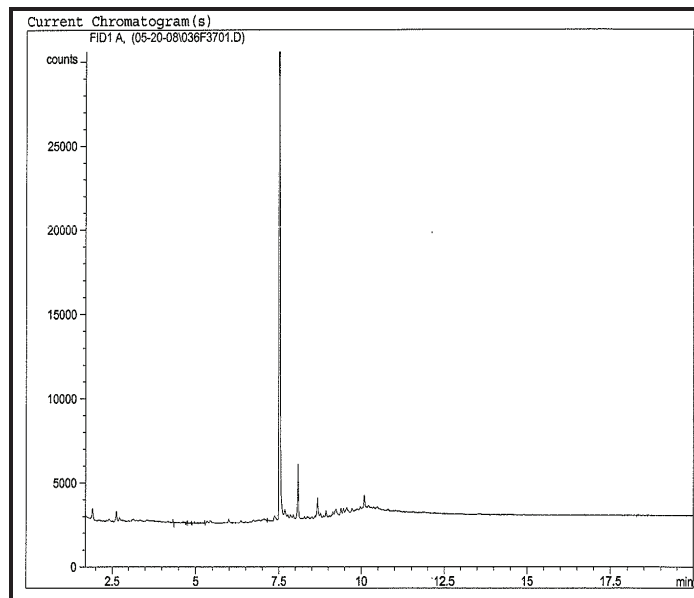
Chromatogram for sediment core BP-39 (256-266 cm).
