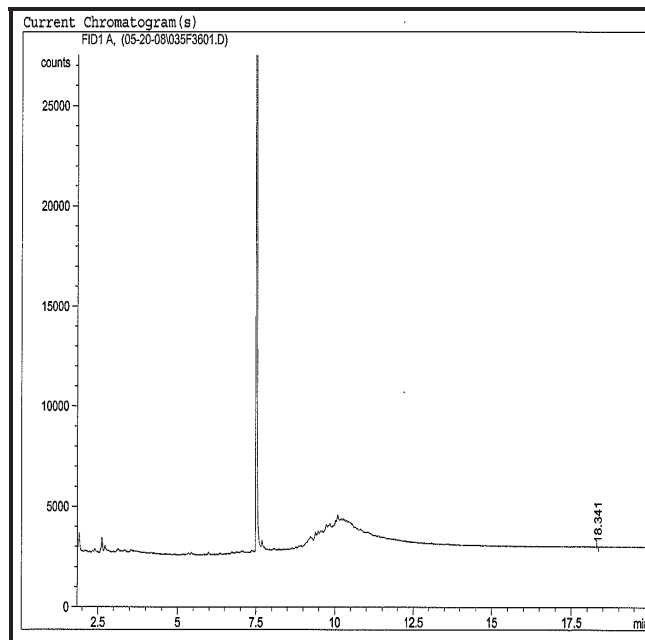
Chromatogram for sediment core BP-39 (168-178 cm).
