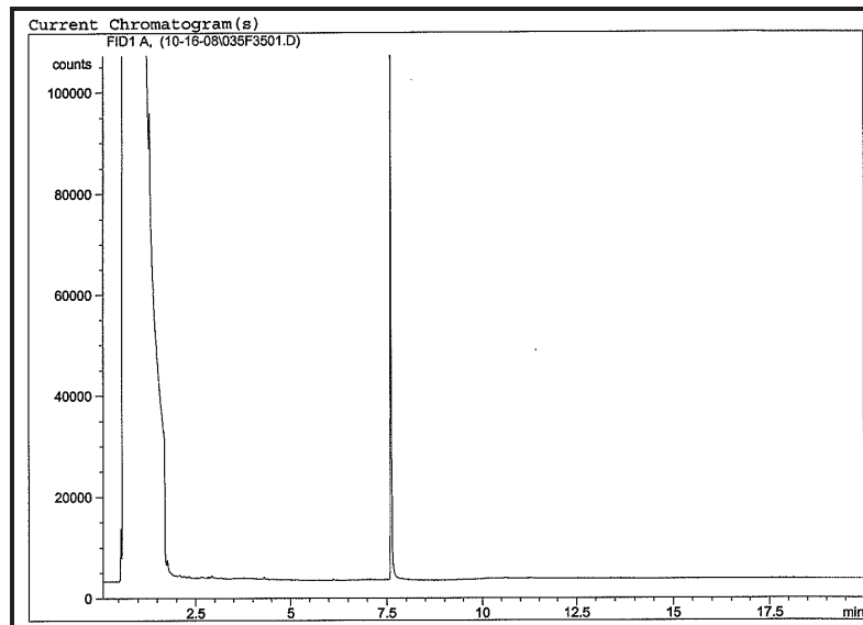
Chromatogram of sediment core JP-4 (185-190 cm).
