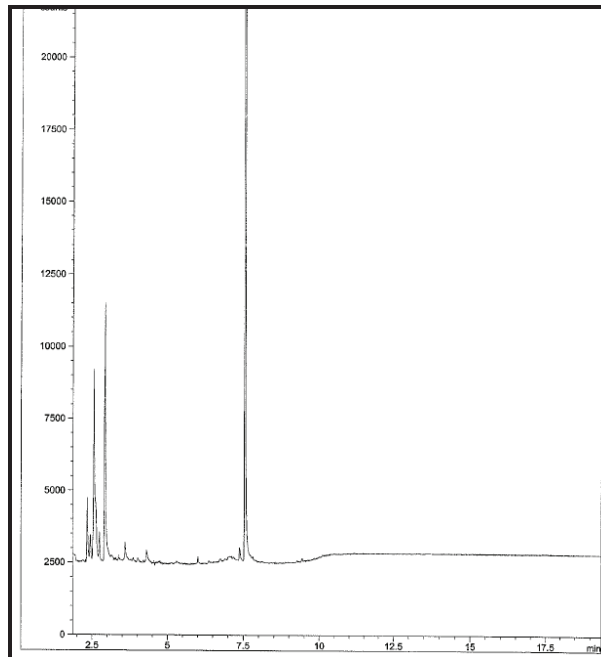
Chromatogram for sediment core BP-59 (186-191 cm).
