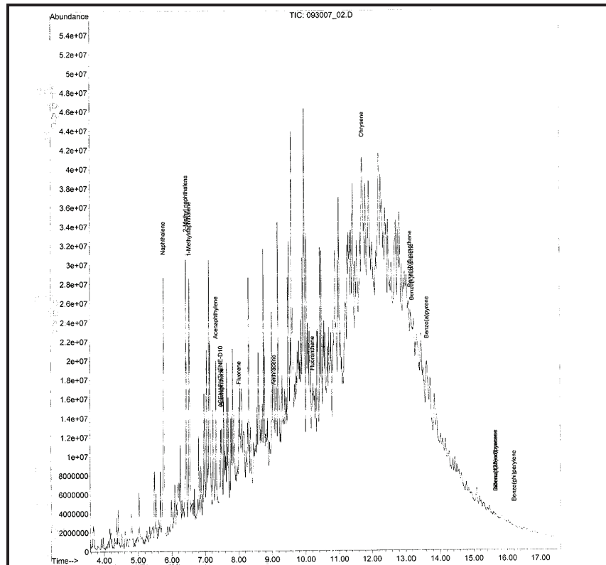
Chromatogram for the Bouchard 155 sample.
