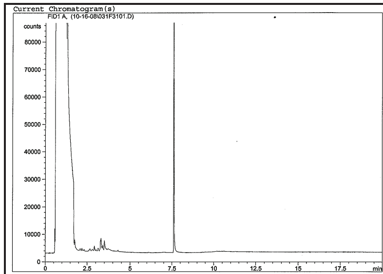
Chromatograph of sediment core JP-3 (85-90 cm).
