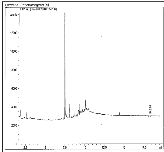
Chromatogram for sediment core BP-40 (109-119 cm).
