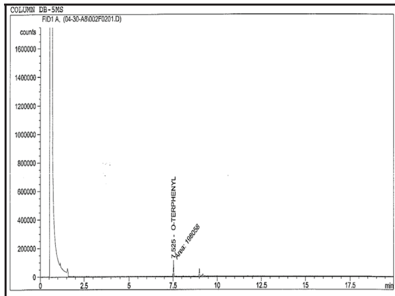
Chromatogram for sediment core BP-83 (70-75 cm).
