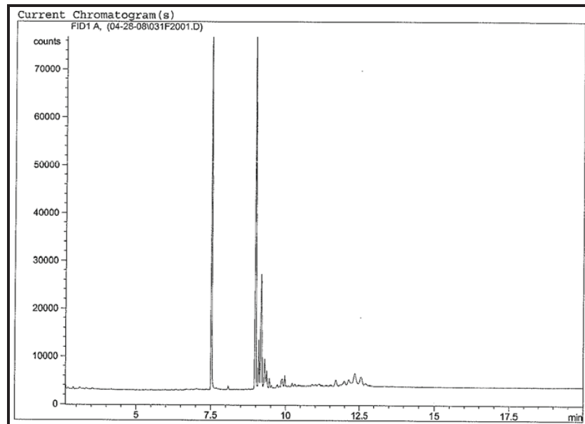
Chromatogram for sediment core BP-3 (256-261 cm).
