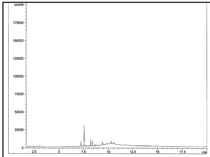
Chromatogram for sediment core BP-86 (246-249 cm).
