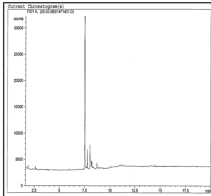
Chromatogram of sediment core BP-1 (239-244 cm).
