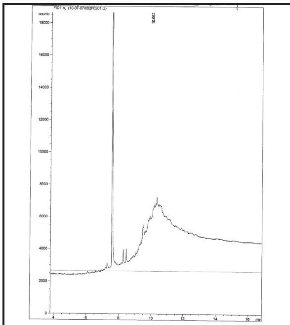
Chromatogram for sediment core BP-57 (229-234 cm).
