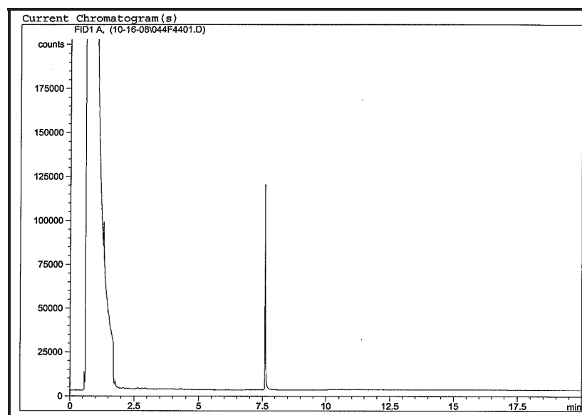
Chromatogram of sediment core JP-15 (240-245 cm).
