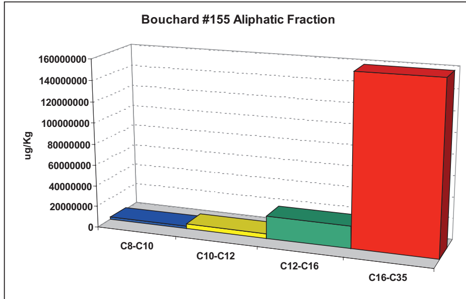
Figure 9: Bouchard 155 reference sample aliphatic concentration.
