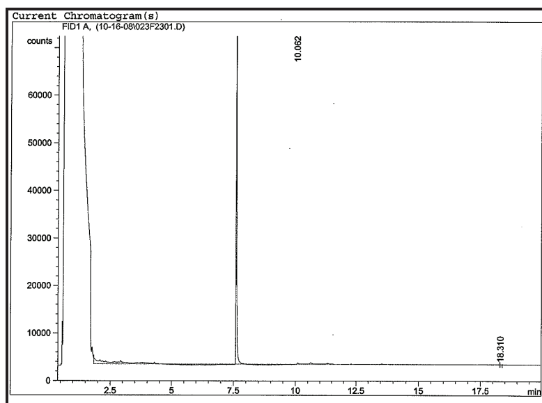
Chromatograph of sediment core JP-13 (65-70 cm).
