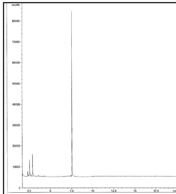
Chromatogram for sediment core BP-91 (238-243 cm).
