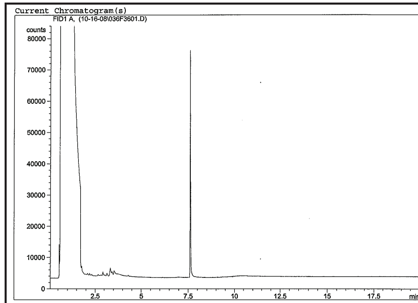
Chromatograph of sediment core JP-5 (160-165 cm).
