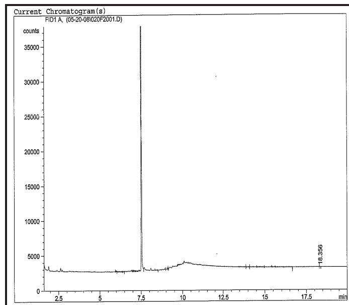
Chromatogram for sediment core BP-45 (189-194 cm).
