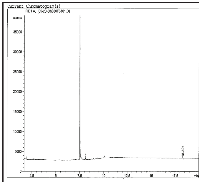
Chromatogram for sediment core BP-31 (183-188 cm).
