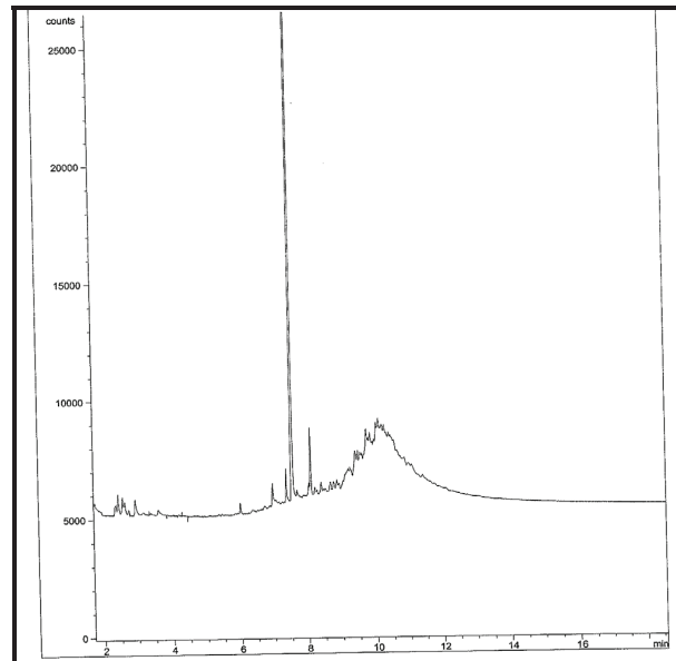
Chromatogram for sediment core BP-24 (293-294 cm).
