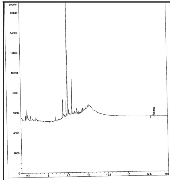
Chromatogram for sediment core BP-31 (265-271 cm).
