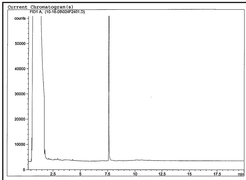
Chromatogram of sediment core JP-11-2 (148-153 cm).
