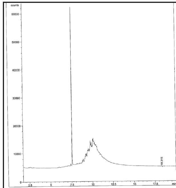
Chromatogram for sediment core BP-39 (231-238 cm).
