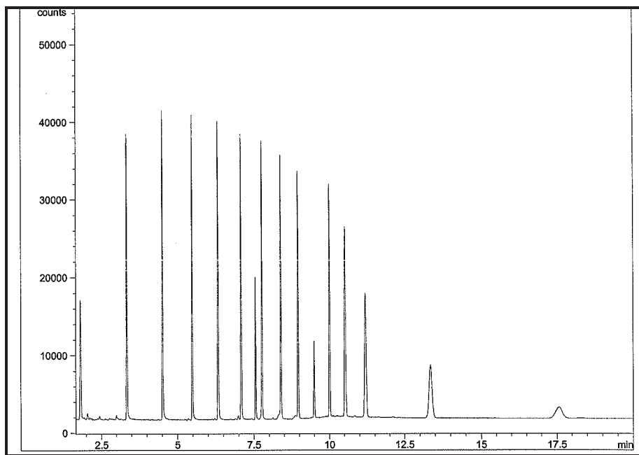
Chromatogram
