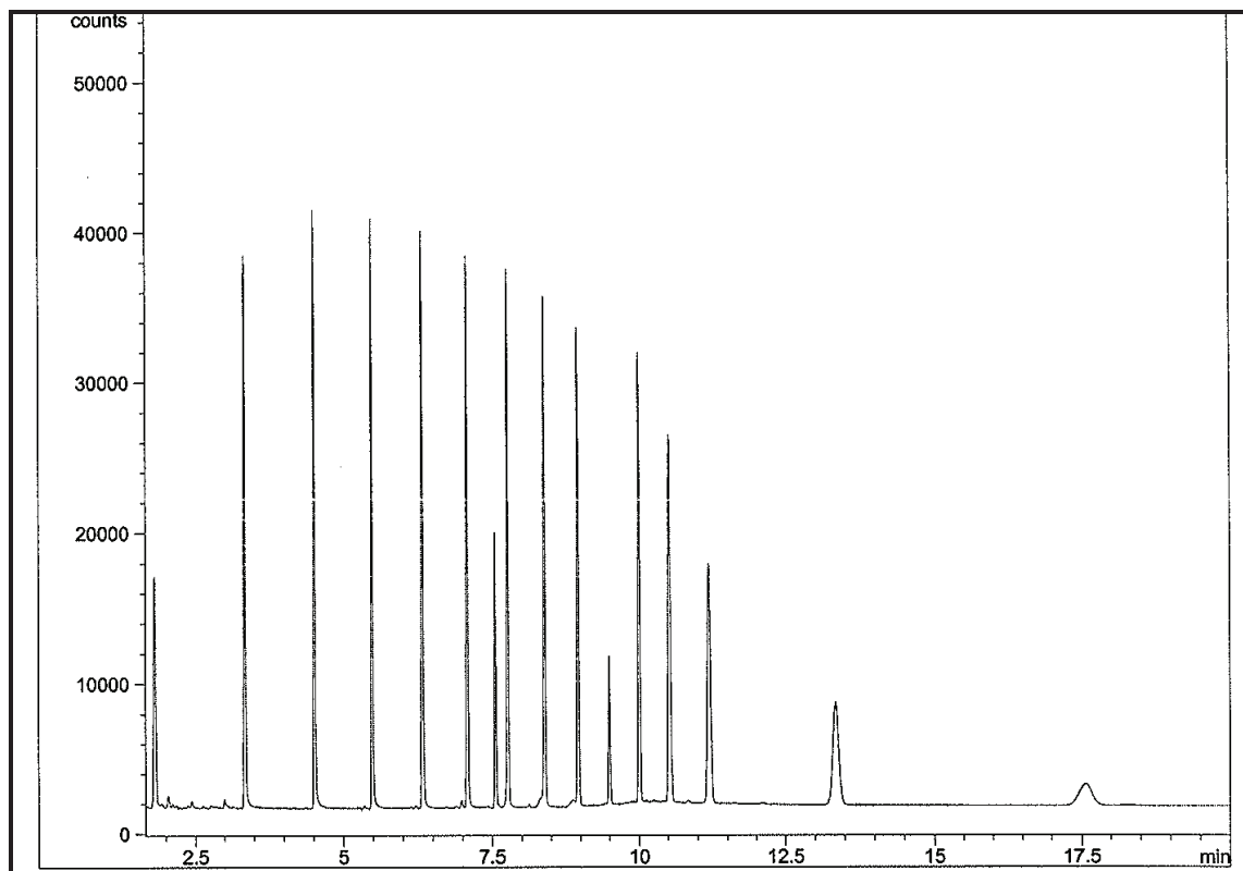
Figure 16: Instrument calibration chromatogram for GC/MS.
