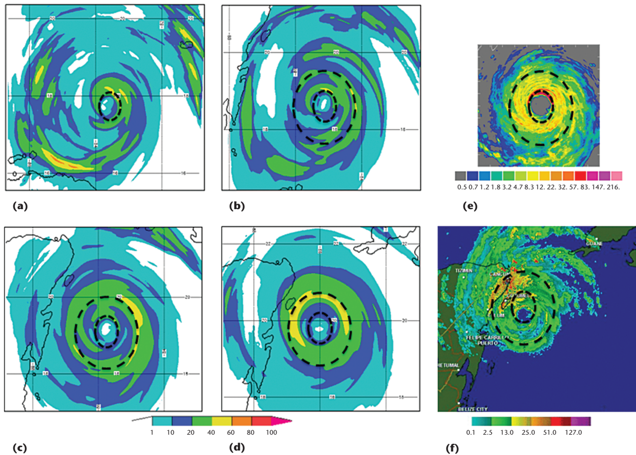
Figure 3. HRRF's forecast for Hurricane Wilma eyewall replacement compared to radar-estimated precipitation rate. The HRRF 9/3-km resolution forecast was initiated at 1200 UTC 19 October 2005. The HRRF precipitation rate (mm/hr) at (a) 12 hours, (b) 24 hours, (c) 30 hours, and (d) 36 hours into the forecast. Radar-estimated precipitation rate (mm/hr) from the NOAA P3 aircraft radar observation and Mexico National Meteorological Service (e) at 1414 UTC 20 October 2005 and (f) 1156 UTC 21 October 2005 (see ( http://www.srh.noaa.gov/tae/?n=research-zrpaper )). Dashed circles indicate the approximate eyewall positions before and after the replacement process.
