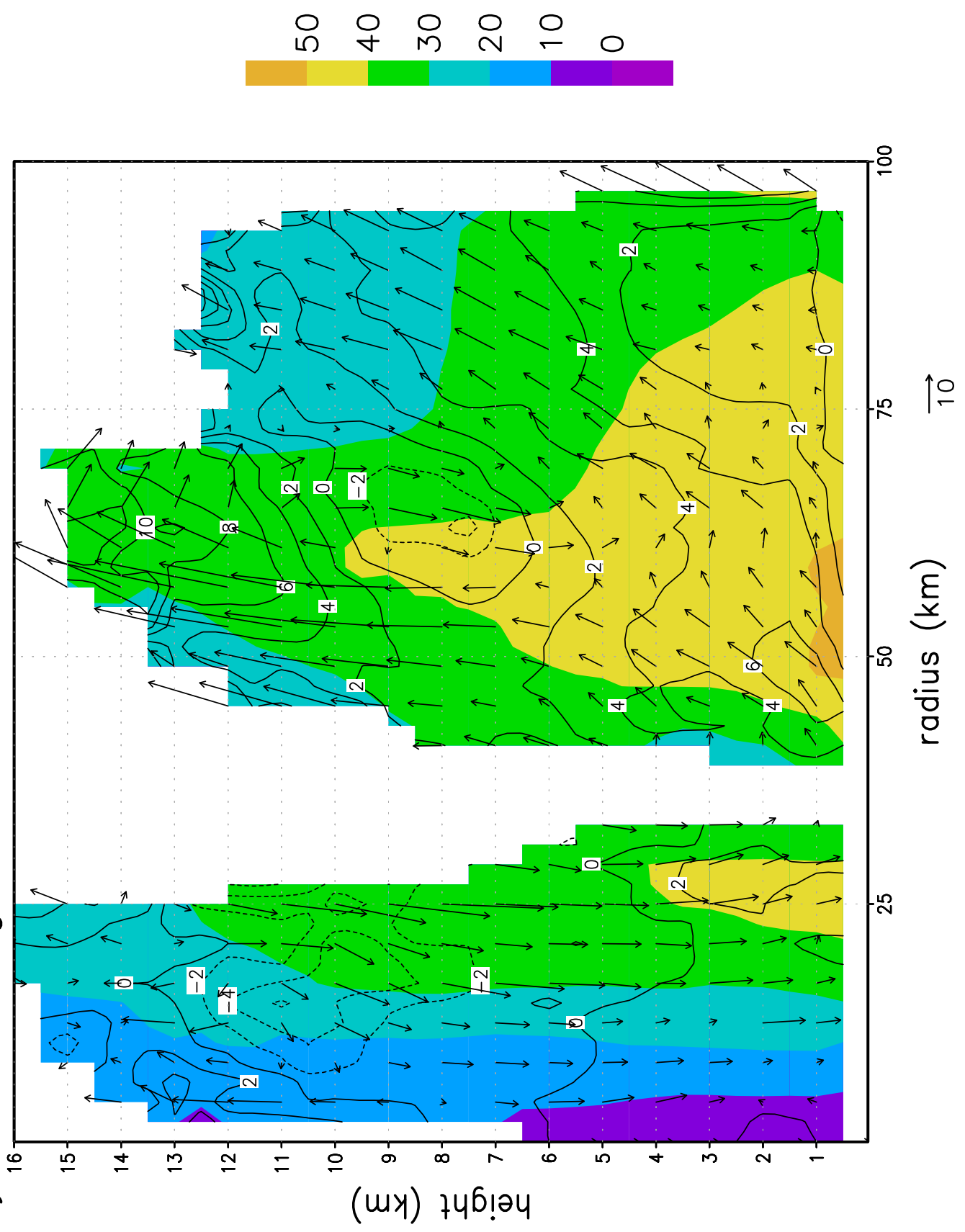
Axisymmetric tangential and radial wind at 20:08Z27AUG2005
