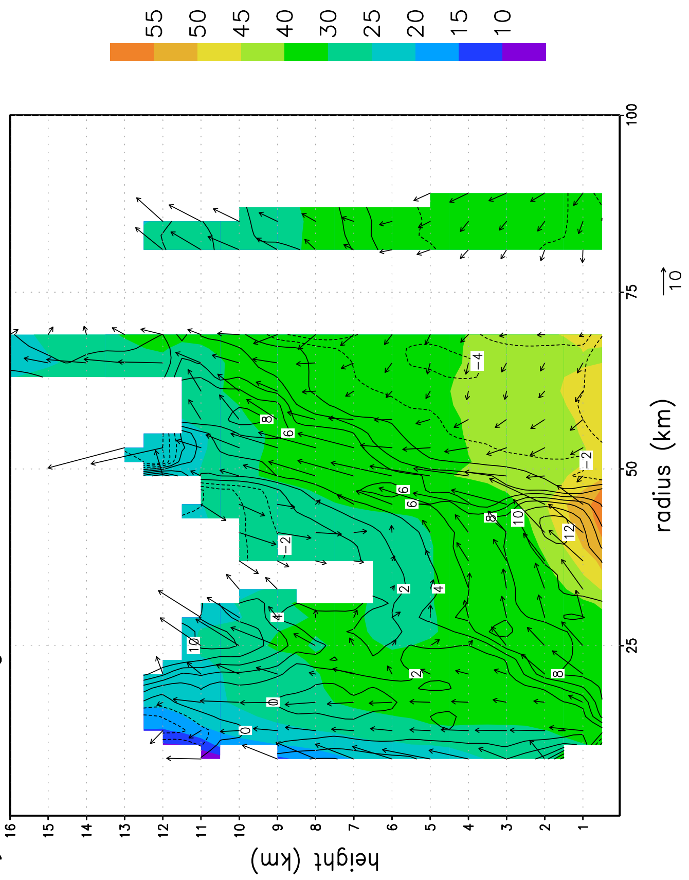
Axisymmetric tangential and radial wind at 16:51Z27AUG2005
