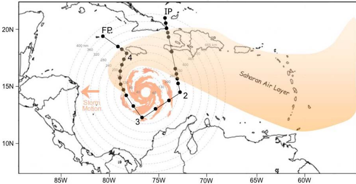
Figure GEN-4. Sample G-IV flight track for a TC embedded in the SAL for most or all of its lifecycle.
