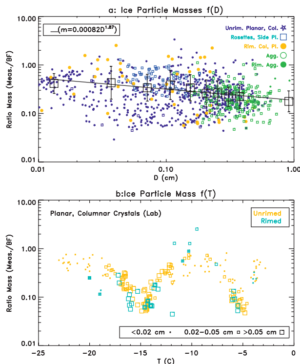
FIG. 1. Ratio of particle mass as derived from the BF95 relationship for a given particle size divided by the mass as measured. (a) Data for a number of particle types from sources given in the text. (b) Data from Takahashi and Fukuta (1988) and Takahashi et al. (1991) from laboratory experiments for unrimed and rimed ice particles grown at constant temperatures.
