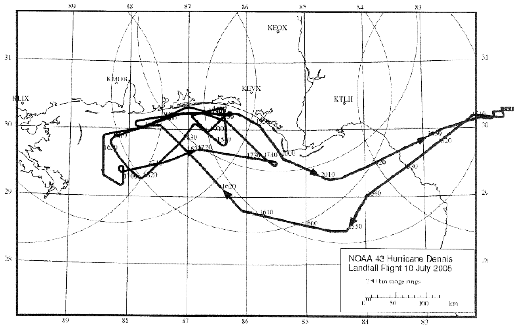
Fig. 1: Flight track of NOAA43.
