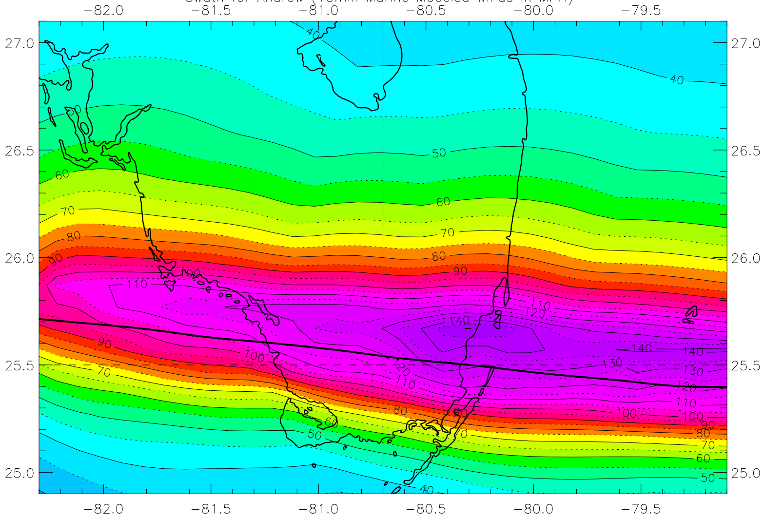
Swath for Andrew (10min Marine Modeled winds in MPH)
