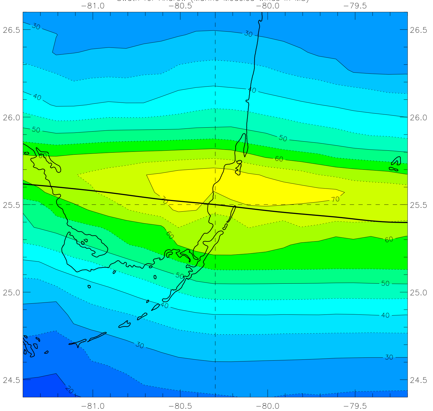
Swath for Andrew (Marine Modeled winds in MS)
