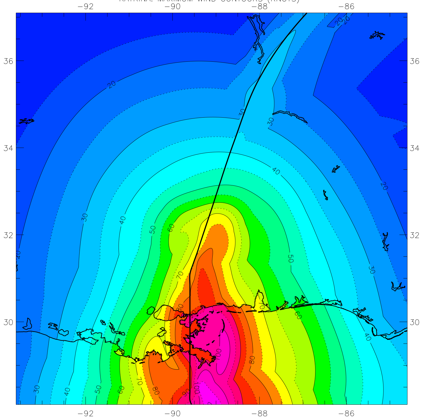
KATRINA: MAXIMUM WIND CONTOURS (KNOTS)
