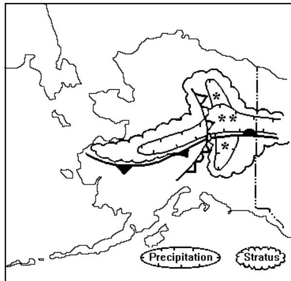
Figure 1-34. Occluded Front and Location of Snow. The heaviest snow usually occurs just on the cold-air side of the arctic front near the occluded front or the trough.
