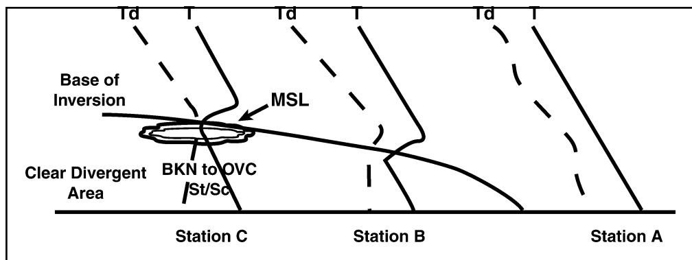
Figure 2-22. Typical Cold-Air Stratocumulus/Stratus Scenerio. Station A is still in warm air, and clouds are dependent upon the moisture and stability of the warm air mass. Station B is in the cold air, but the inversion is below the MCL, hence no stratocumulus is present. At Station C, the frontal inversion is above the calculated MCL and broken to overcast stratocumulus results. Note: ceilings formed purely from turbulent mixing generally have bases above 1,500 feet.
