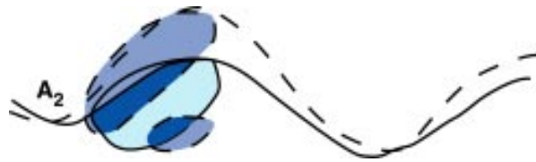
Figure 2-8. Rule A2. Cirrus spreads northward and diminishes in the south slightly. Cirrus becomes denser.
