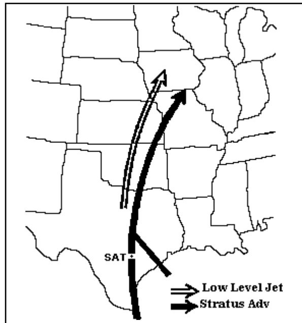
Figure 2-28. Type 2 Gulf Stratus Advection. This type of stratus advects into the central plains and remains until the air mass changes.
