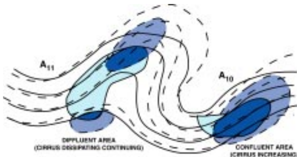
Figure 2-17. Rule A11. Cirrus dissipates in developing diffluent area, and the dissipating cirrus spreads upstream.
