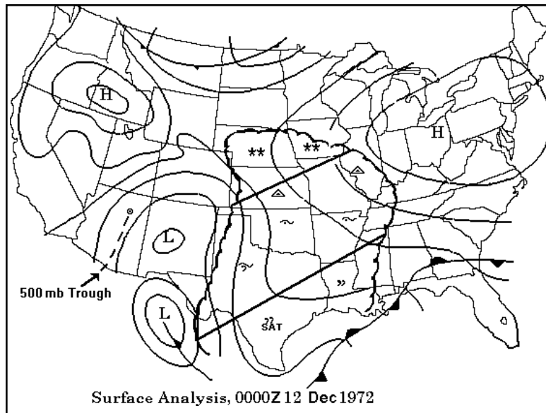
Figure 2-24. Stationary Front 24 Hours Later. Overrunning stratus and precipitation spread northward from Texas into the upper Midwest producing a variety of precipitation types
