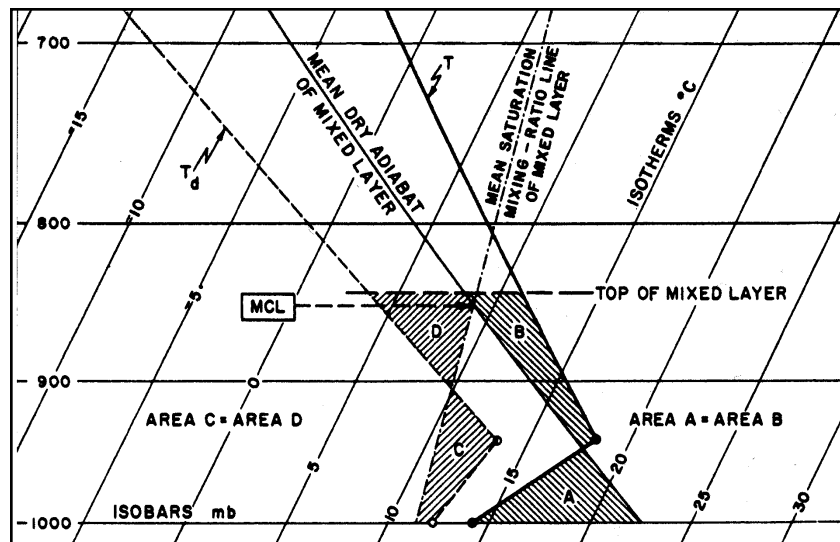
Figure 2-3. MCL Calculations. The MCL provides a good approximation of stratus or stratocumulus base heights
