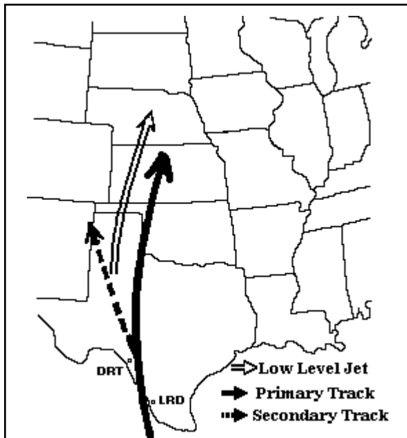
Figure 2-27. Type 1 Gulf Stratus Advection. Moist air enters coastal Mexico and tracks north-west, then north into Nebraska.
