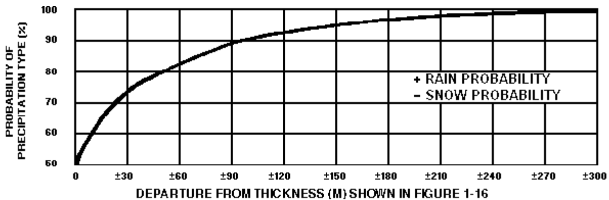
Figure 1-17. Probability of Precipitation being Frozen Versus Liquid.
