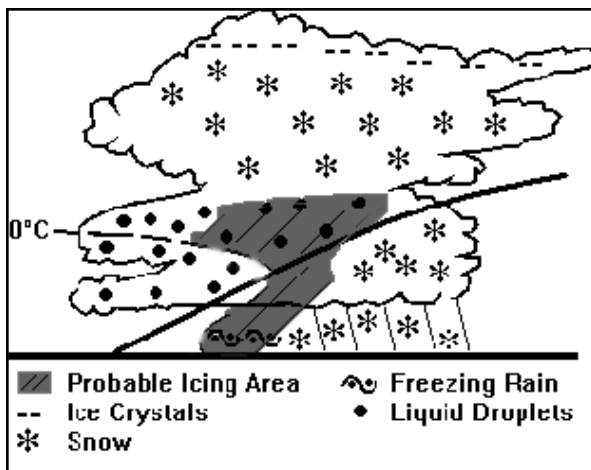
Figure 2-64. Icing with a Warm Front. Icing occurs up to 300 miles ahead of the warm frontal surface position.
