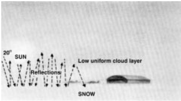
Figure 1-1. Whiteout Conditions. Occur when light reflected back and forth between snow- or ice-covered ground and low stratus clouds
