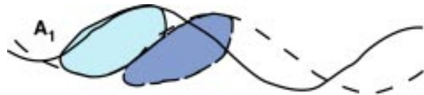
Figure 2-7. Rule A1. Cirrus generally spreads eastward.
