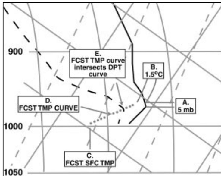
Figure 1-10. Skew-T Method for Estimating the Top of Radiation Fog. Uses data at sunrise to calculate the dissipation temperature.
