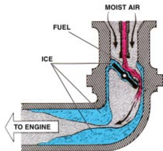
Figure 2-67. Carburetor Icing.
