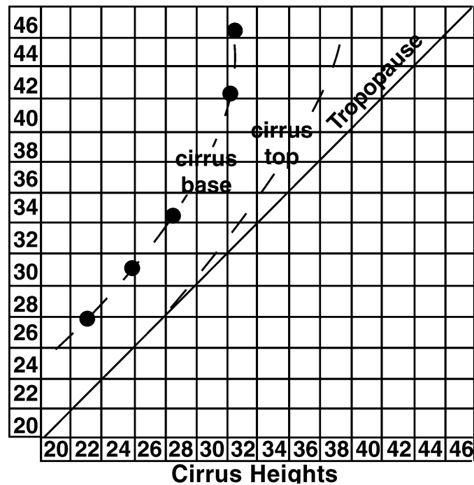
Figure 2-20. Tropopause Method of Forecasting Cirrus. Find the current tropopause height and read across to see the average cirrus base and top.
