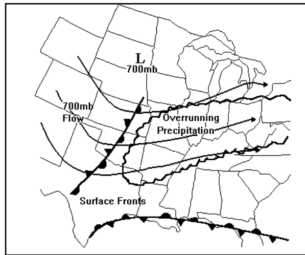
Figure 1-15. Overrunning Precipitation Associated with a Stationary Front. This type of overrunning occurs well to the north of the surface frontal zone.
