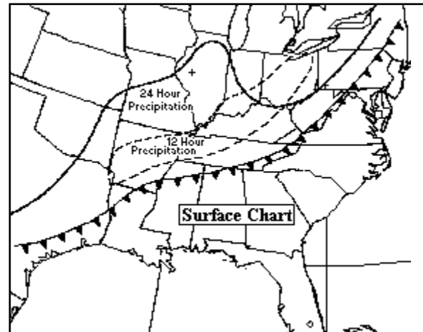
Figure 1-12. Widespread Precipitation Scenario. The resulting spread of precipitation 24 hours after the system shown in Figure 1-13.
