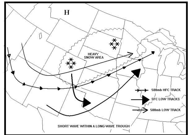
Figure 1-31. Heavy Snow Track Pattern 2. the alignment and movement of the surface low, the 500-mb low, and the 500-mb height fall center tracks are shown, as well as the heavy snow area.
