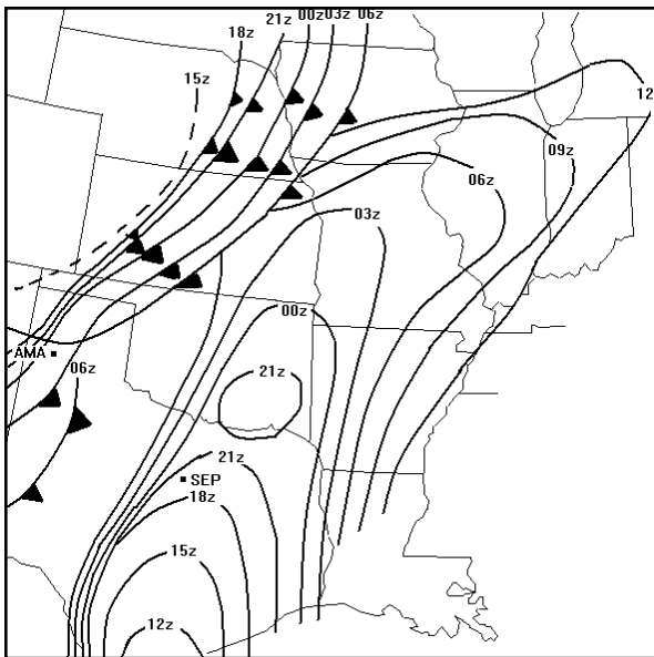
Figure 2-25. Advection of Gulf Stratus with a LLJ. A strong jet can advect significant amounts of gulf moisture from Texas to the Great Lakes within 24 hours.
