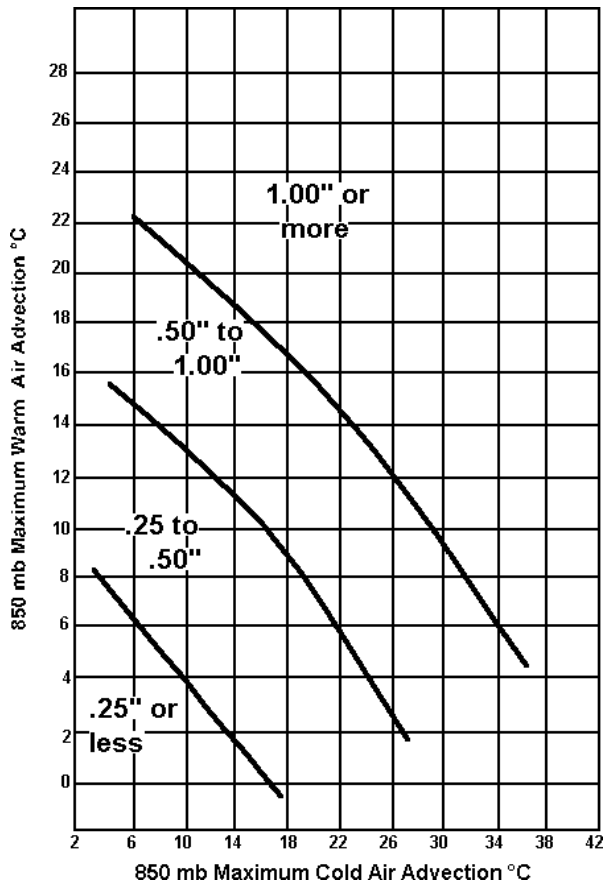
Figure 1-26b. Maximum Precipitation, 850 mb Trough East of 100° Meridian. Figure shows 12- to 24-hour maximum precipitation.
