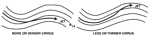
Figure 2-19. Rule A14. Cirrus is more likely to exist if the jet crosses contours toward higher heights.
