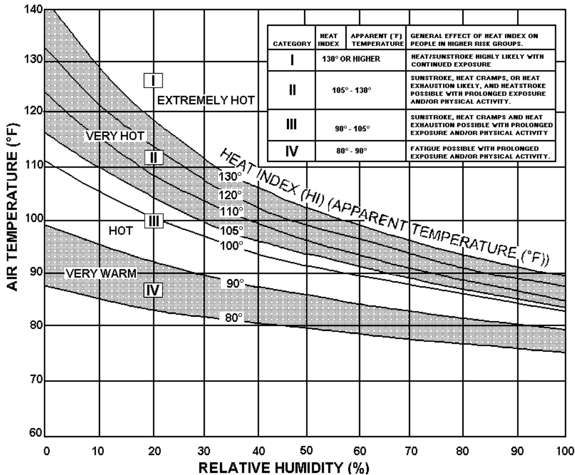
Figure 1-52. Heat Index. Enter this temperature/humidity nomogram with observed or forecast data to predict apparent temperature and effect on people.
