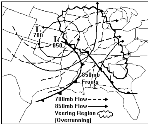
Figure 1-14. Overrunning Associated with a Typical Cyclone. This pattern occurs with an active warm front to the north of a surface cyclone
