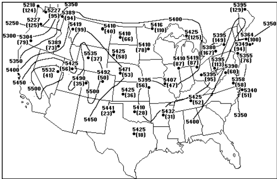
Figure 1-16. Equal Probability of Liquid or Frozen Precipitation. Based upon 1000- to 500-mb thickness (climatology).
