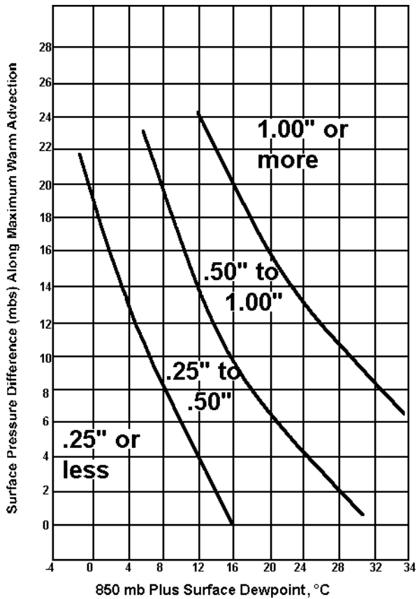
Figure 1-26a. Maximum Precipitation, 850 mb Trough East of 100° Meridian. Figure shows 0- to 12-hour maximum precipitation.
