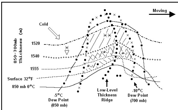
Figure 1-18. Method 2. Plotting indicated parameters on one map shows where to expect different precipitation types.
