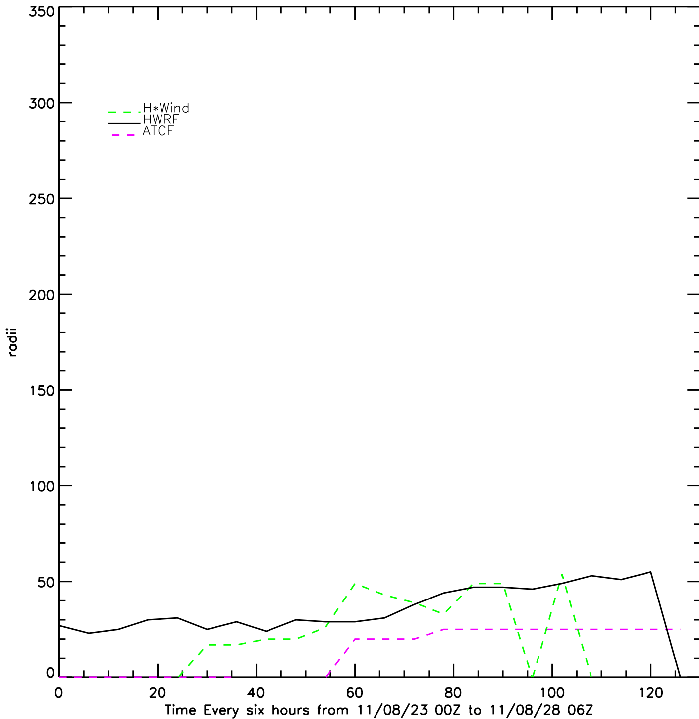
Irene: SW wind radii 33
