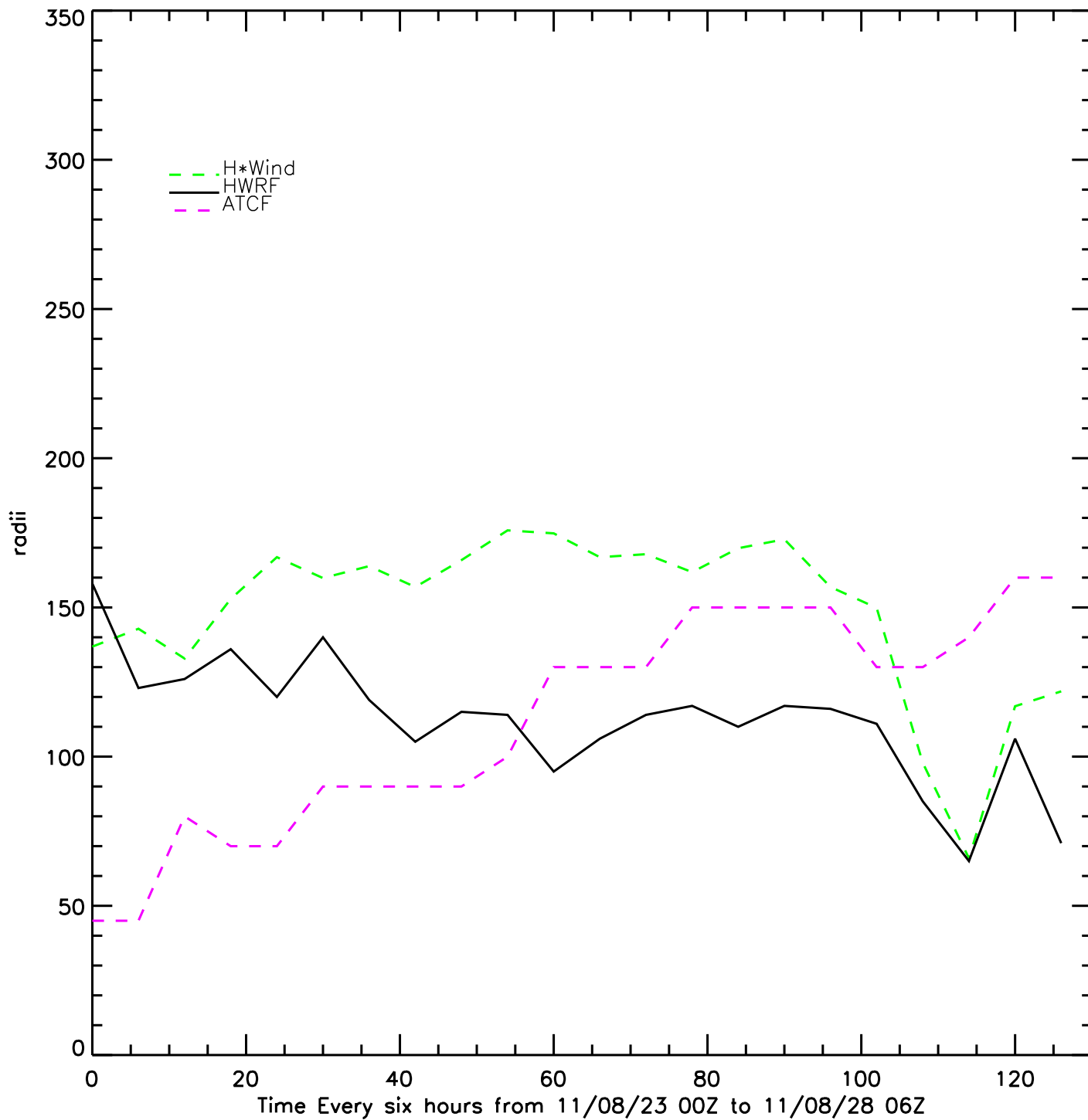
Irene: NW wind radii 18
