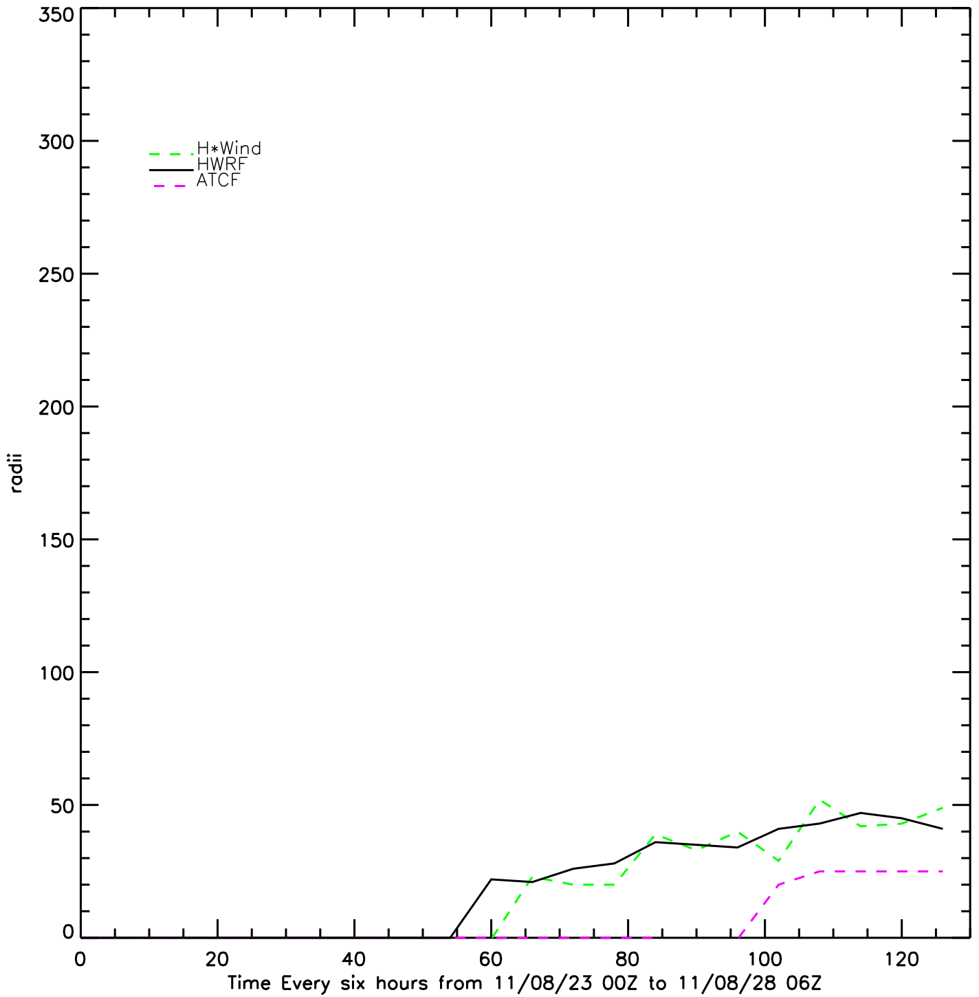
Earl: SW wind radii 33
