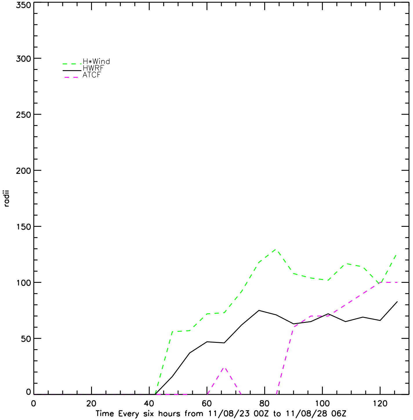
Earl: SE wind radii 26
