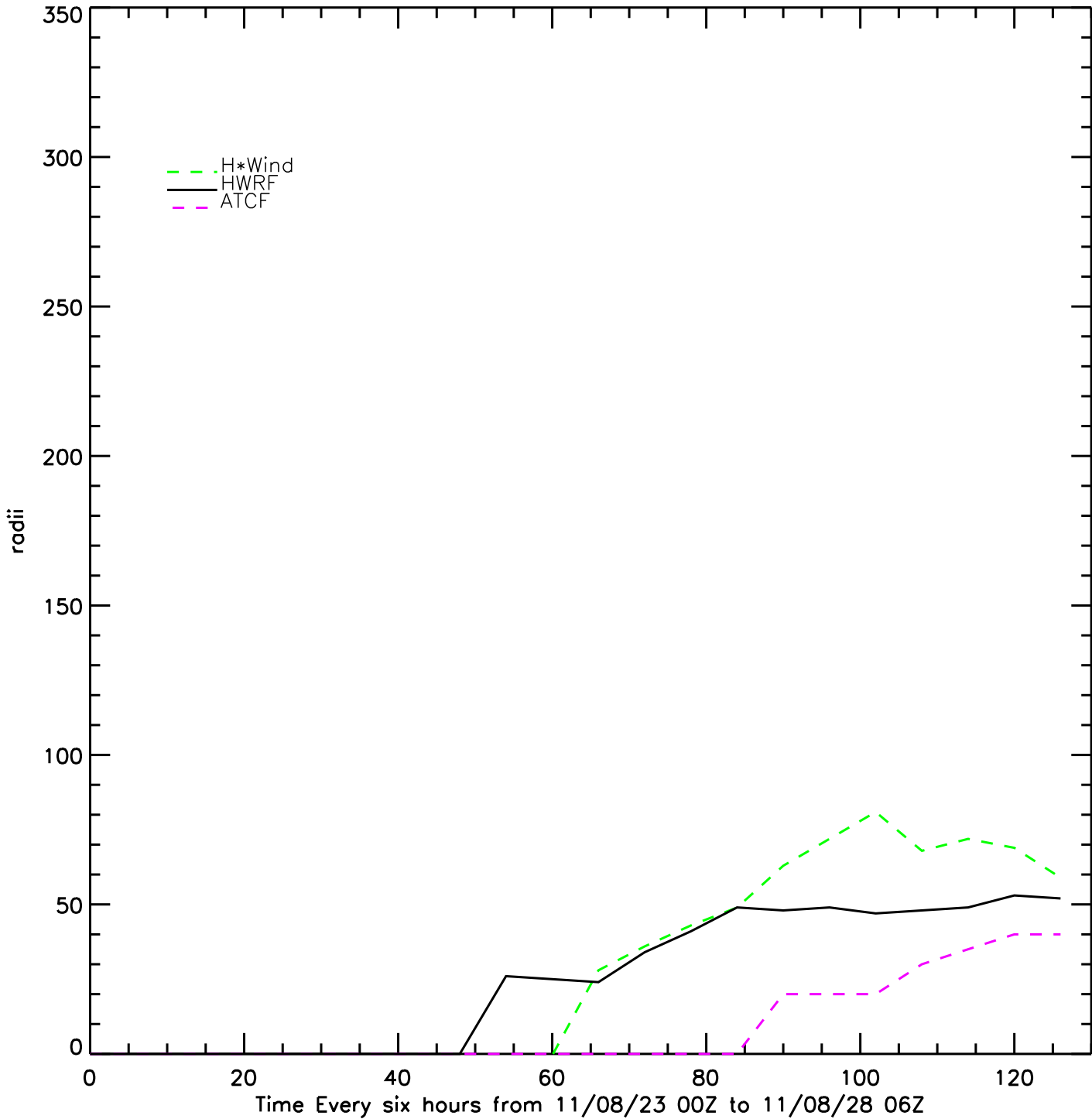
Earl: NW wind radii 33
