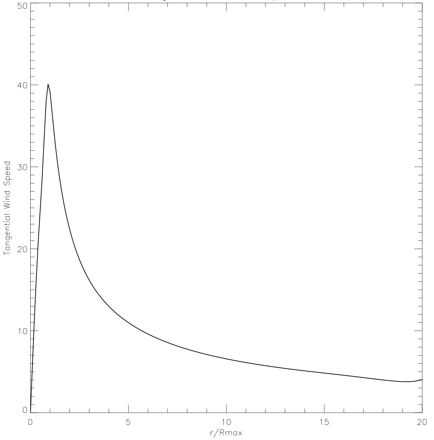
Tangential Wind versus r/R_{max}
