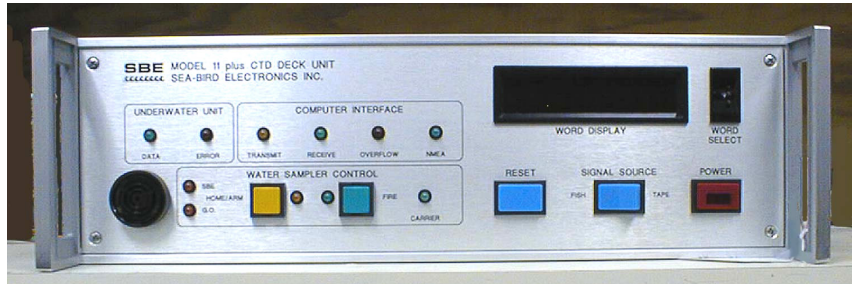
Front Panel – switches and LEDs
