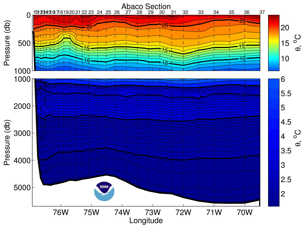
Figure 30: Potential Temperature (°C) section for the Abaco Section. Dashed vertical lines are the CTD station locations.
