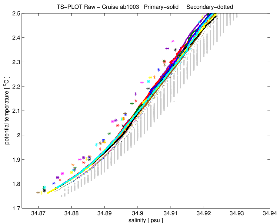
Figure 7: T-S plot of the original salinity samples compared with the sensors and the historical data.
