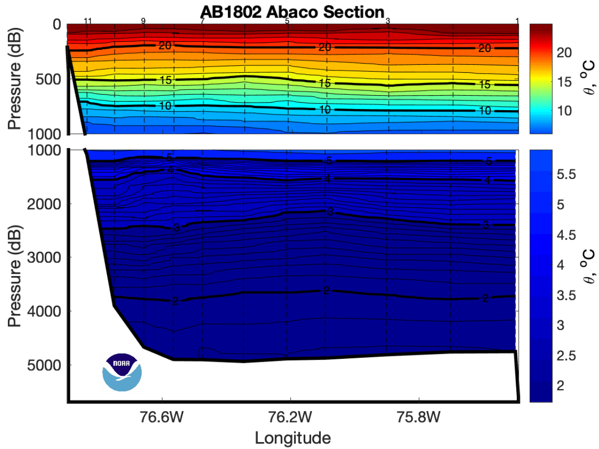
Figure 31: Potential Temperature (°C) section for the Abaco Section. Dashed vertical lines are the CTD station locations.
