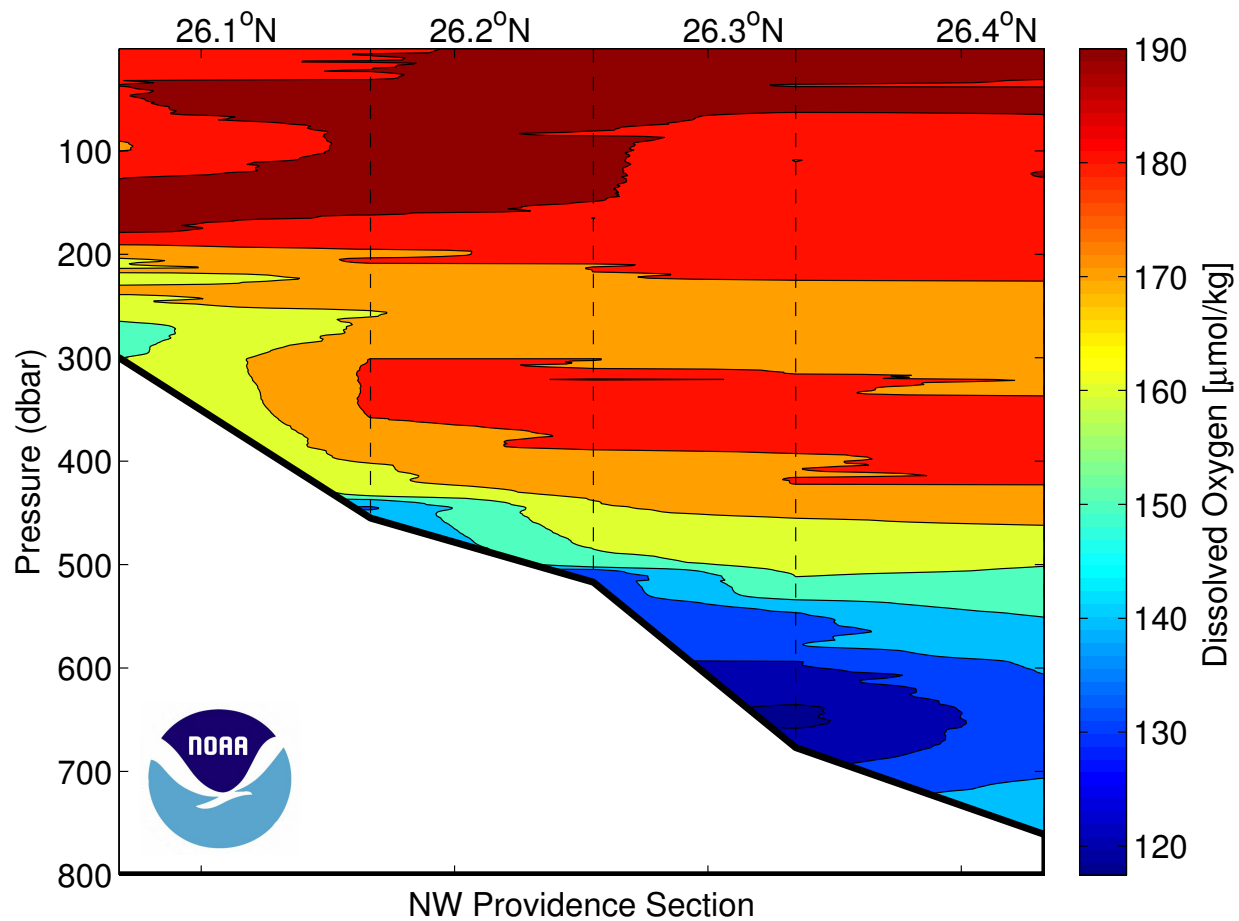
Figure 41: Dissolved Oxygen ( \mu\text{mol/kg} ) section for the Northwest Providence Channel section. Dashed vertical lines are the CTD station locations.
