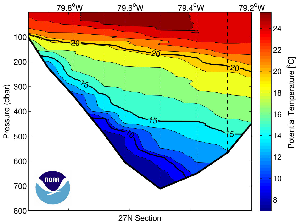
Figure 31: Potential Temperature (°C) section for the Florida Current North section. Dashed vertical lines are the CTD station locations.
