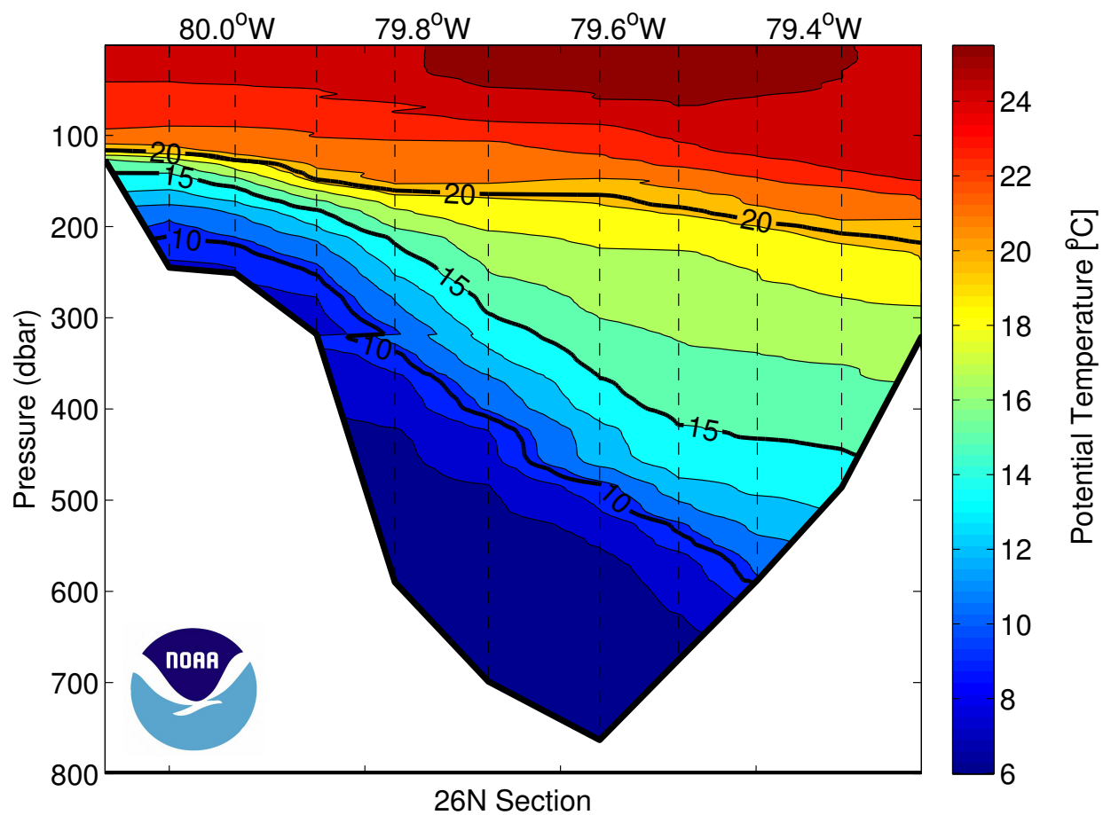
Figure 35: Potential Temperature ( ^{\circ}\text{C} ) section for the Florida Current South section. Contour intervals are 1^{\circ}\text{C} . Dashed vertical lines are the CTD station locations.
