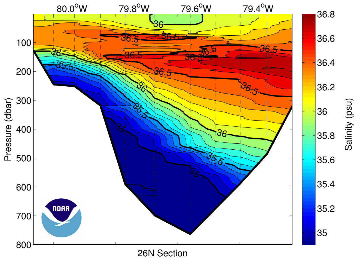
Figure 36: Salinity (PSS 78) section for the Florida Current South section. Contour intervals are 0.1. Dashed vertical lines are the CTD station locations.
