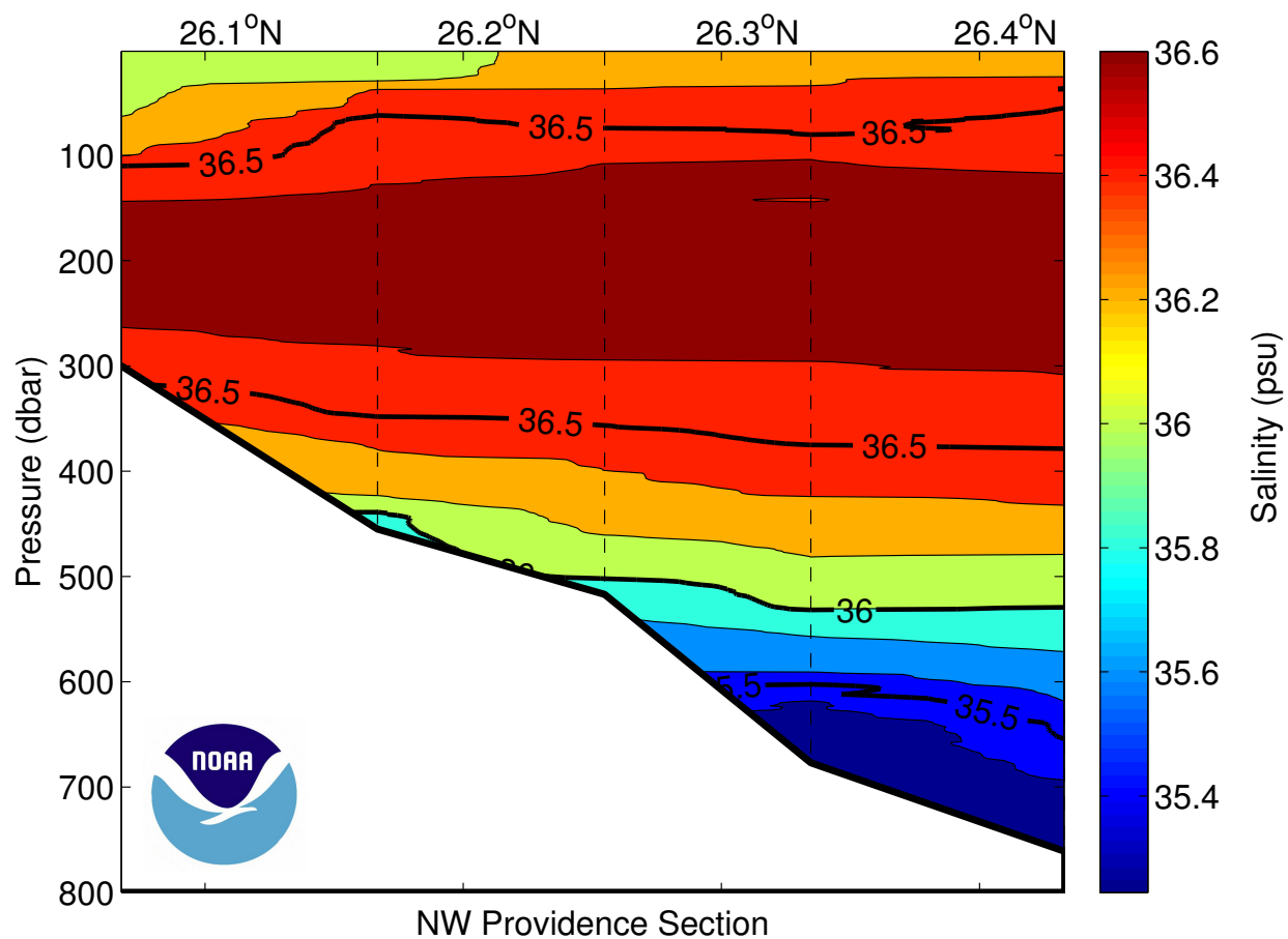
Figure 40: Salinity (PSS 78) section for the Northwest Providence Channel section. Dashed vertical lines are the CTD station locations.
