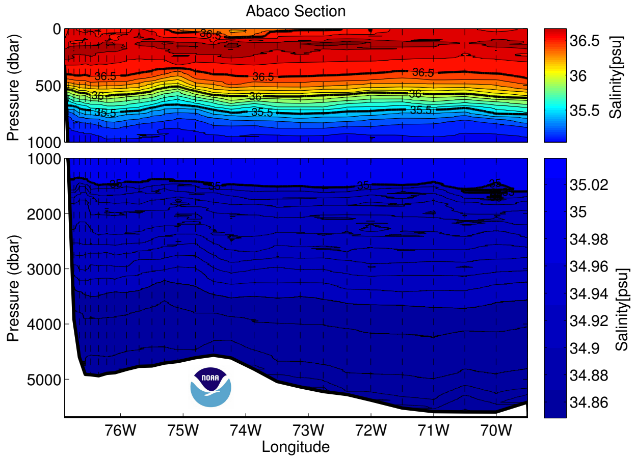
Figure 28: Salinity (PSS 78) section for the Abaco section. Dashed vertical lines are the CTD station locations.
