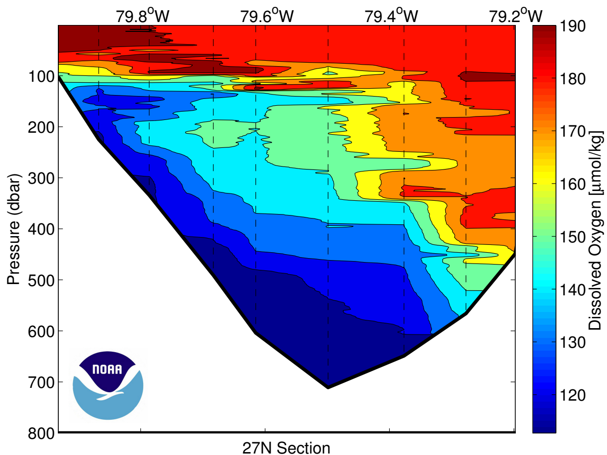
Figure 33: Dissolved Oxygen ( \mu\text{mol/kg} ) section for the Florida Current North section. Dashed vertical lines are the CTD station locations.
