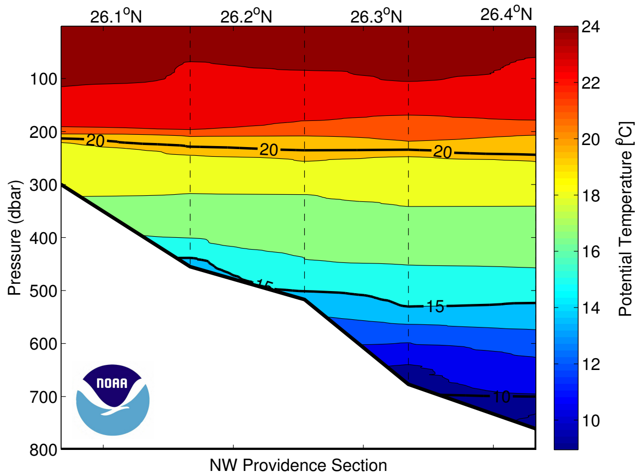
Figure 39: Potential Temperature ( ^{\circ}\text{C} ) section for the Northwest Providence Channel section. Dashed vertical lines are the CTD station locations.
