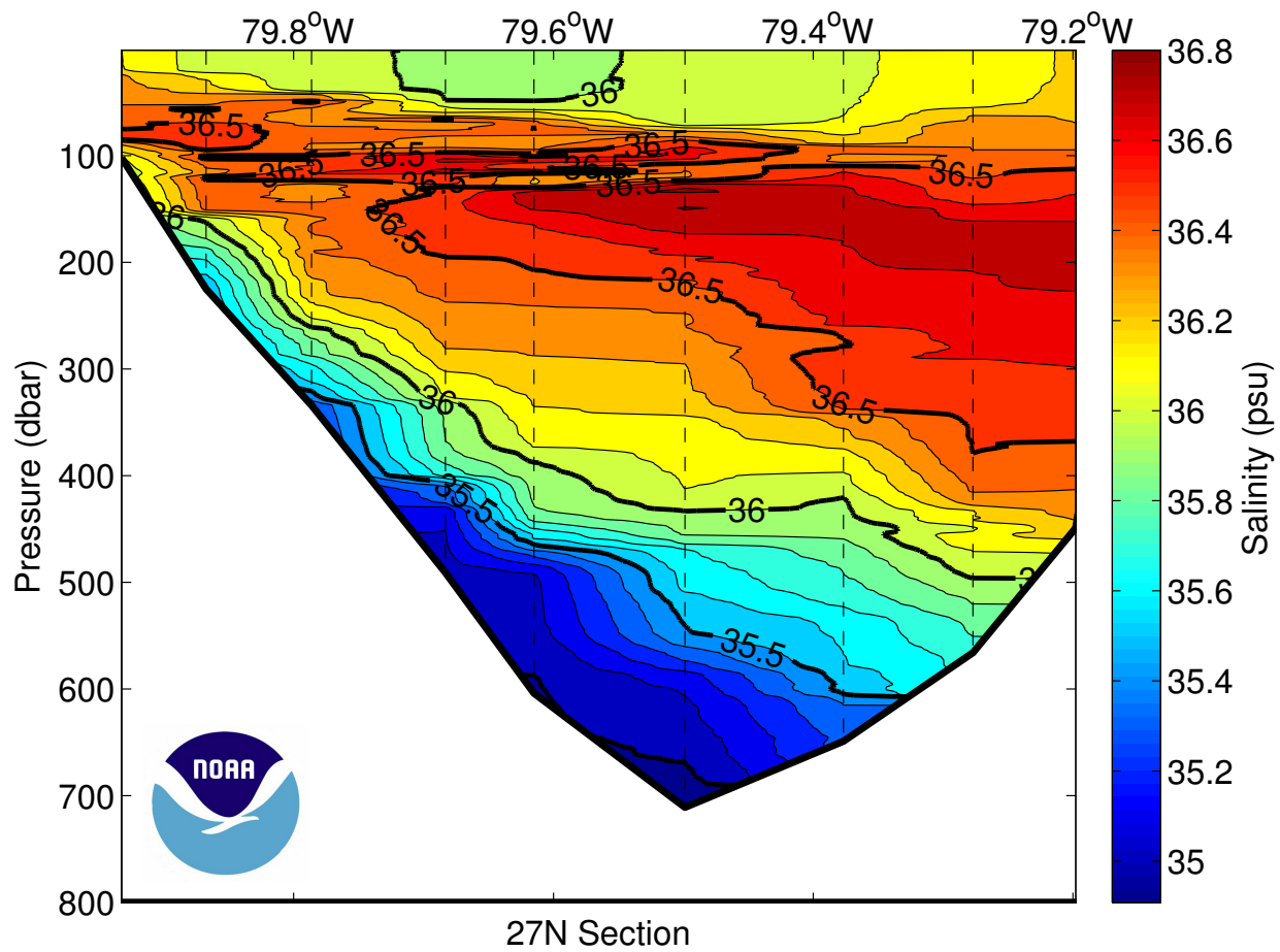
Figure 32: Salinity (PSS 78) section for the Florida Current North section. Dashed vertical lines are the CTD station locations.
