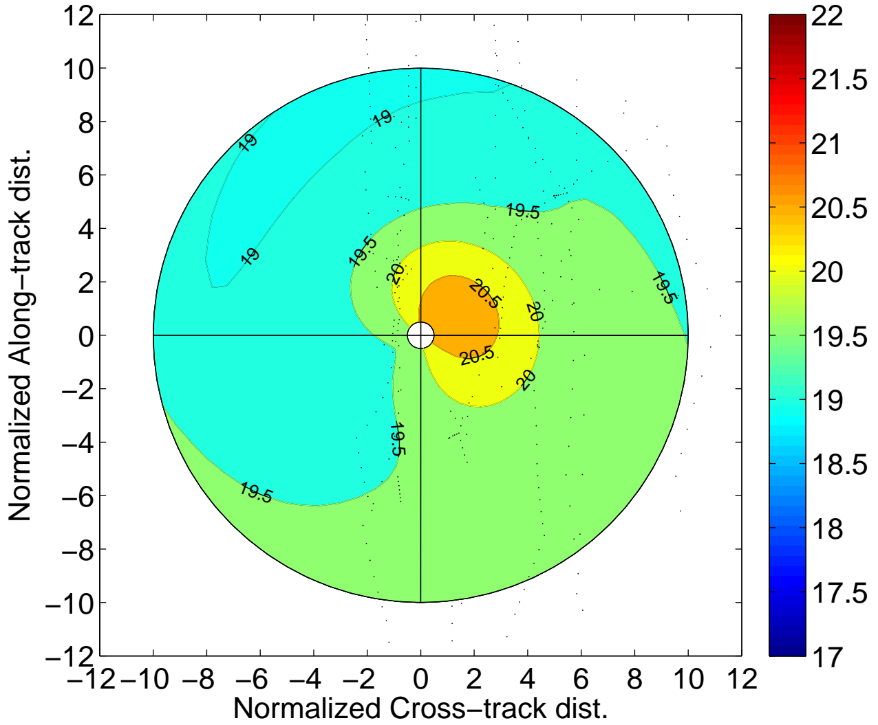
Westward q_{10} (g/kg)
