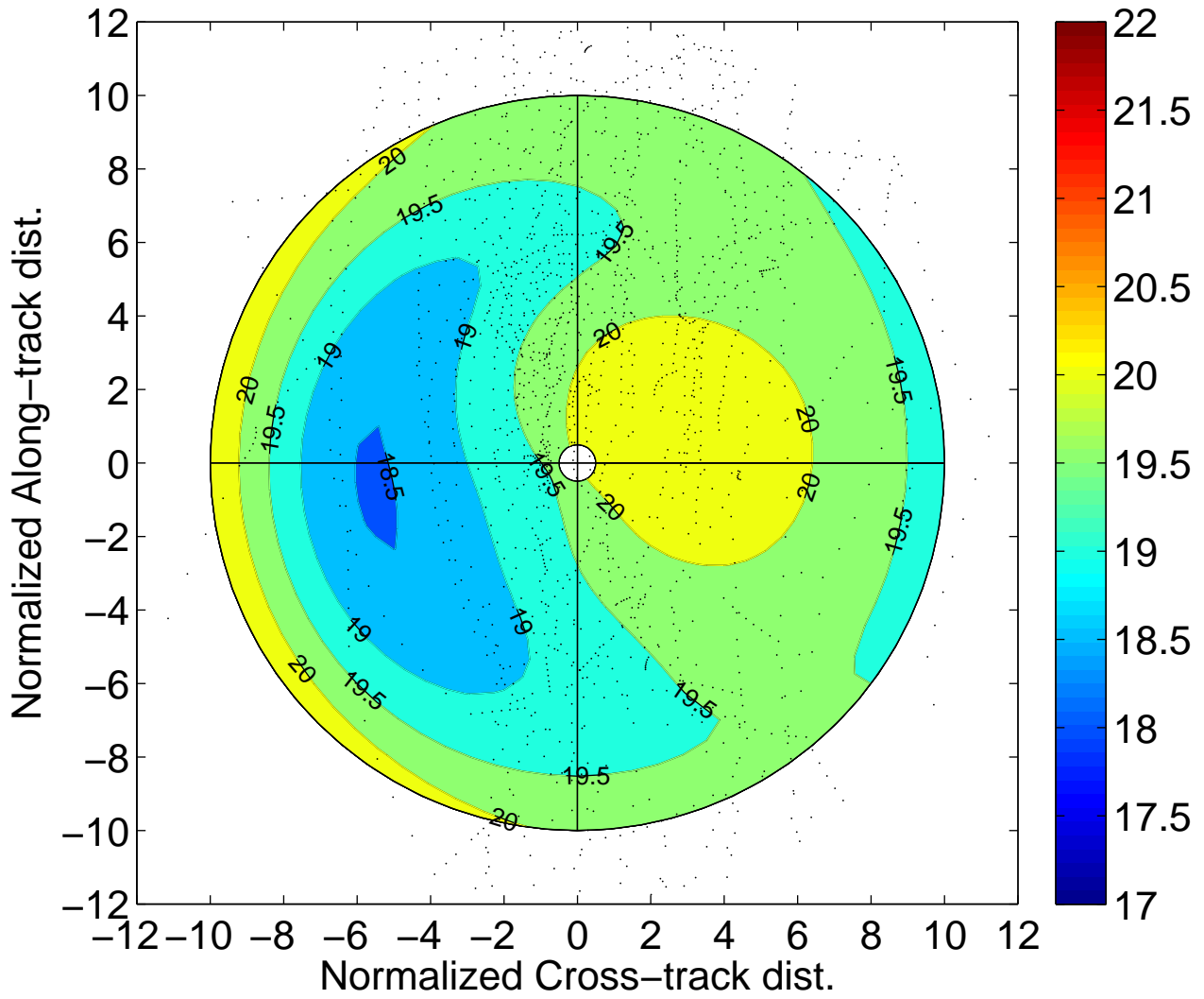
All Storms q_{10} (g/kg)
