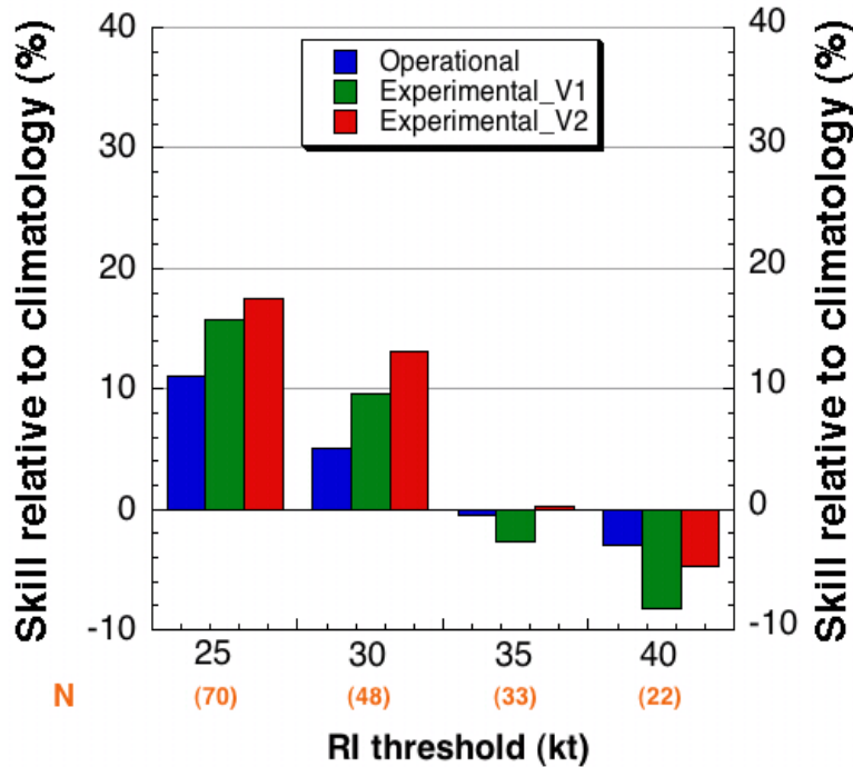
Fig. 6. Skill of the new Experimental Atlantic RII for both the original (Experimental_V1) and the newest (Experimental_V2) formulation for the 2008-2010 independent re-run forecasts (N=503). Also shown for comparison is the skill of the operational version of the RII for those same forecasts. The number of RI cases for each RI threshold is provided in orange.
