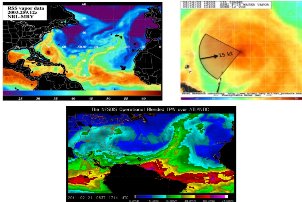
Fig. 2. Total precipitable water (TPW) analysis at 9/16/03 at 12 UTC courtesy NRL (top left panel). A close-up view showing the area over which the TPW predictor is computed is also depicted for Hurricane Isabel located several hundred kilometers east of Florida at this time (top right panel). Finally, an example of the new blended NESDIS operational TPW analysis product that is currently used in real-time is also provided (bottom panel).
