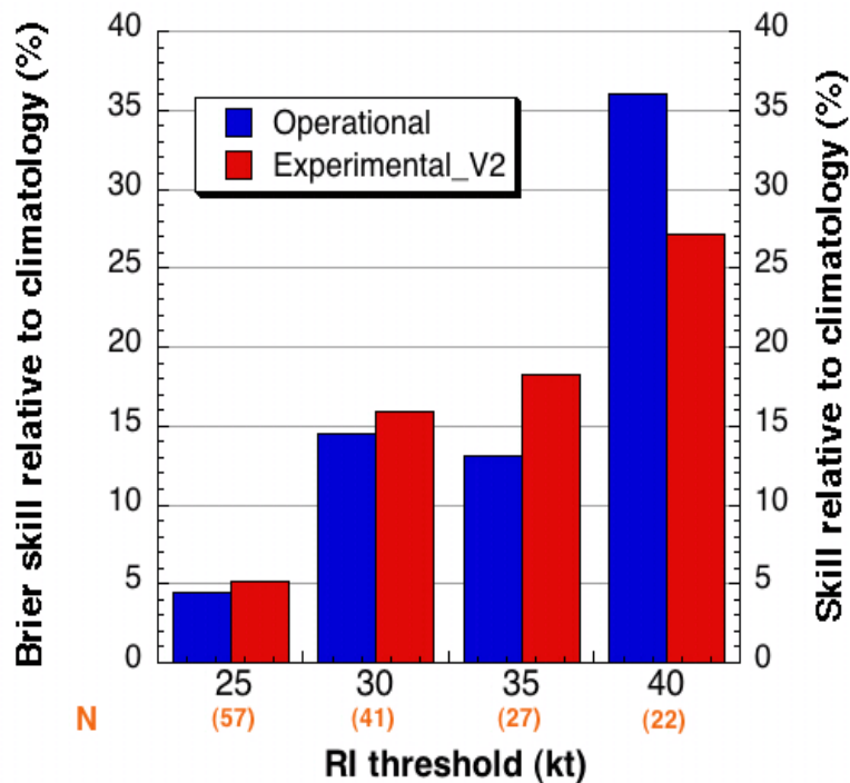
Fig. 7. Skill of the operational and experimental_V2 version of the eastern North Pacific RII for the independent 2008-2010 re-run forecasts (N=509). Also shown for comparison is the skill of the operational version of the RII for those same forecasts. The number of RI cases for each RI threshold is also shown in orange.
