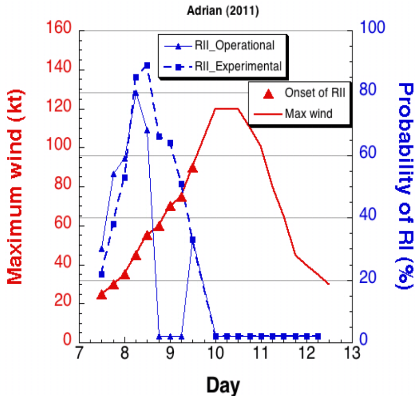
Fig 8. The probability of RI for the operational (solid blue) and new experimental (dashed blue) versions of the RII for eastern North Pacific Hurricane Adrian (2011). The NHC real-time maximum sustained wind estimates (solid red line) and the initial (T=0 h) times at which RI commenced (red triangles) are also provided.
