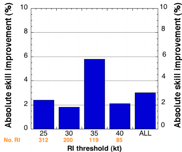
Fig. 4. Improvement of the new Atlantic Experimental RII over the current operational version for the 1995-2009 dependent sample (N=2524). The number of RI cases for each RI threshold are shown in orange along the x-axis.
