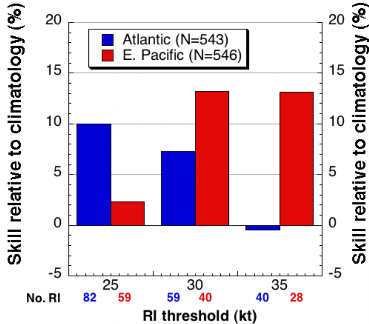
Fig. 1. The skill of the 2008-2010 operational RII forecasts. The number of RI cases for each RI threshold is also provided for both the Atlantic (blue) and eastern North Pacific (red) basins.
