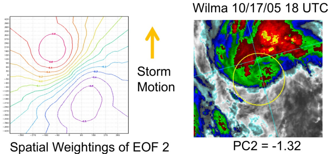
Fig. 3. Preferred pattern of PC2 (left) and an example of the corresponding GOES-IR representation for Hurricane Wilma at 18 UTC on 17 October (right). The yellow circle denotes a circle with a radius of 440 km over which the PCs were evaluated. The direction of motion is to the top center of both diagrams.
