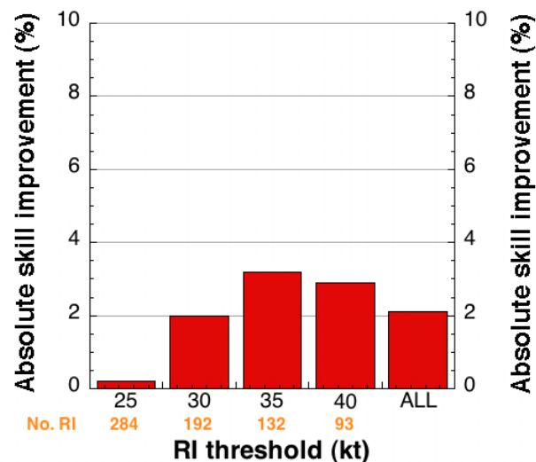
Fig. 5. Improvement of the new eastern North Pacific Experimental RII over the current operational version for the 1995-2009 dependent sample (N=2422). The number of RI cases for each RI threshold is depicted in orange along the x-axis.
