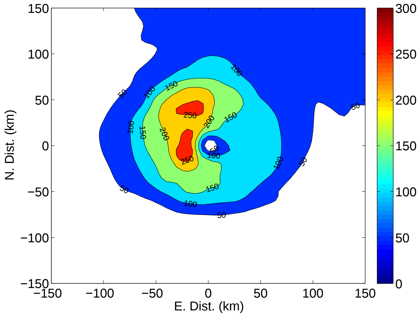
Paloma 20081107I2 F_{\text{sens}} ( \text{W m}^{-2} )
