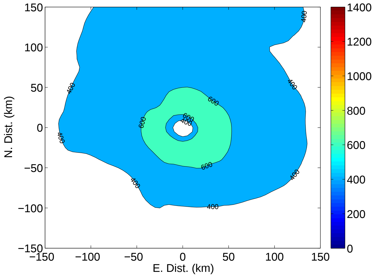
Paloma 20081107I1 F_{\text{lat}} ( \text{W m}^{-2} )
