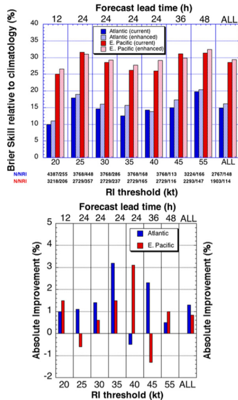
FIG. 4. (top) BSS relative to climatology of the current (solid bars) and enhanced (hatched bars) versions of the SHIPS-RII for the Atlantic (blue) and eastern North Pacific (red) basins at each lead time and RI threshold and for all seven of the RI thresholds combined (ALL) (upper x axis) for the 1995–2012 developmental sample. The total number of cases N and RI cases N_{RI} at each lead time are provided for the Atlantic (blue) and eastern Pacific basins (red) (lower x axis). (bottom) The improvements in skill of the enhanced SHIPS-RII over the current version are also provided.
