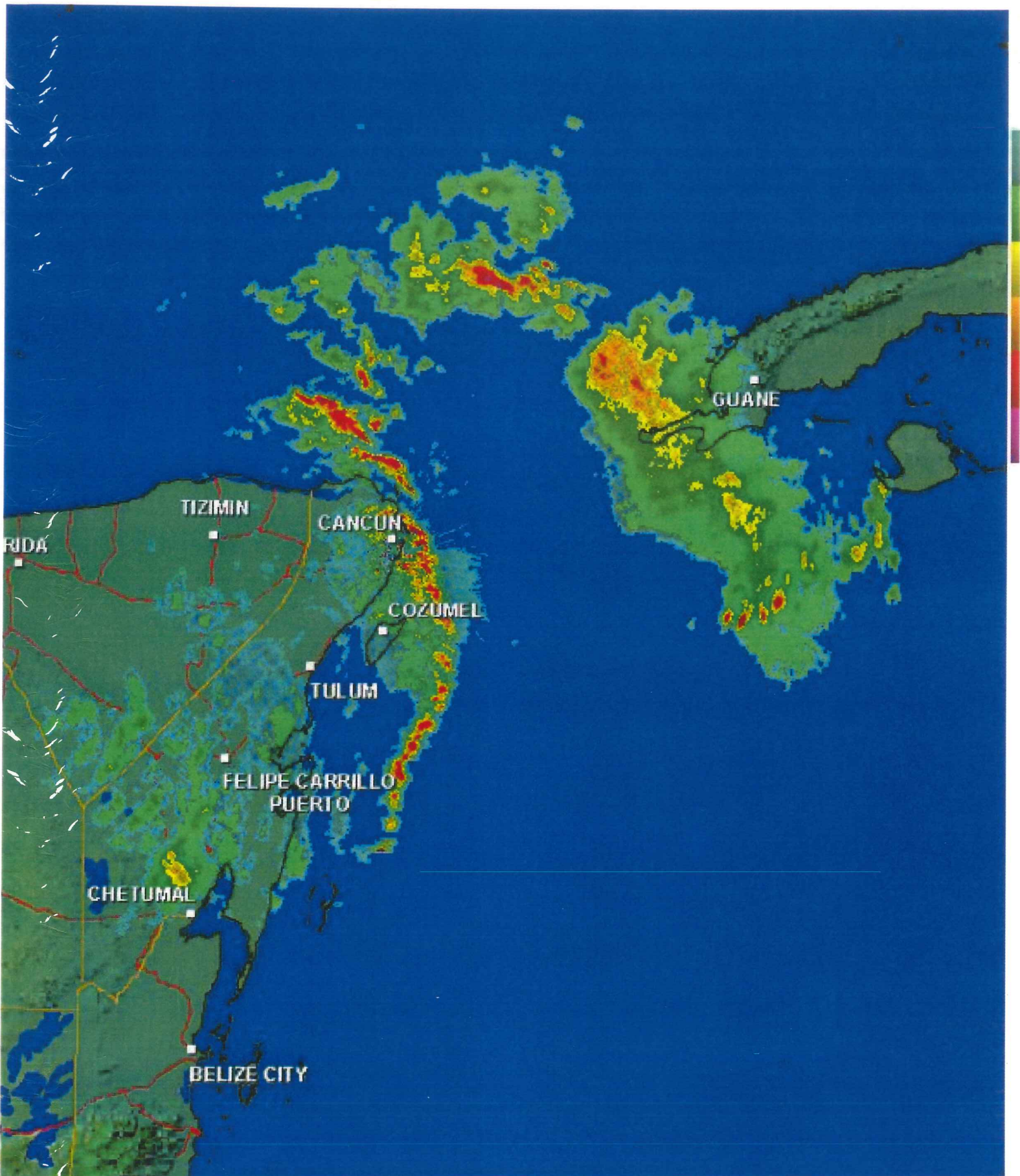
Figure 1. Radar image of the Yucatan Peninsula and surrounding waters.
