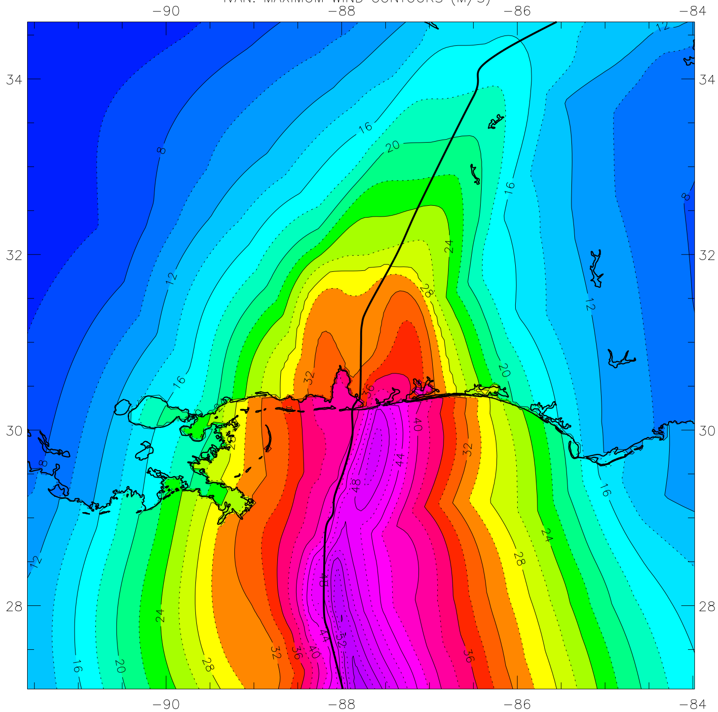
IVAN: MAXIMUM WIND CONTOURS (M/S)
