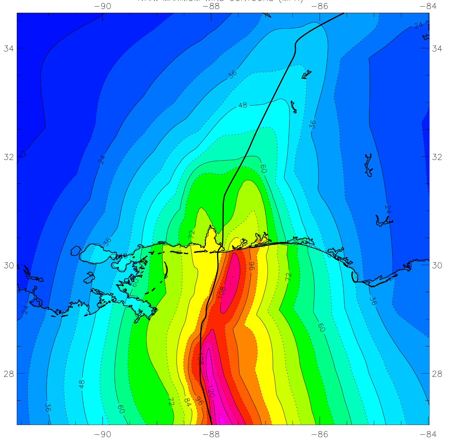
IVAN: MAXIMUM WIND CONTOURS (MPH)
