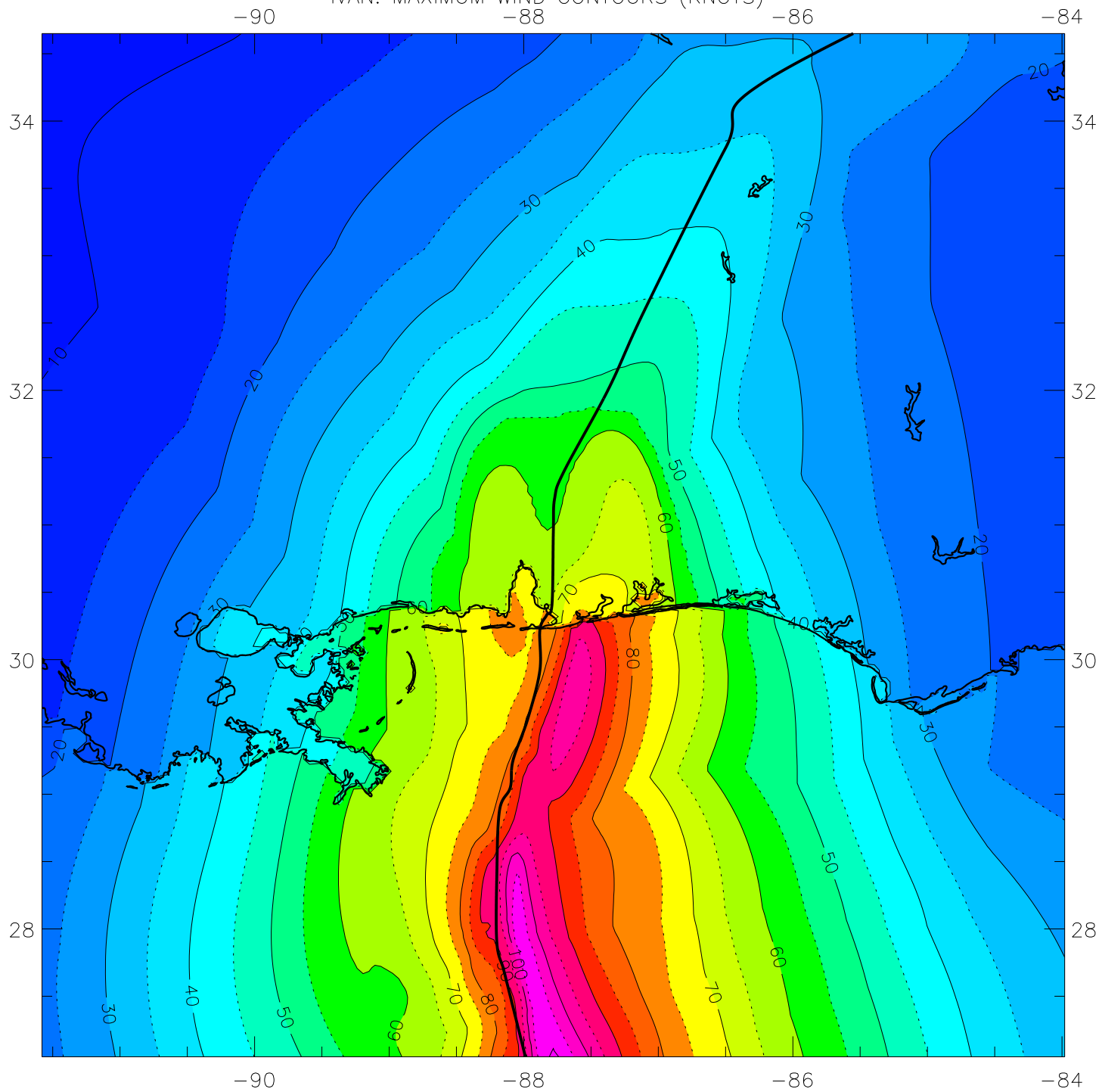
IVAN: MAXIMUM WIND CONTOURS (KNOTS)
