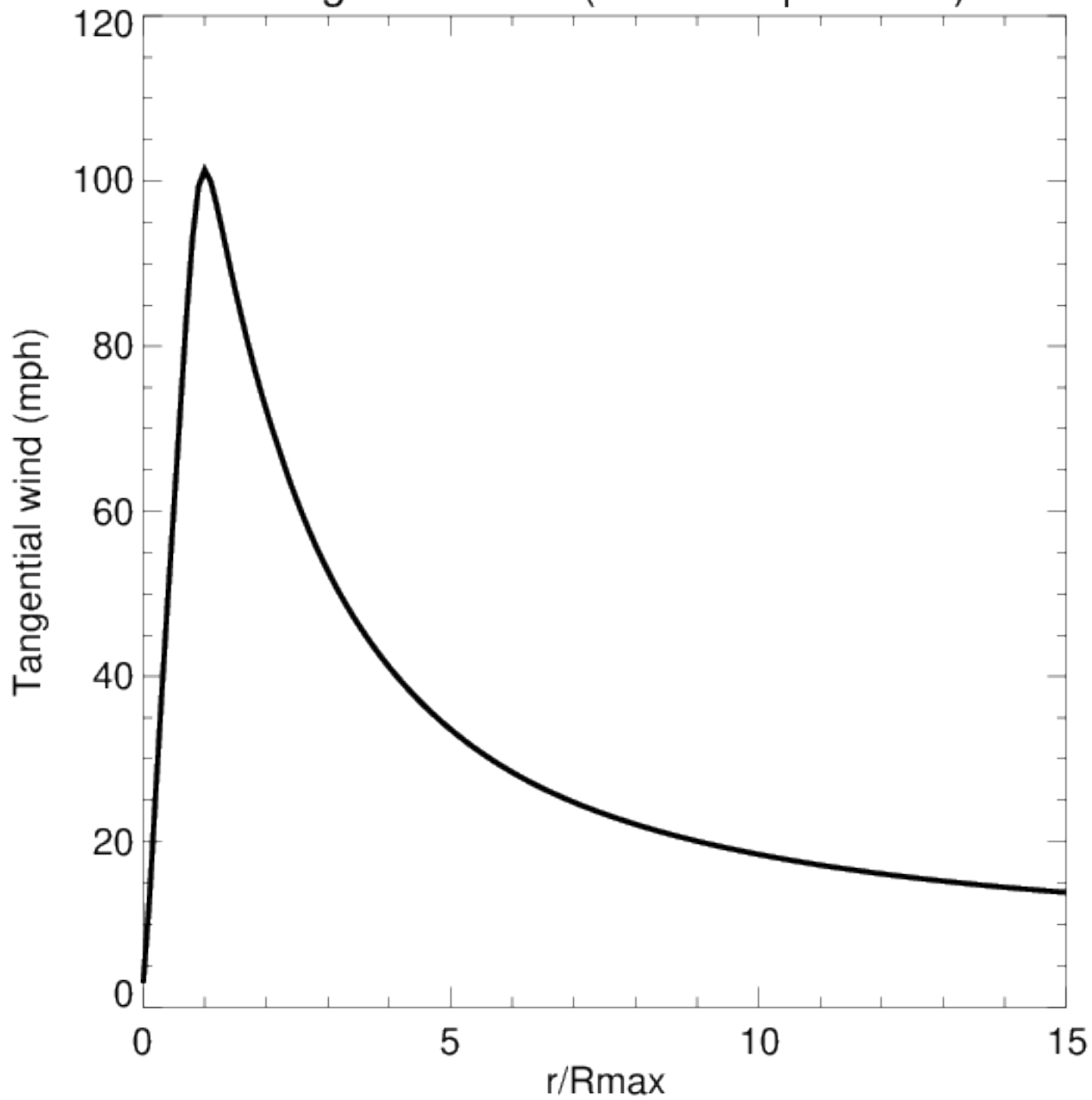
Tangential wind (B=1.40 cp=962.1)
