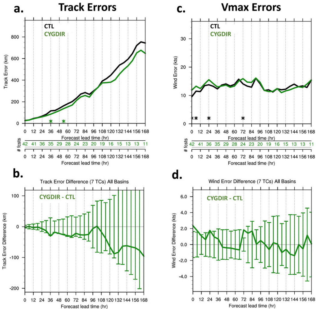
FIG. 5. As in Fig. 4, but for CTL (black lines) and CYGDIR (green lines).
