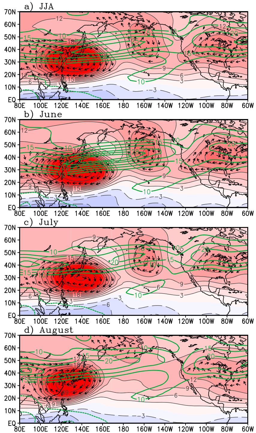
Figure 6. Steady-state linear baroclinic model response depicted by the 200-hPa streamfunction (color, contour interval 3 \times 10^6 \text{ s}^{-1} ) and rotational wind (vector) to the heating profile associated with the East Asian Monsoon shown in Figure 5. The background state is from (a) June-July-August (JJA), (b) June, (c) July, and (d) August. Different background states were chosen in order to illustrate the importance of subseasonality on teleconnection.
