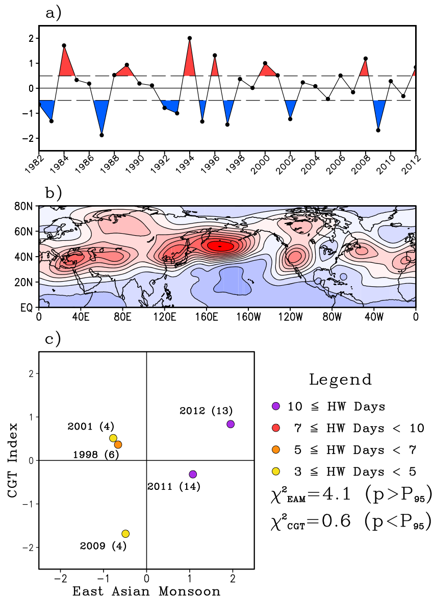
Figure 10. (a) Observed normalized circumboreal teleconnection (CGT) index and (b) the spatial map associated with the CGT index as defined by an empirical orthogonal function analysis of June–July–August 200-hPa geopotential height variability. (c) Scatter diagram of the number of heat wave (HW) days over the Great Plains with respect to the East Asian Monsoon (EAM) index (x axis) and the CGT index (y axis). Heat wave days are color coded as in the legend with their respective year shown as well as the number of days (parenthesis). \chi^2 values given for the composites of heat wave days for positive and negative EAM and CGT indices.
