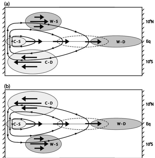
FIG. 15. Sketch of the mechanism by which the positive zonal SST gradient is induced along the equator during the (a) positive and (b) negative phases of the Atlantic dipole oscillation. Thicker arrows indicate wind perturbations associated with the dipole oscillation. Dark shades are used for warm SST anomalies and light shades for cold SST anomalies. Here W-D represents a warm and deep anomaly, W-S is a warm and shallow anomaly, C-D is a cold and deep anomaly, and C-S is a cold and shallow anomaly. Closed circuits represent cross-equatorial gyre circulation that brings the tropical surface water toward the equator. This gyre circulation supplies cold water in the western boundary layer and warm water in the Sverdrup interior during both the positive and negative phases of the dipole oscillation. The warm equatorial SSTA is then shifted to the east and intensified as a result of the Bjerknes feedback, thus producing a stationary Atlantic Niño condition.
