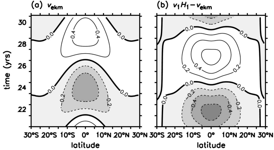
FIG. 3. Case 1: latitude–time structure of the zonally averaged meridional (a) Ekman transport and (b) non-Ekman transport components ( \text{m}^2 \text{s}^{-1} ). Ekman transport is not defined at the equator; thus it is interpolated at the equator.
