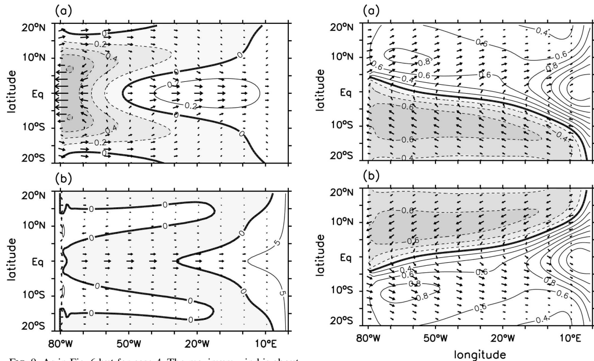
FIG. 9. As in Fig. 6 but for case 4. The maximum wind is about 0.3 \text{ m s}^{-1} , and the maximum zonal mixed layer transport is about 2.5 \text{ m}^2 \text{ s}^{-1} .
