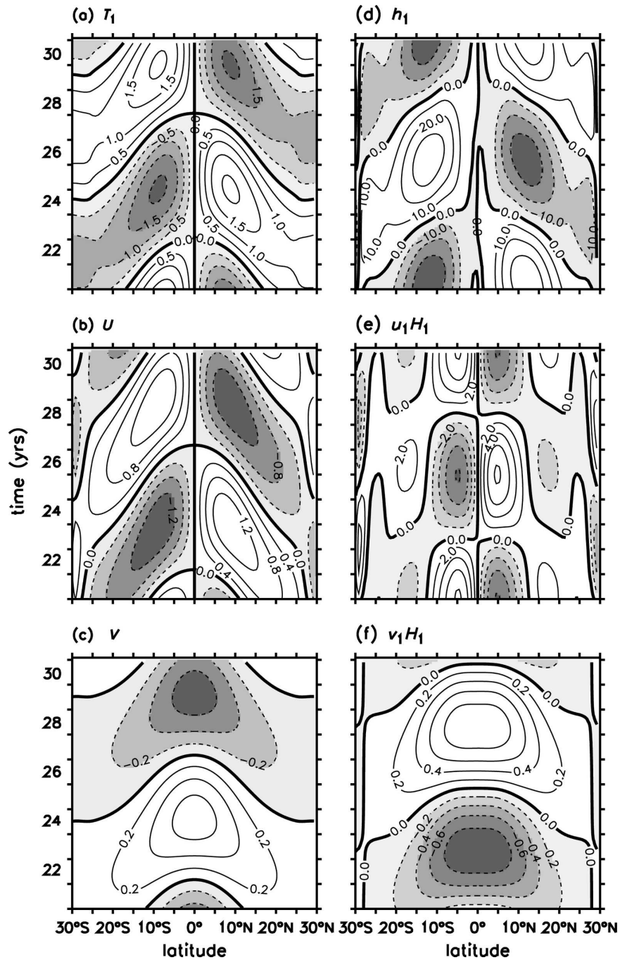
FIG. 1. Case 1: latitude–time structure of the zonally averaged (a) SST ( ^{\circ}\text{C} ), (b) zonal and (c) meridional winds ( \text{m s}^{-1} ), (d) mixed layer depth (m), and (e) zonal and (f) meridional mixed layer transport ( \text{m}^2 \text{s}^{-1} ) anomalies.
