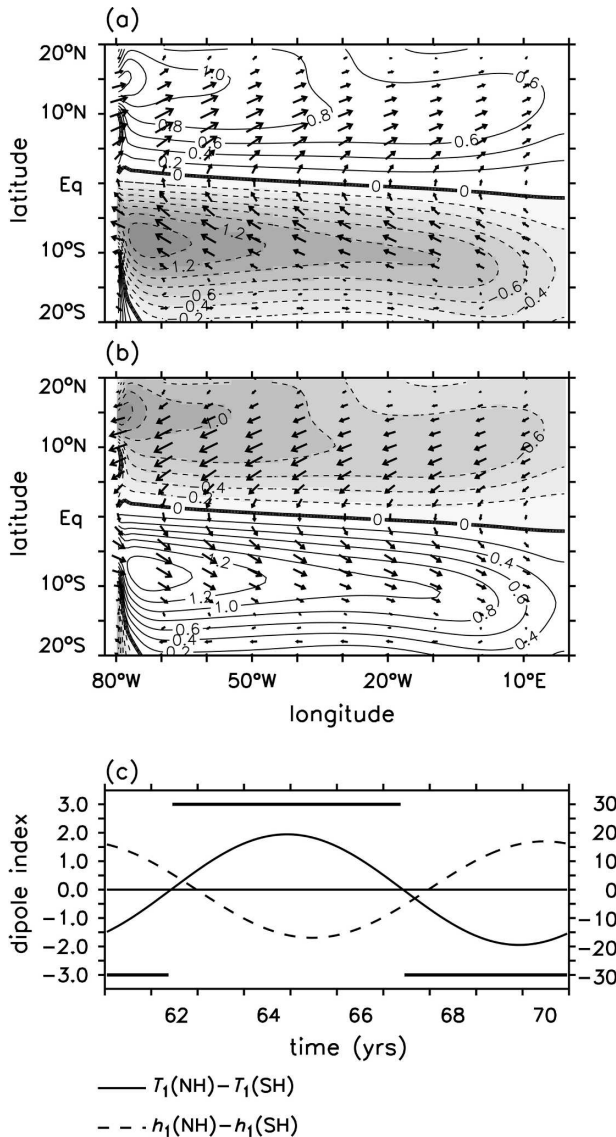
FIG. 13. As in Fig. 8 but for case 6. The maximum wind is about 1.2 \text{ m s}^{-1} .
