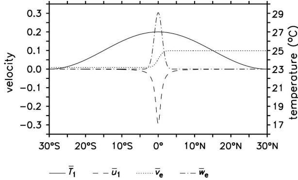
FIG. 12. The mixed layer temperature ( ^{\circ}\text{C} ), zonal mixed layer velocity ( \text{m s}^{-1} ), meridional mixed layer velocity ( 10 \text{ m s}^{-1} ), and entrainment rate ( 10^5 \text{ m s}^{-1} ) of the mean state used for cases 6 and 7. See text for how these values are derived.
