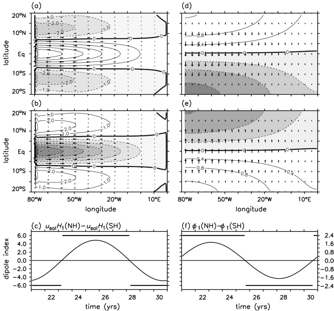
FIG. 4. Case 1: (left) the streamfunction ( \psi_1 ) and solenoidal flow ( u_{sol}H_1 and v_{sol}H_1 ) anomalies for the mixed layer averaged for the (a) positive and (b) negative phase. (c) The dipole index used for the phase averaging is the area-averaged zonal solenoidal transport ( u_{sol}H_1 ) of the Northern Hemisphere minus that of the Southern Hemisphere. (right) The transport potential ( \phi_1 ) and potential flow ( u_{pot}H_1 and v_{pot}H_1 ) anomalies for the mixed layer averaged for the (d) positive and (e) negative phase. (f) The dipole index used in this case is the area-averaged transport potential anomaly of the Northern Hemisphere minus that of the Southern Hemisphere. The unit is 10^{-6} meters cubed per second for the streamfunction and transport potential and meters squared per second for the solenoidal flow and potential flow components. The maximum transport value is about 9.4 \text{ m}^2 \text{ s}^{-1} for the solenoidal flow component and about 0.9 \text{ m}^2 \text{ s}^{-1} for the potential flow component.
