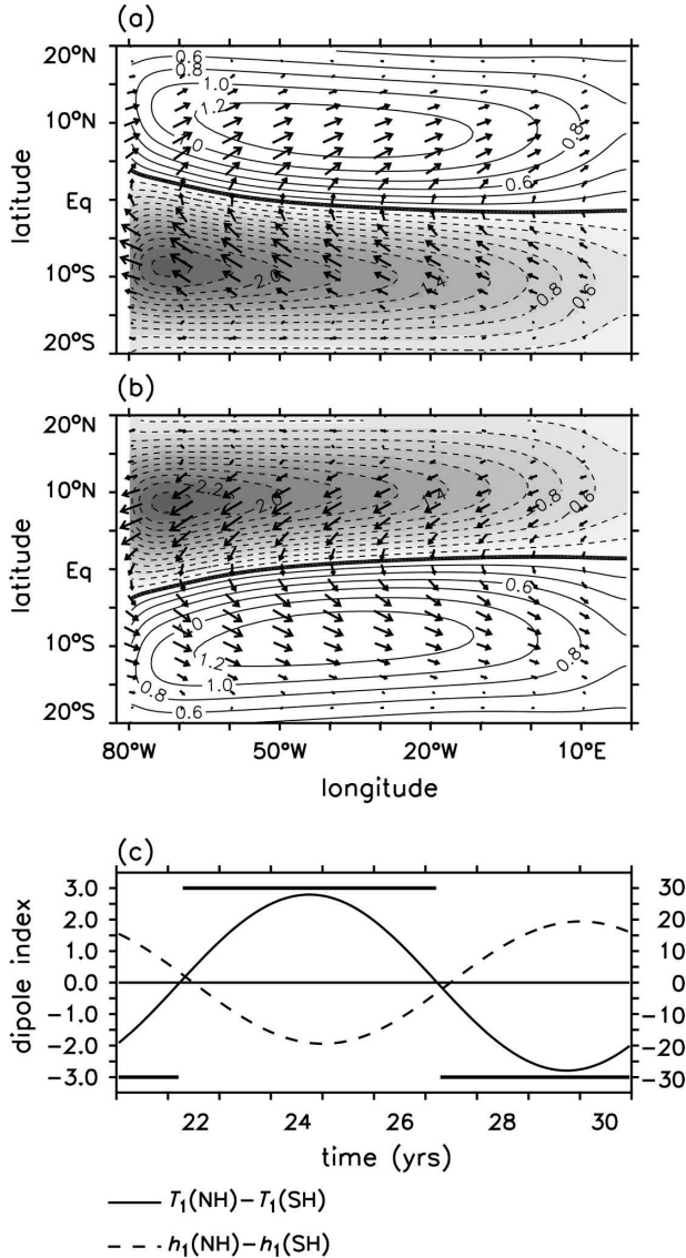
FIG. 8. As in the left column of Fig. 2 but for case 4. The broken line in (c) is the area-averaged mixed layer depth of the Northern Hemisphere minus that of the Southern Hemisphere. The maximum wind is about 1.4 \text{ m s}^{-1} .
