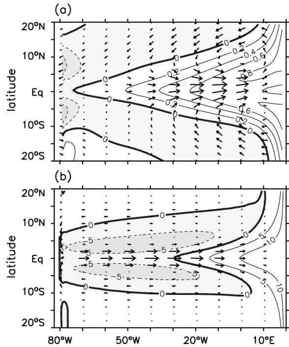
FIG. 14. As in Fig. 9 but for case 7. The maximum wind is about 0.4 \text{ m s}^{-1} , and the maximum zonal mixed layer transport is about 5.3 \text{ m}^2 \text{ s}^{-1} .
