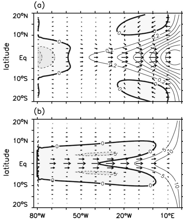
FIG. 11. As in Fig. 9 but for case 5. The maximum wind is about 0.4 \text{ m s}^{-1} , and the maximum zonal mixed layer transport is about 5.2 \text{ m}^2 \text{ s}^{-1} .
