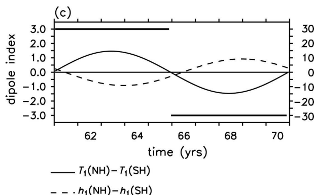
FIG. 10. As in Fig. 8 but for case 5. The maximum wind is about 0.8 \text{ m s}^{-1} .
