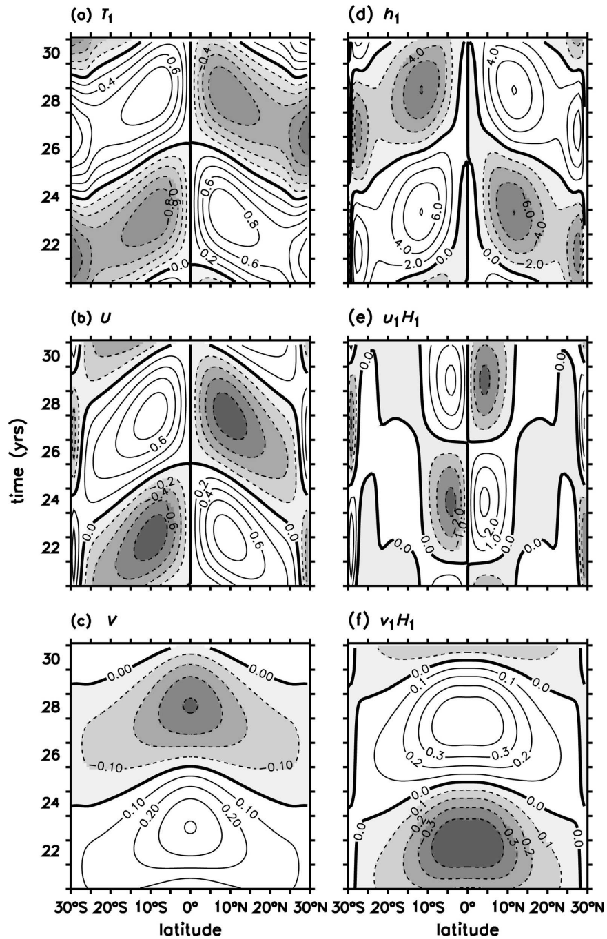
FIG. 7. As in Fig. 1 but for case 3. Note that the contour intervals are different from those used in Fig. 1.
