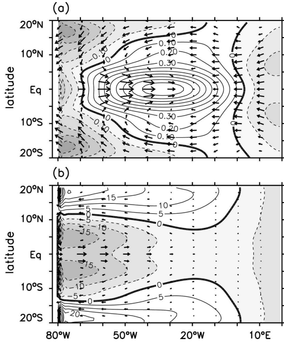
FIG. 6. Case 2: the two-dimensional structures of (a) SST and wind anomalies and (b) the mixed layer depth and transport anomalies, all averaged for one full cycle of the dipole oscillation between model year 21 and 30. The maximum wind is about 0.4 \text{ m s}^{-1} , and the maximum zonal mixed layer transport is about 3.2 \text{ m}^2 \text{ s}^{-1} .
