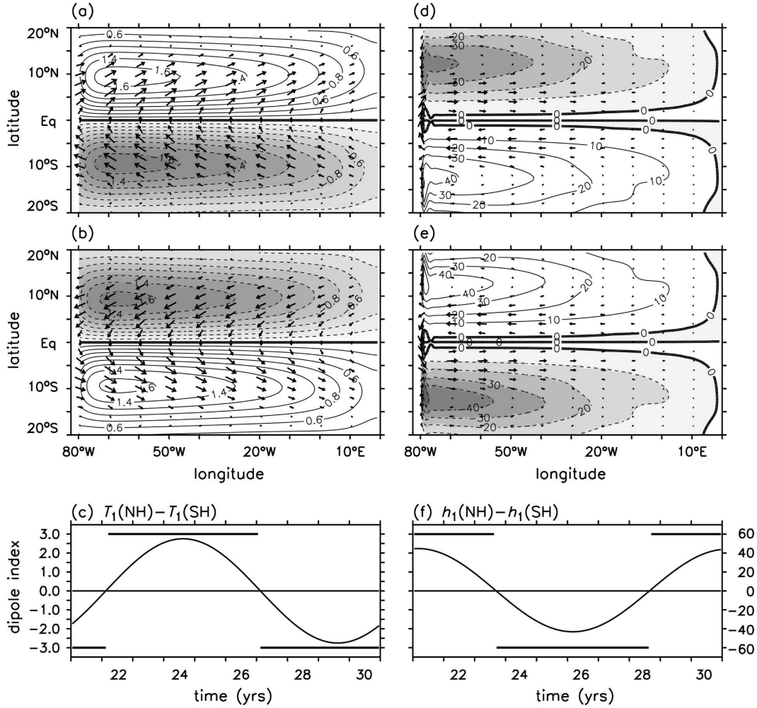
FIG. 2. Case 1: (left) two-dimensional structure of SST and wind anomalies averaged for (a) the positive phase and (b) the negative phase. (c) The dipole index used for the phase averaging is the area-averaged SST of the Northern Hemisphere minus that of the Southern Hemisphere. (right) The mixed layer depth and transport anomalies averaged for (d) the negative phase and (e) the positive phase. (f) The dipole index used in this case is the area-averaged mixed layer depth of the Northern Hemisphere minus that of the Southern Hemisphere. The maximum wind is about 1.3 \text{ m s}^{-1} , and the maximum zonal mixed layer transport is about 9.5 \text{ m}^2 \text{ s}^{-1} .
