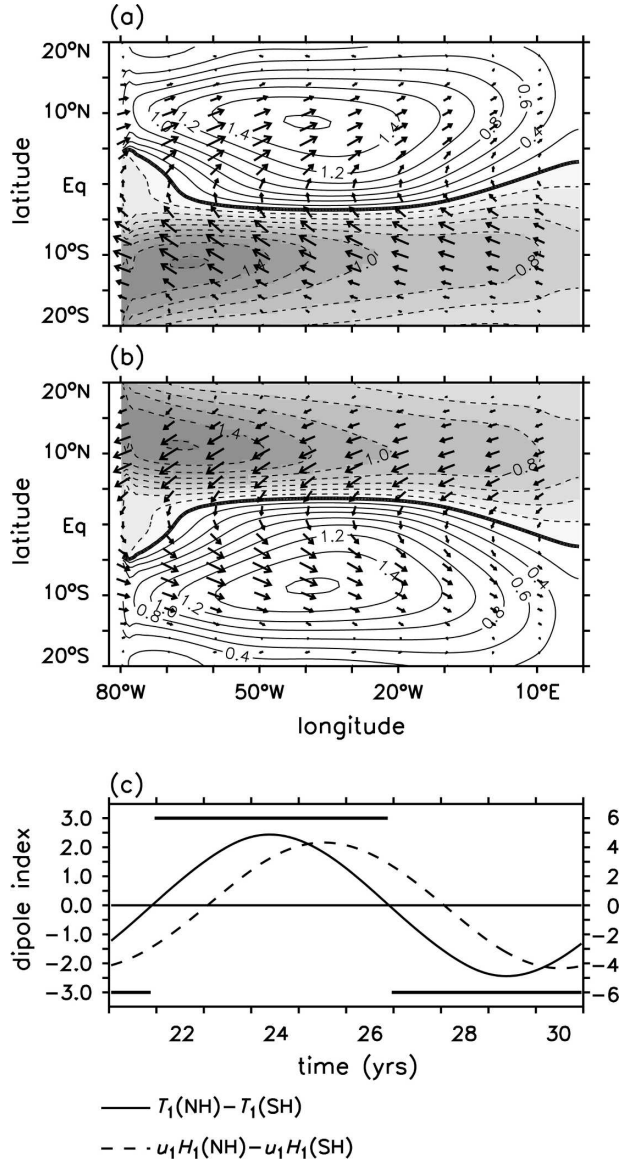
FIG. 5. Case 2: two-dimensional structure of SST and wind anomalies averaged for the (a) positive and (b) negative phase. (c) The dipole index used for the phase averaging is the area-averaged SST of the Northern Hemisphere minus that of the Southern Hemisphere. The broken line in (c) is the area-averaged zonal transport of the Northern Hemisphere minus that of the Southern Hemisphere, and this index is used for cross-equatorial gyre circulation: a negative value indicates a cyclonic circulation and a positive value indicates a clockwise circulation. The maximum wind is about 1.3 \text{ m s}^{-1} .
